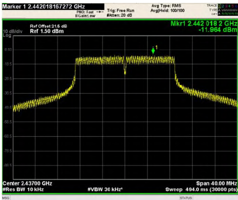
802.11n-HT20 Middle Channel
