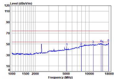
11ax_20M_TX_CH_01_Vertical
