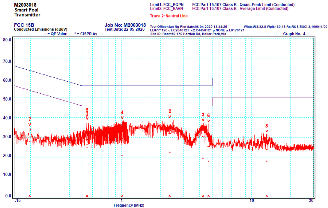
Graph 3-4: Neutral Line (0.15 MHz to 30 MHz)
