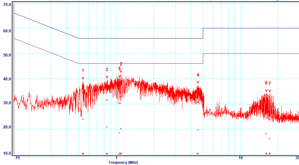
Graph 3-3: Active Line (0.15 MHz to 30 MHz)
