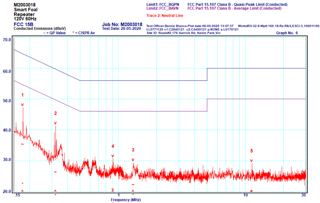
Graph 3-6: Neutral Line (0.15 MHz to 30 MHz)
