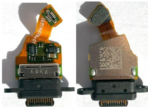
Figure 6: BRC3610 USB FPC top (left) and bottom (right)
