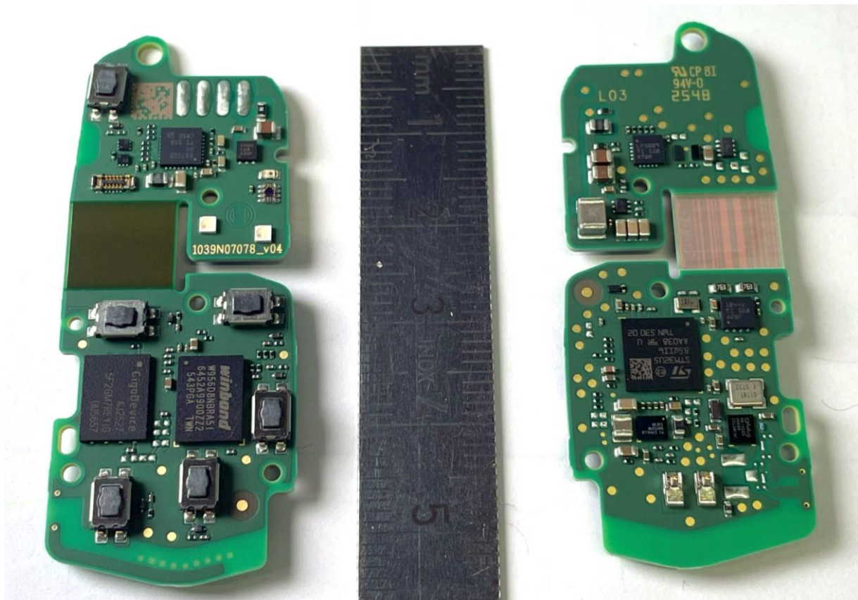
Figure 7: BRC3610 PCB top (left) and bottom (right)
