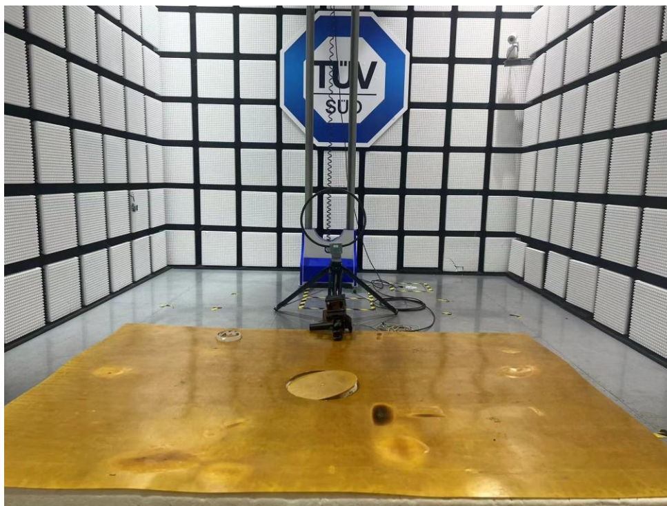
Spurious Emission Below 30MHz
