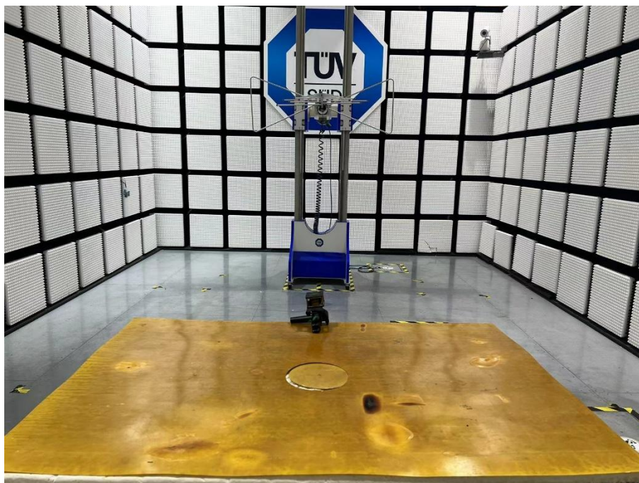
Spurious Emission Below 1GHz
