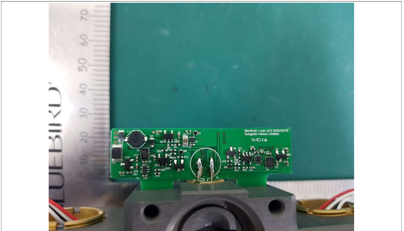
Sub Board_Rear
