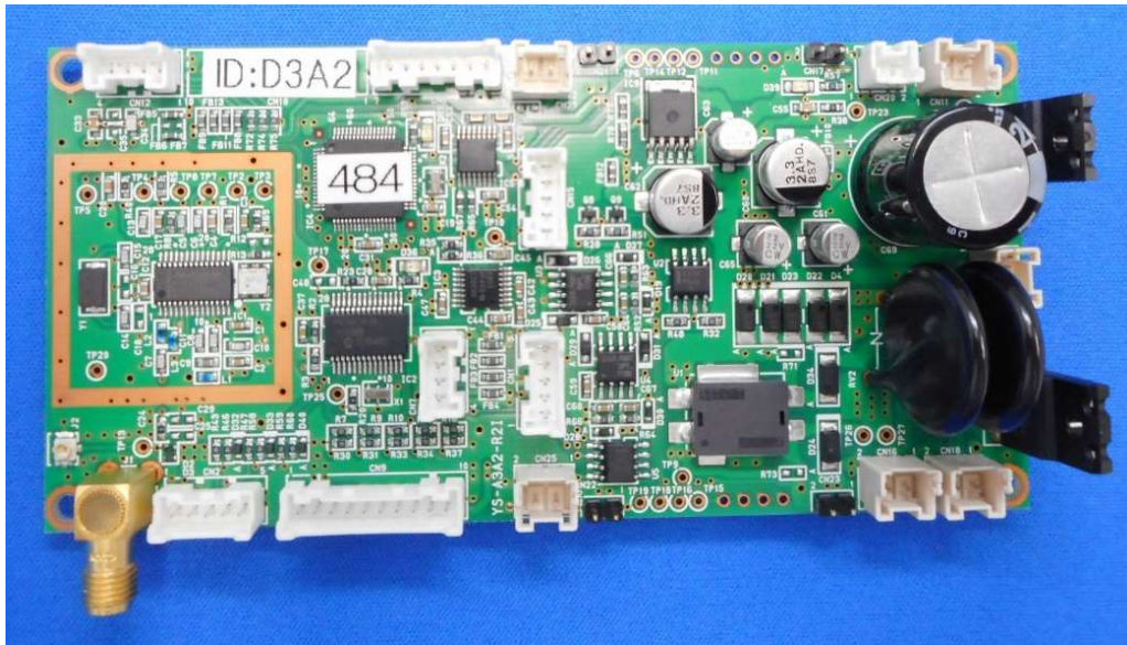
MAIN BOARD FRONT
