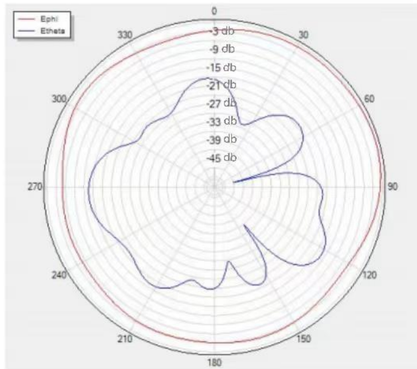
Theta=90 freq=2450MHz
