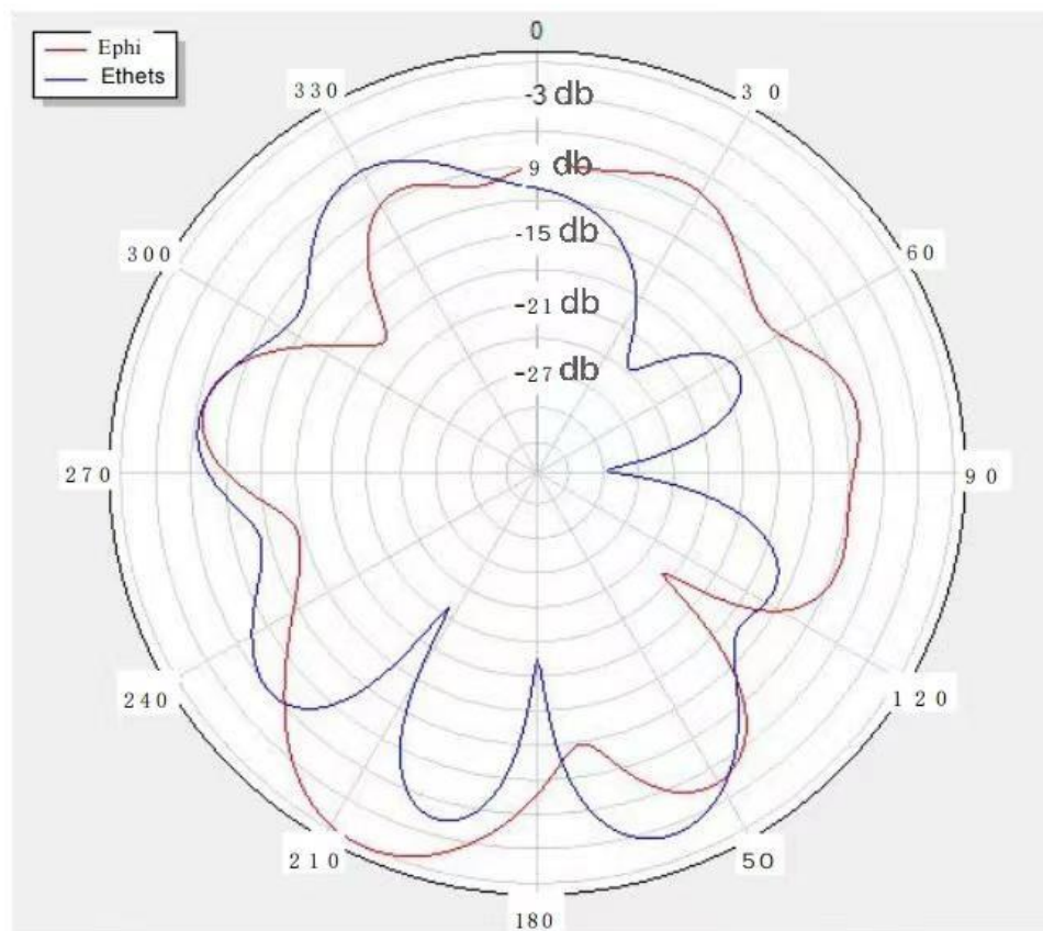
Phi=90 freq=2490MHz
