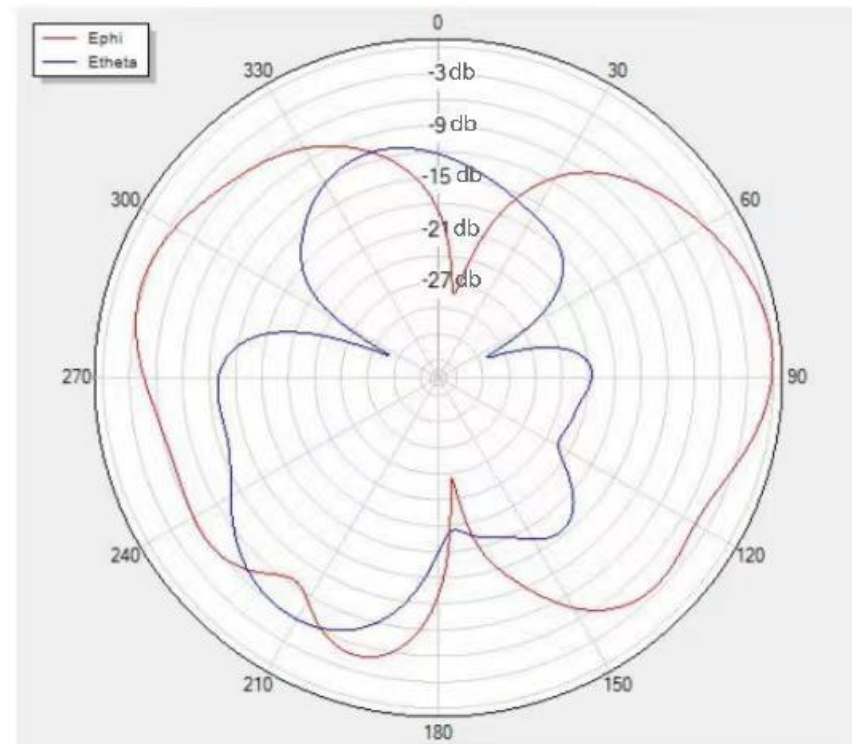
Phi=90 freq=2500MHz
