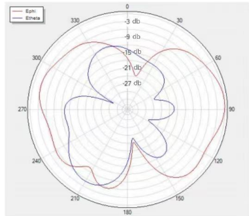
Phi=90 freq=2450MHz
