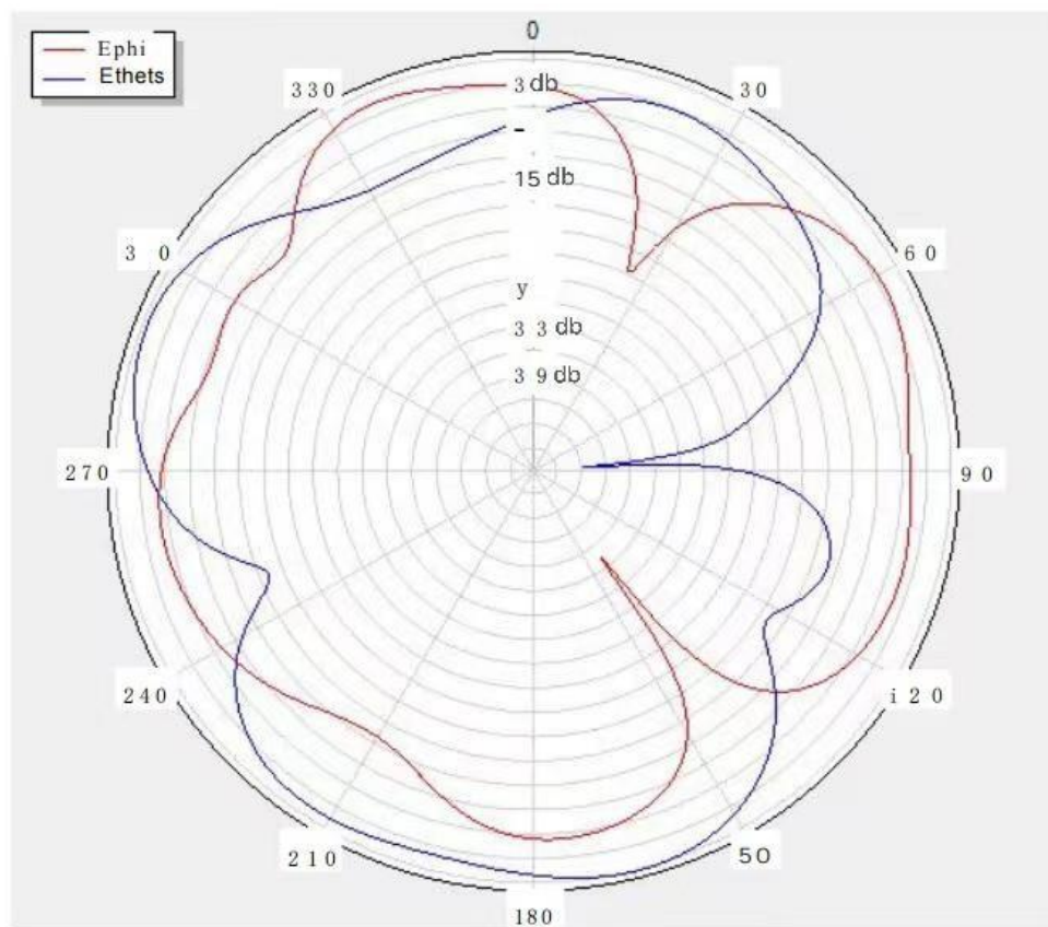
Theta=90 freq=2490MHz
