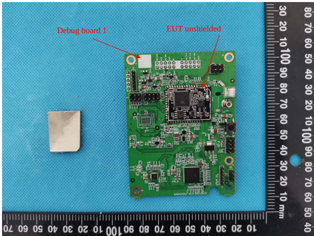
EUT unshielded View
