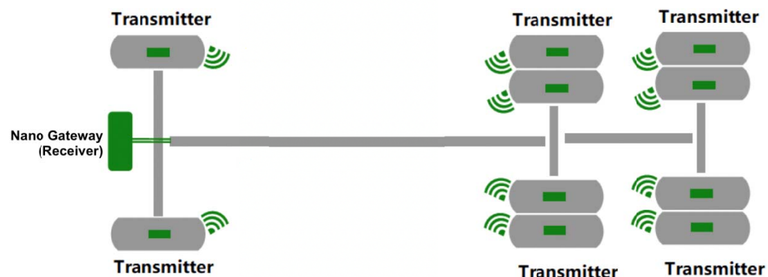
Fig. 1 Architecture diagram
