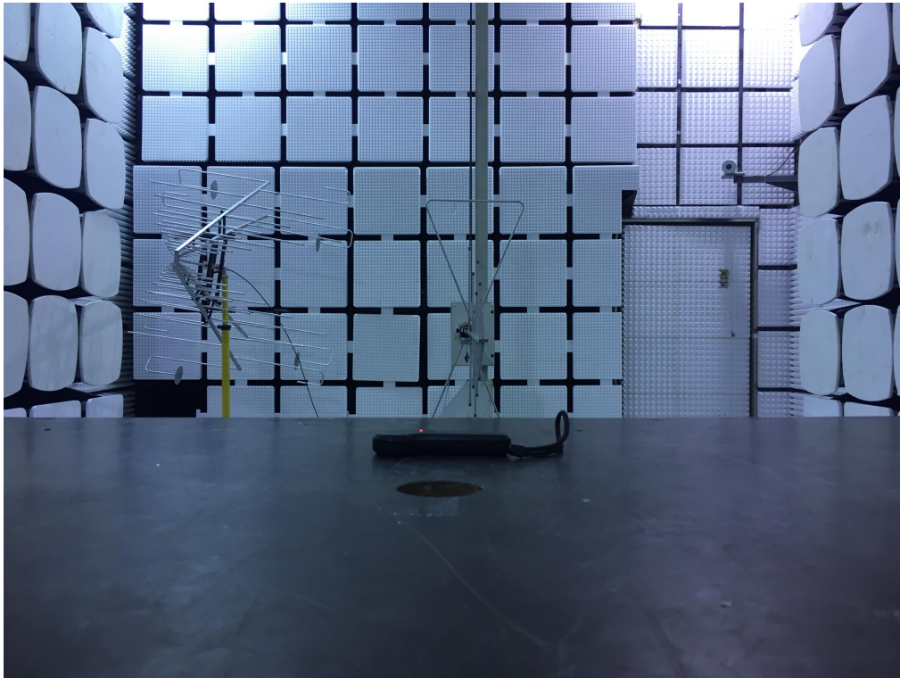
Photo of Radiated Measurement (Below 1G)
