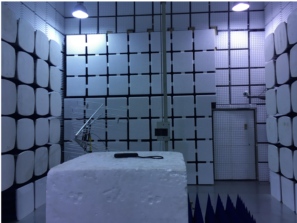
Photo of Radiated Measurement (Above 1G)
