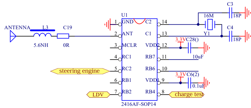
PAN2416AF-SOP14
