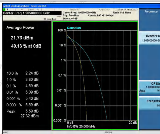
Band25-20MHz-16QAM-26140-1RB#0
