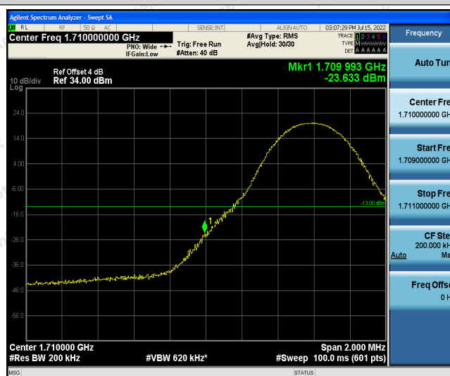
Band4-10MHz-QPSK-20000-1RB#49
