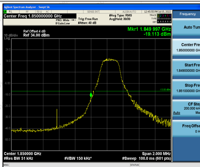
Band2-3MHz-16QAM-18615-1RB#14
