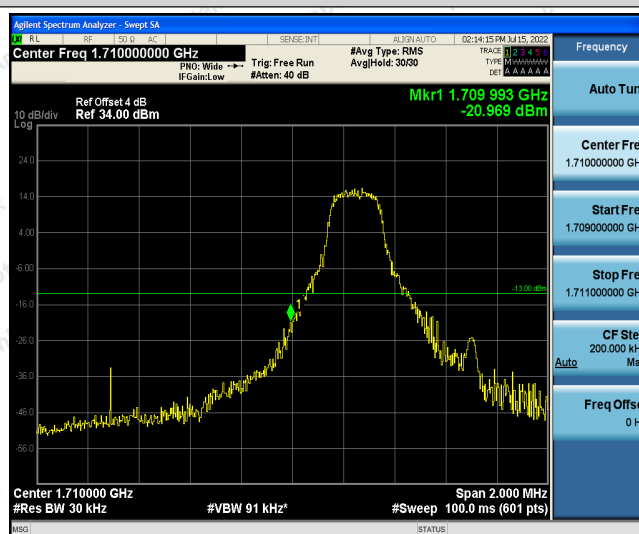
Band4-1.4MHz-QPSK-19957-1RB#5
