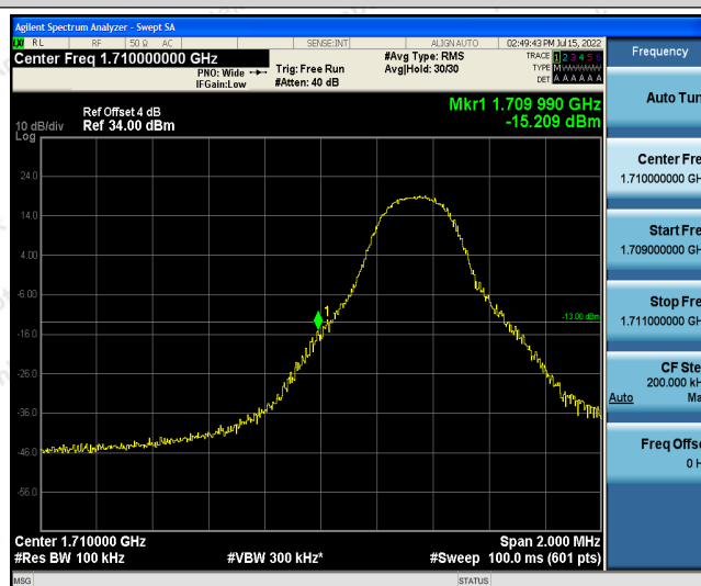
Band4-5MHz-QPSK-19975-1RB#24
