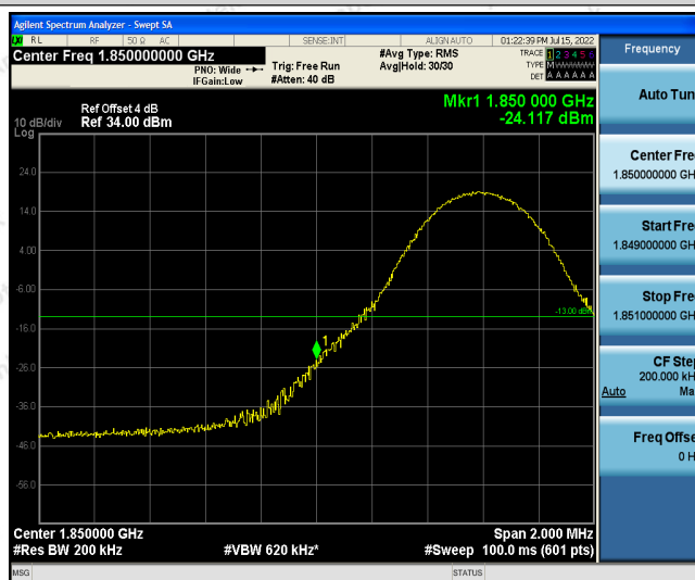
Band2-10MHz-16QAM-18650-1RB#49
