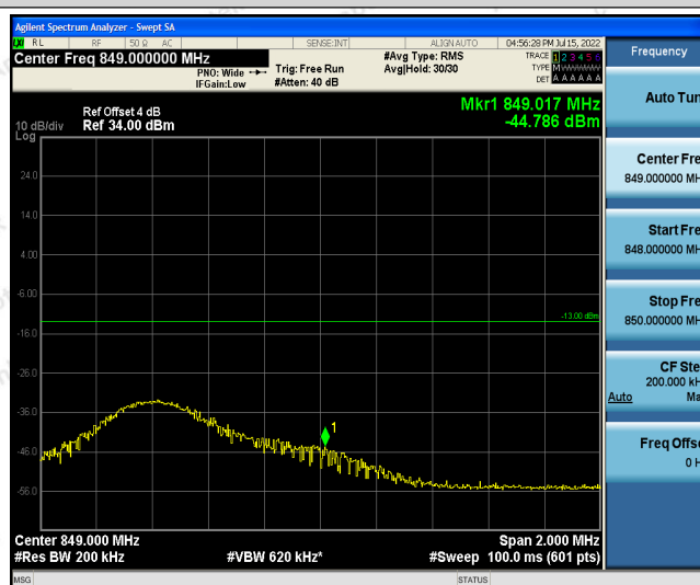
Band5-10MHz-16QAM-20600-1RB#49
