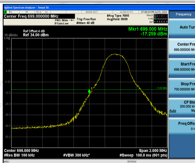
Band12-5MHz-16QAM-23035-1RB#24
