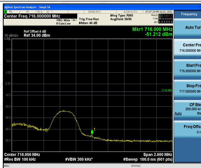
Band12-5MHz-QPSK-23155-1RB#24
