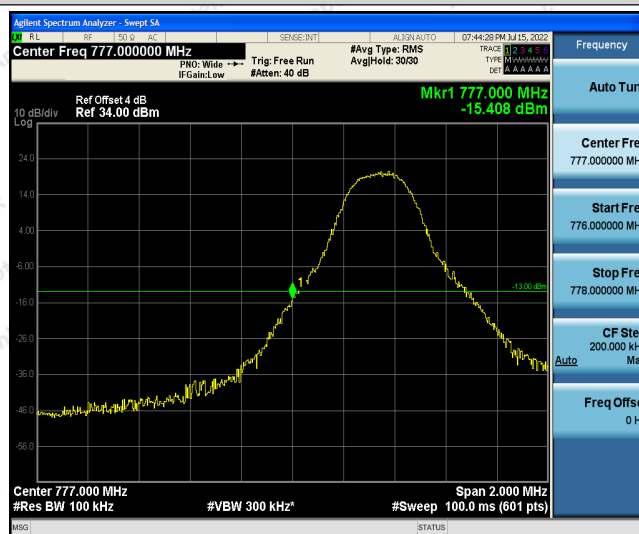
Band13-5MHz-16QAM-23205-1RB#24
