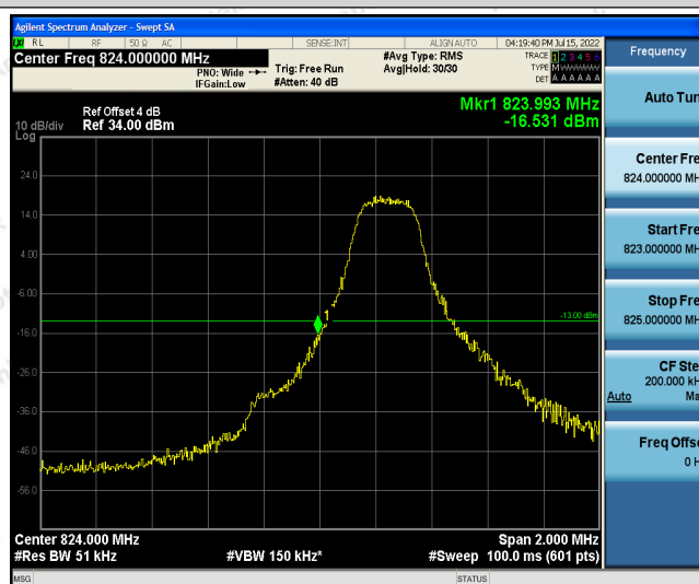
Band5-3MHz-16QAM-20415-1RB#14
