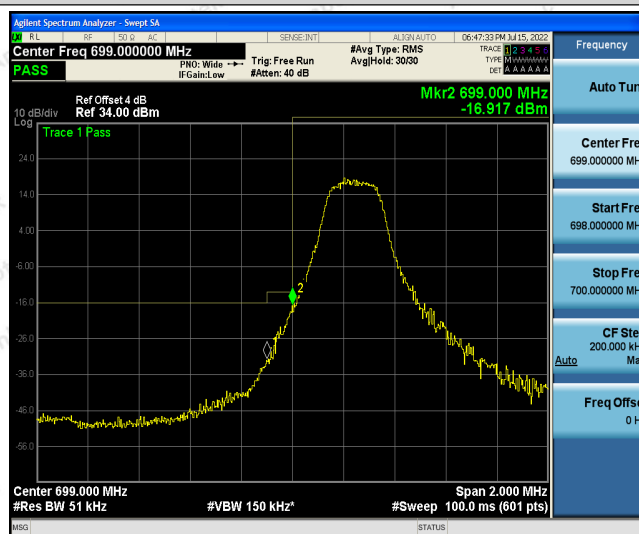
Band12-3MHz-16QAM-23025-1RB#14
