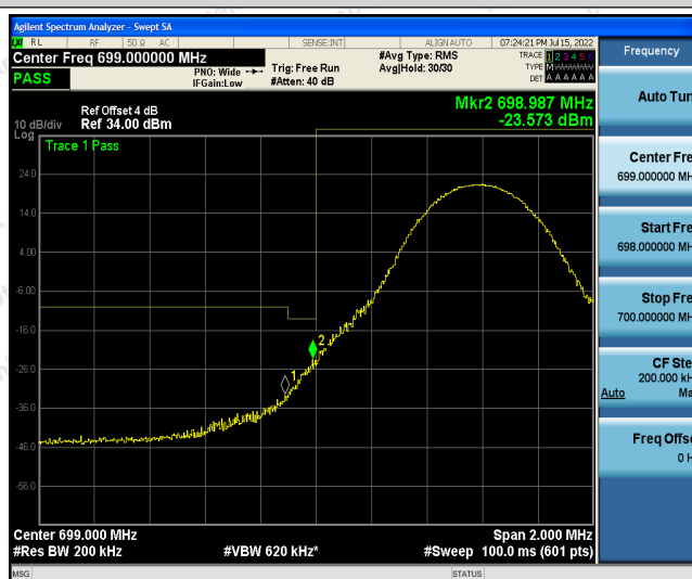
Band12-10MHz-QPSK-23060-1RB#49
