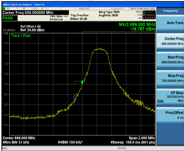
Band12-3MHz-QPSK-23025-1RB#14
