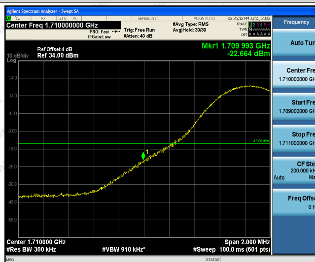
Band4-15MHz-16QAM-20025-1RB#74
