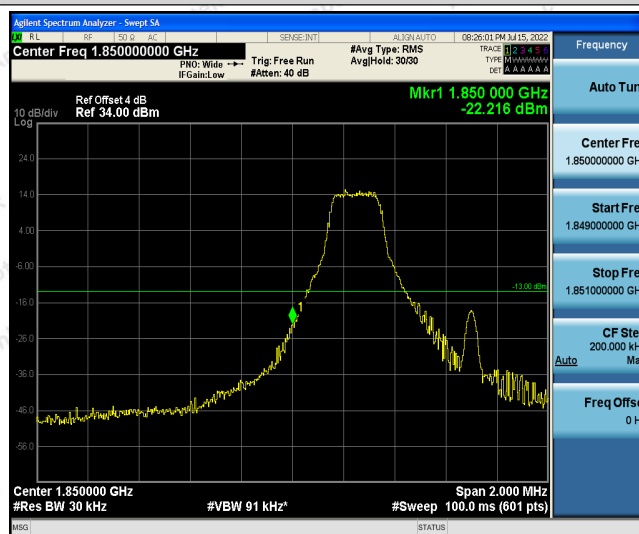
Band25-1.4MHz-16QAM-26047-1RB#5
