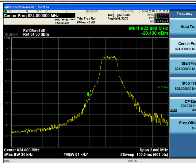
Band5-1.4MHz-16QAM-20407-1RB#5
