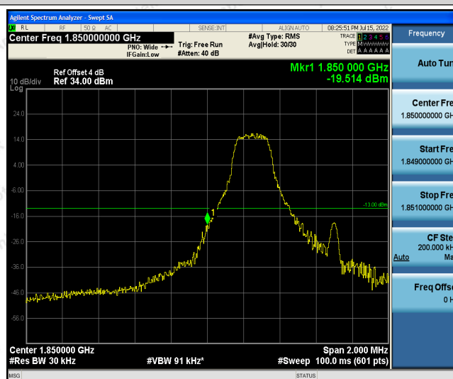
Band25-1.4MHz-QPSK-26047-1RB#5
