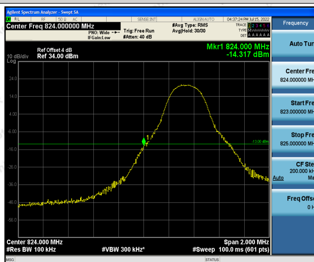
Band5-5MHz-QPSK-20425-1RB#24
