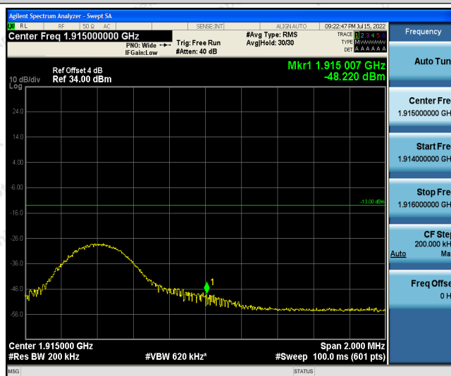
Band25-10MHz-16QAM-26640-1RB#49
