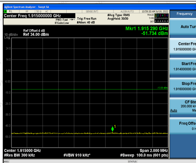
Band25-15MHz-16QAM-26615-1RB#74
