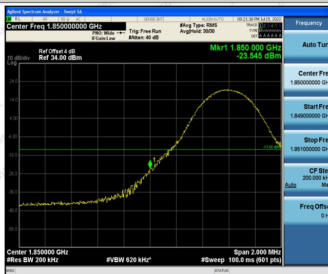
Band25-10MHz-16QAM-26090-1RB#49
