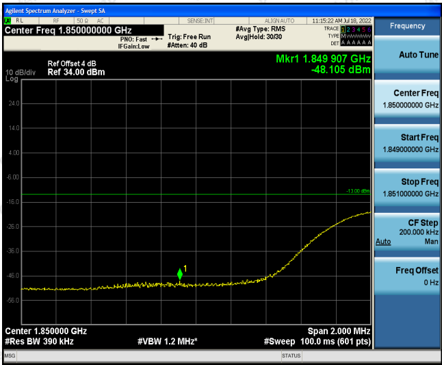
Band25-20MHz-QPSK-26140-100RB#0
