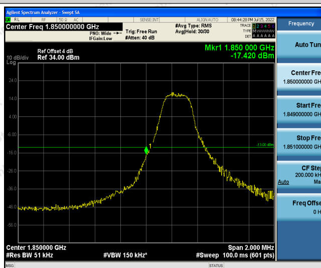
Band25-3MHz-16QAM-26055-1RB#14
