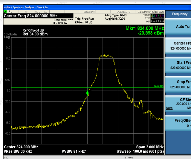
Band26-1.4MHz-QPSK-26797-1RB#5
