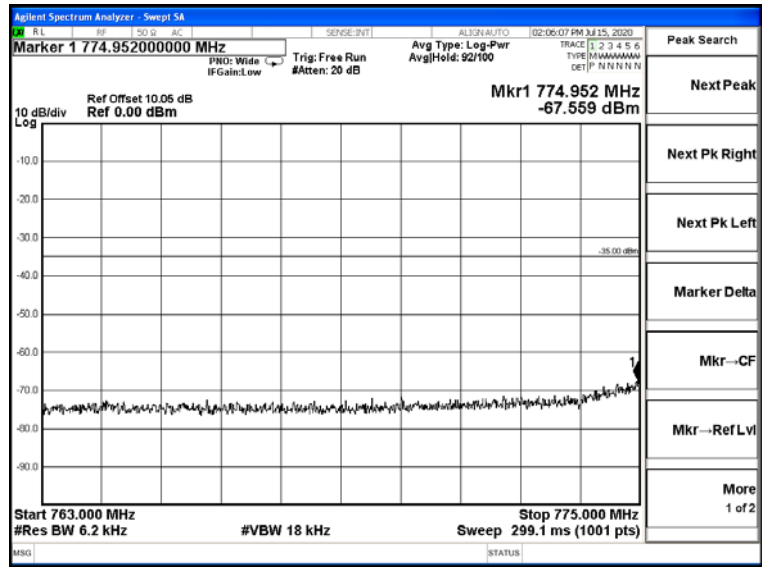
Band Edge Test Graph(s) (Channel Bandwidth: 5 MHz)_LCH_16QAM
