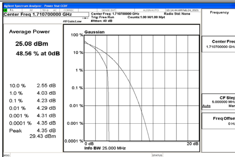
Band66-1.4MHz-QPSK-131979-6RB#0
