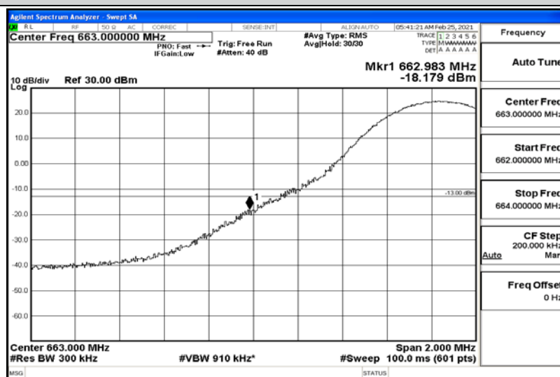
Band71-15MHz-16QAM-133197-75RB#0
