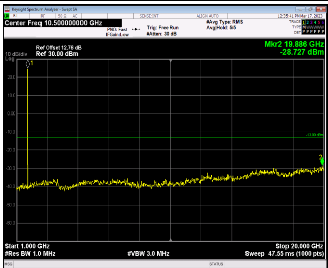
Band66-1.4MHz-QPSK-132322-1RB#0-Range2:1000 ~20000MHz
