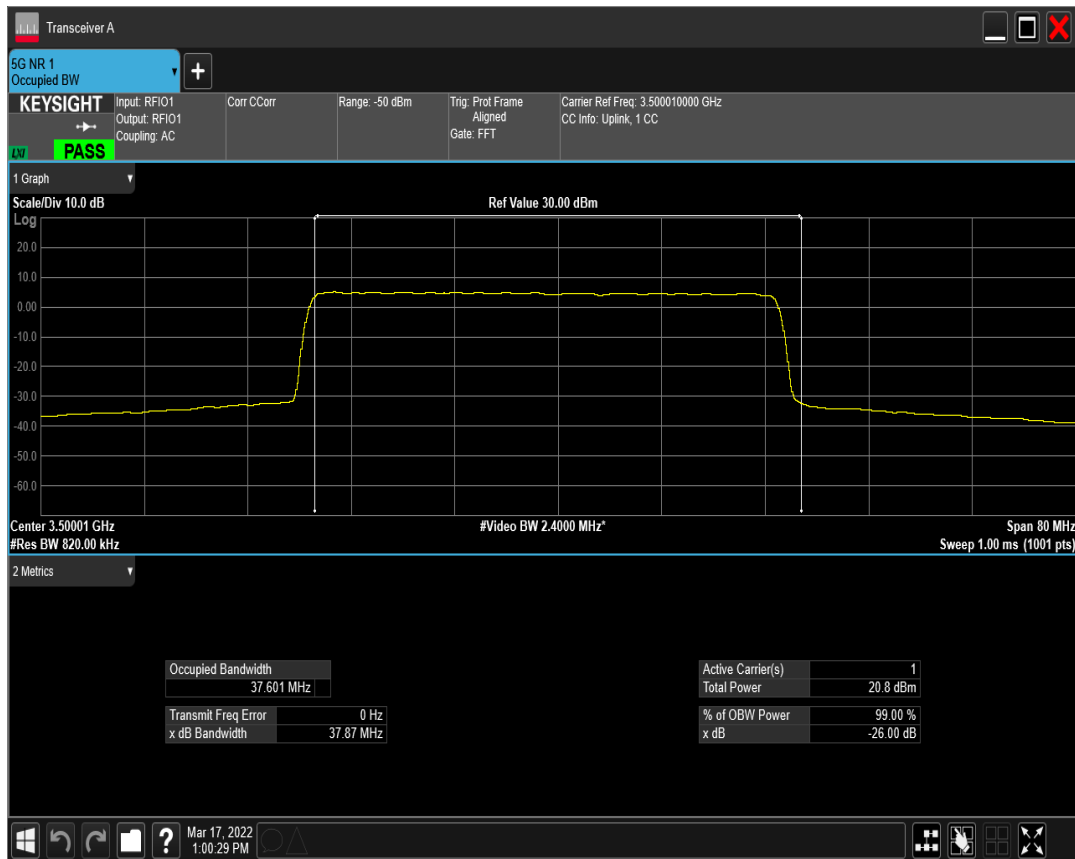
n77(3450-3550) SCS=30kHz CP_QPSK BW=40MHz Channel=633334 RB=106@0
