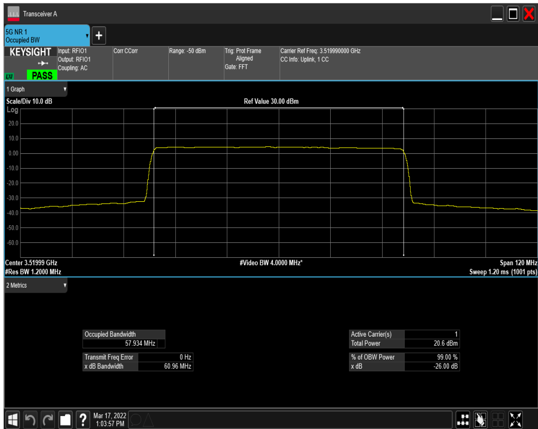
n77(3450-3550) SCS=30kHz CP_QPSK BW=60MHz Channel=634666 RB=162@0
