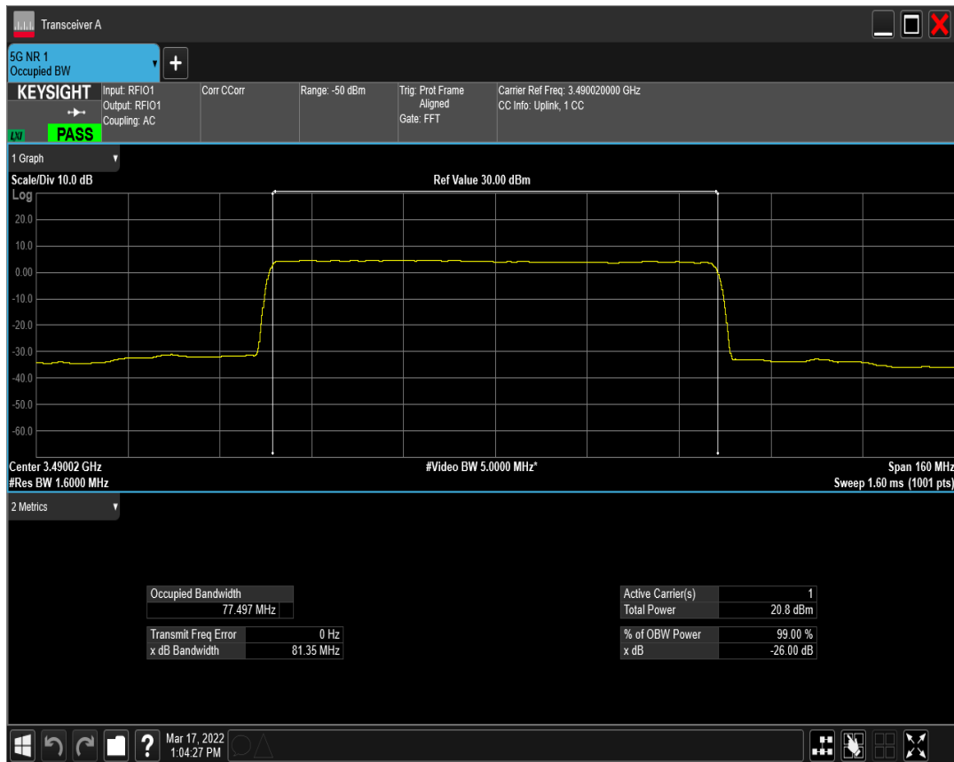
n77(3450-3550) SCS=30kHz CP_QPSK BW=80MHz Channel=632668 RB=217@0
