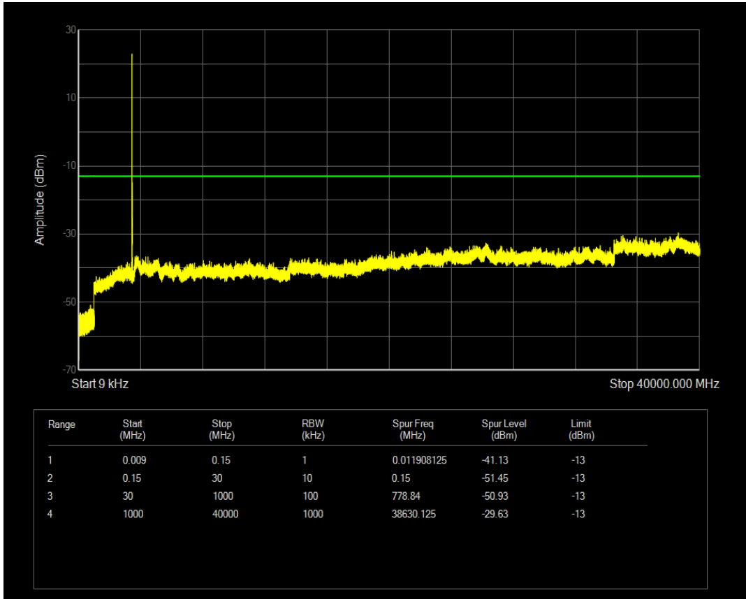
n77(3450-3550) SCS=30kHz DFT_QPSK BW=10MHz Channel=630334 RB=1@23
