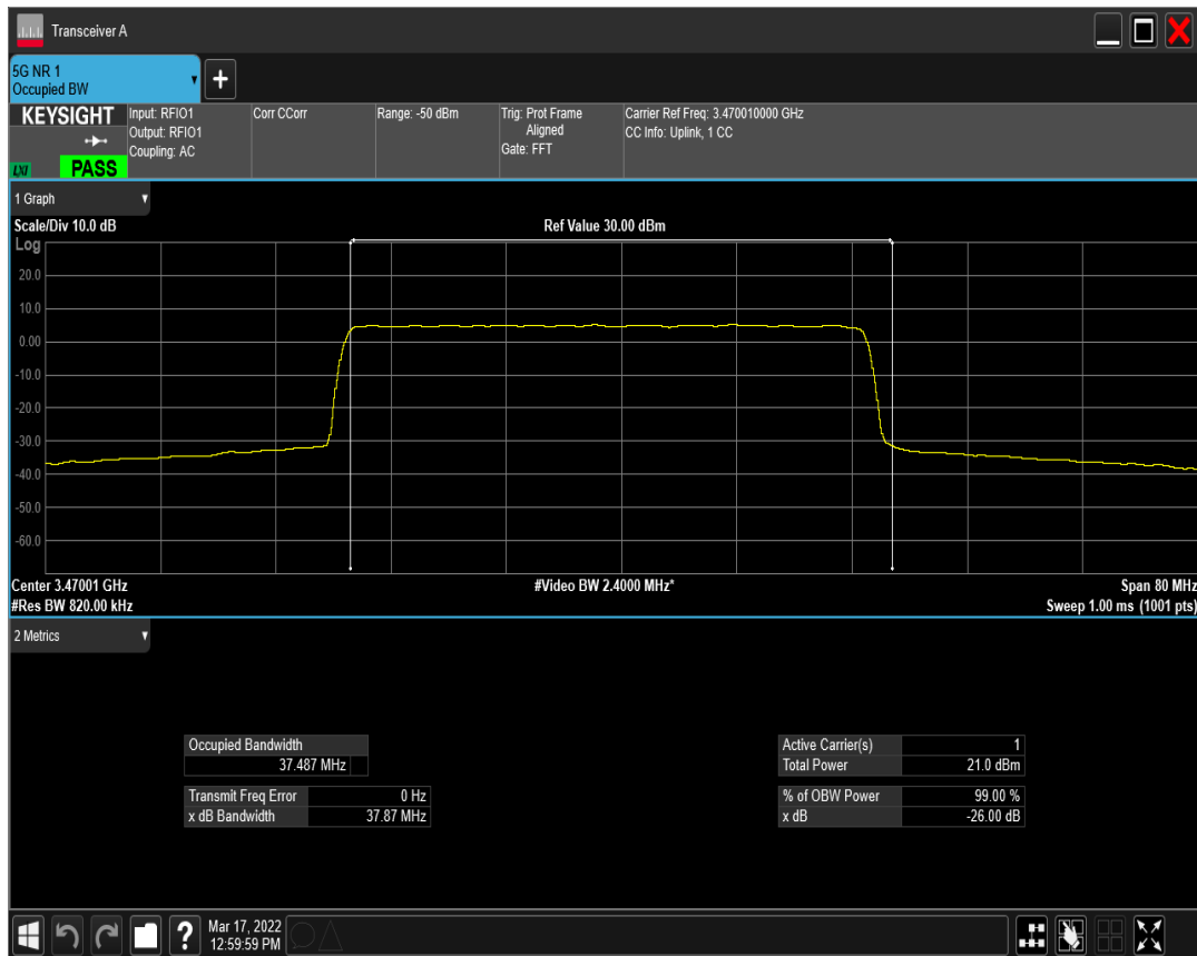
n77(3450-3550) SCS=30kHz CP_QPSK BW=40MHz Channel=631334 RB=106@0
