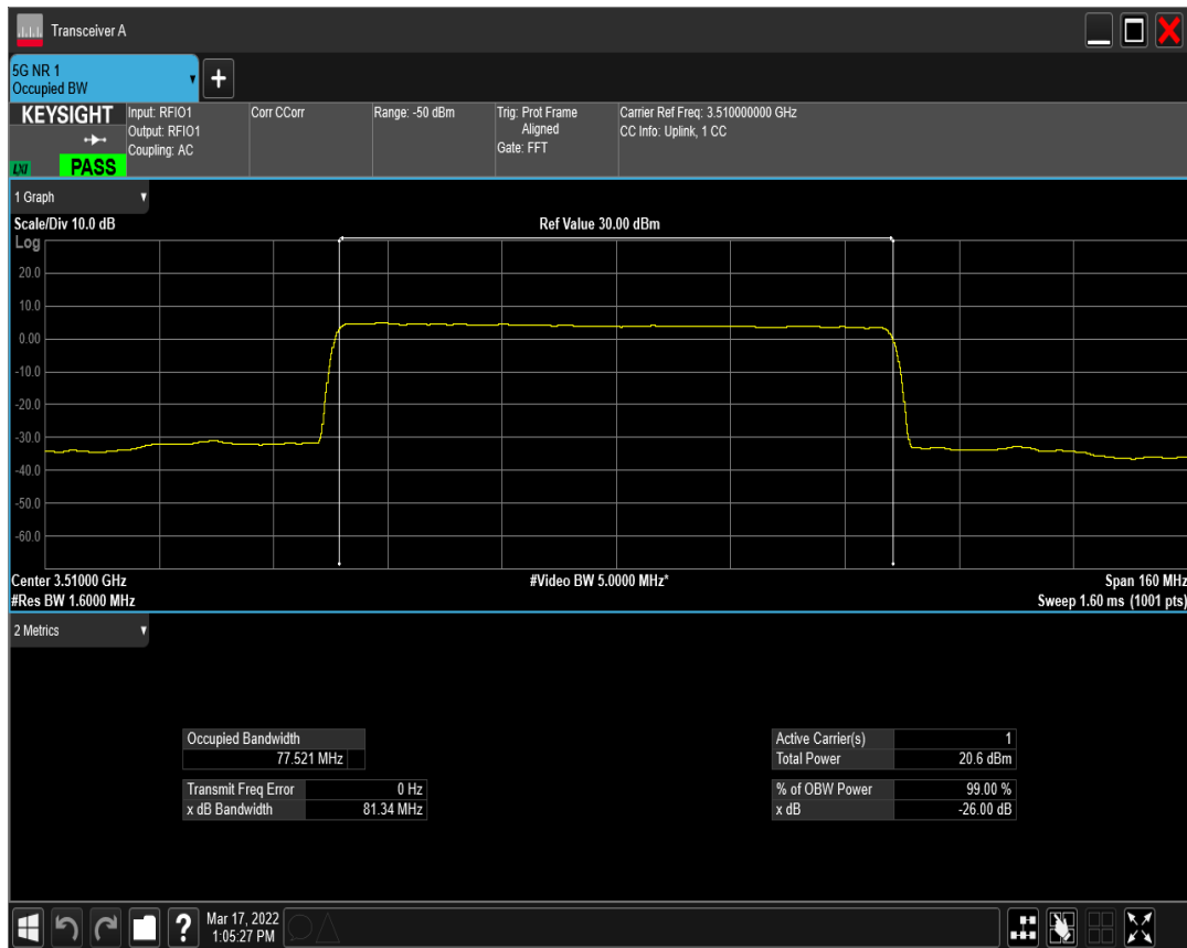
n77(3450-3550) SCS=30kHz CP_QPSK BW=80MHz Channel=634000 RB=217@0
