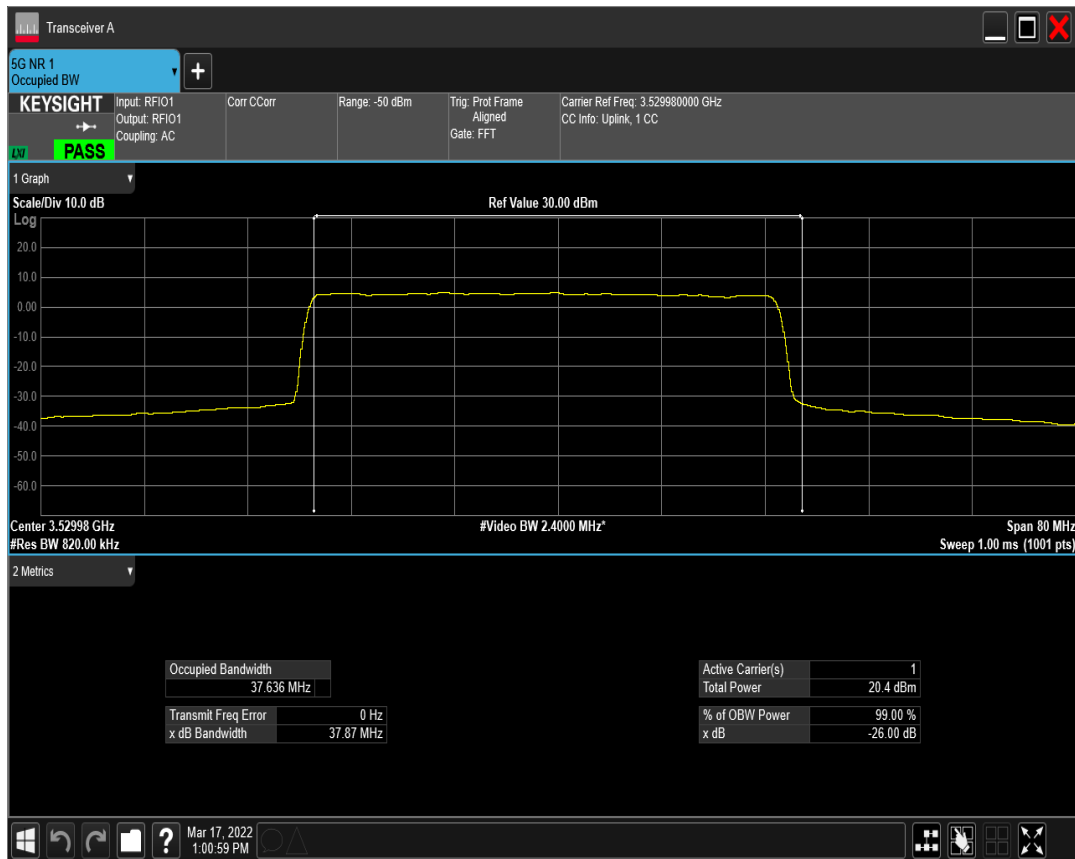
n77(3450-3550) SCS=30kHz CP_QPSK BW=40MHz Channel=635332 RB=106@0
