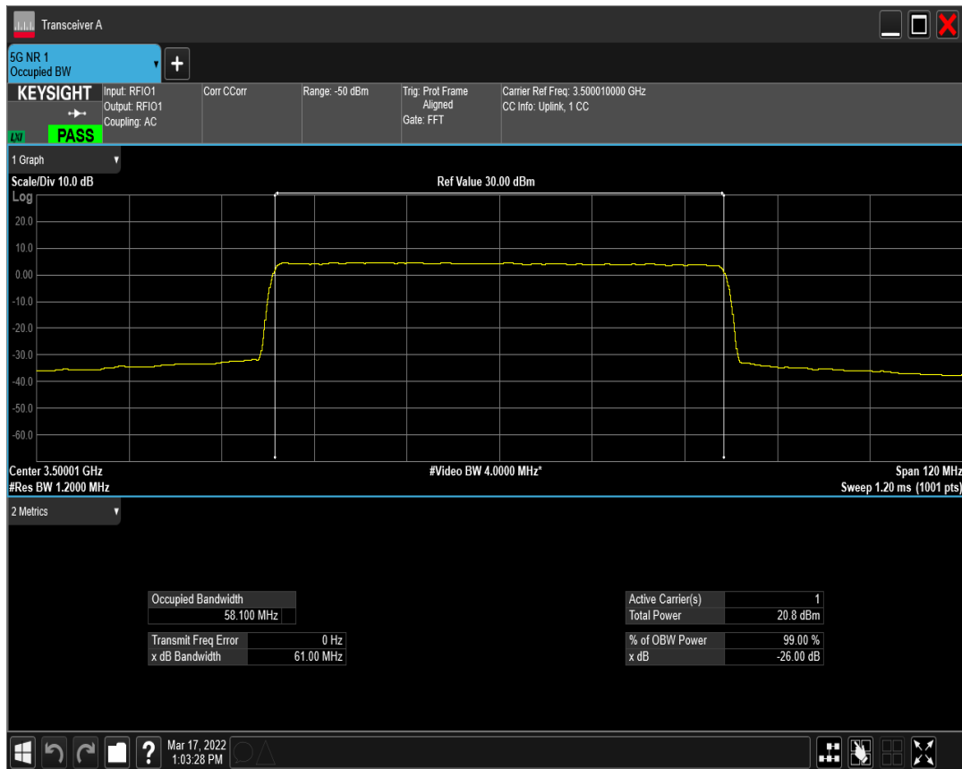
n77(3450-3550) SCS=30kHz CP_QPSK BW=60MHz Channel=633334 RB=162@0
