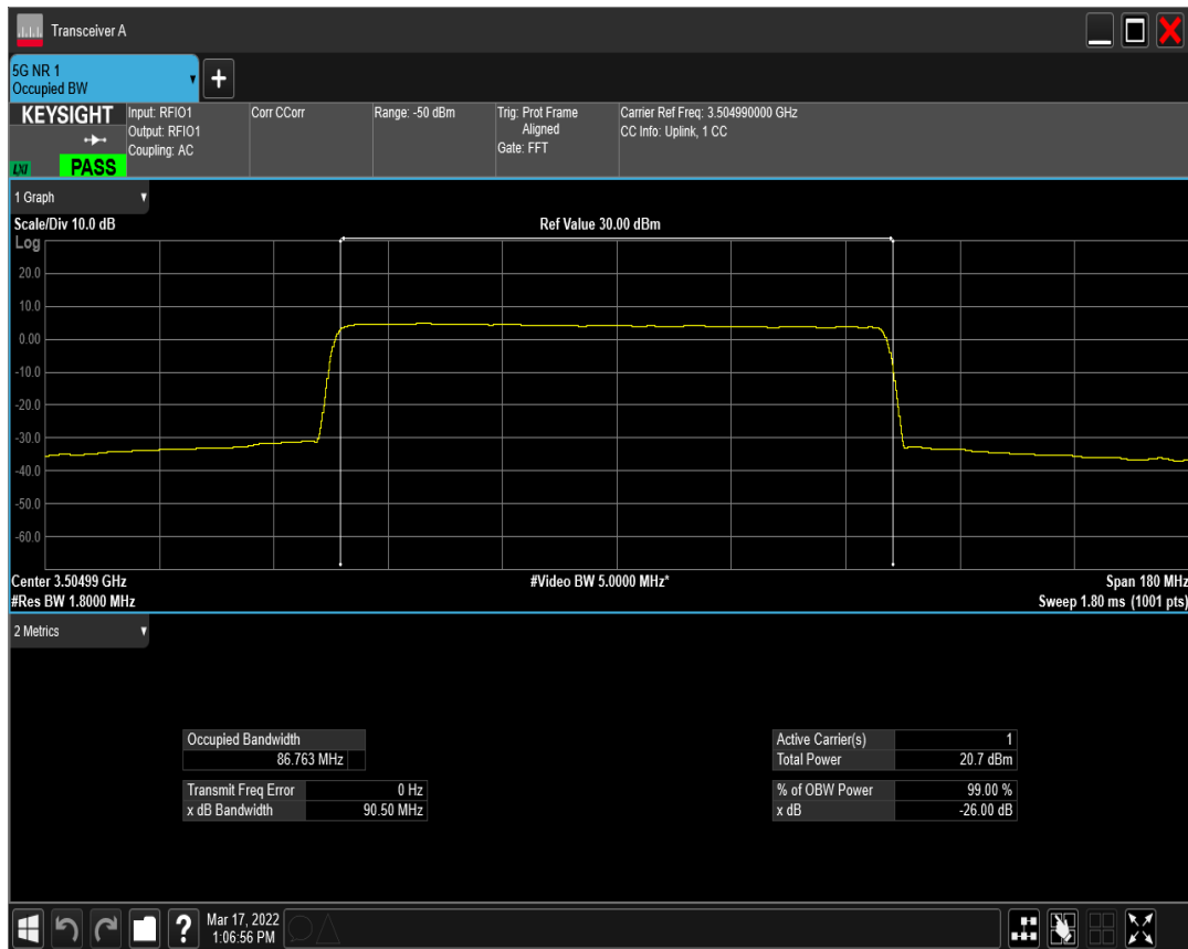
n77(3450-3550) SCS=30kHz CP_QPSK BW=90MHz Channel=633666 RB=245@0
