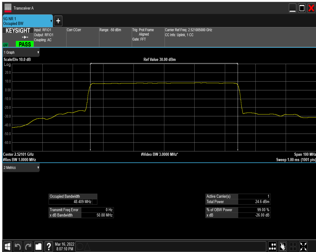
n41 SCS=15kHz DFT_QPSK BW=50MHz Channel=504201 RB=270@0
