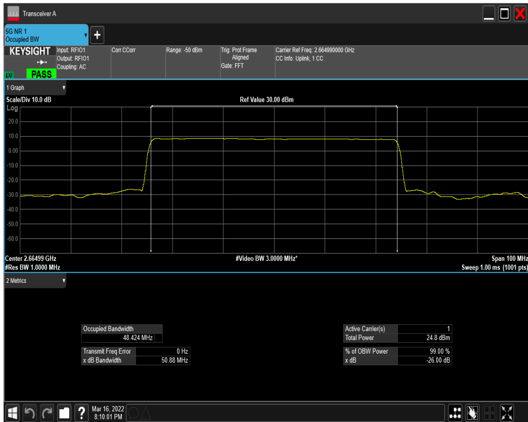
n41 SCS=15kHz DFT_QPSK BW=50MHz Channel=532998 RB=270@0
