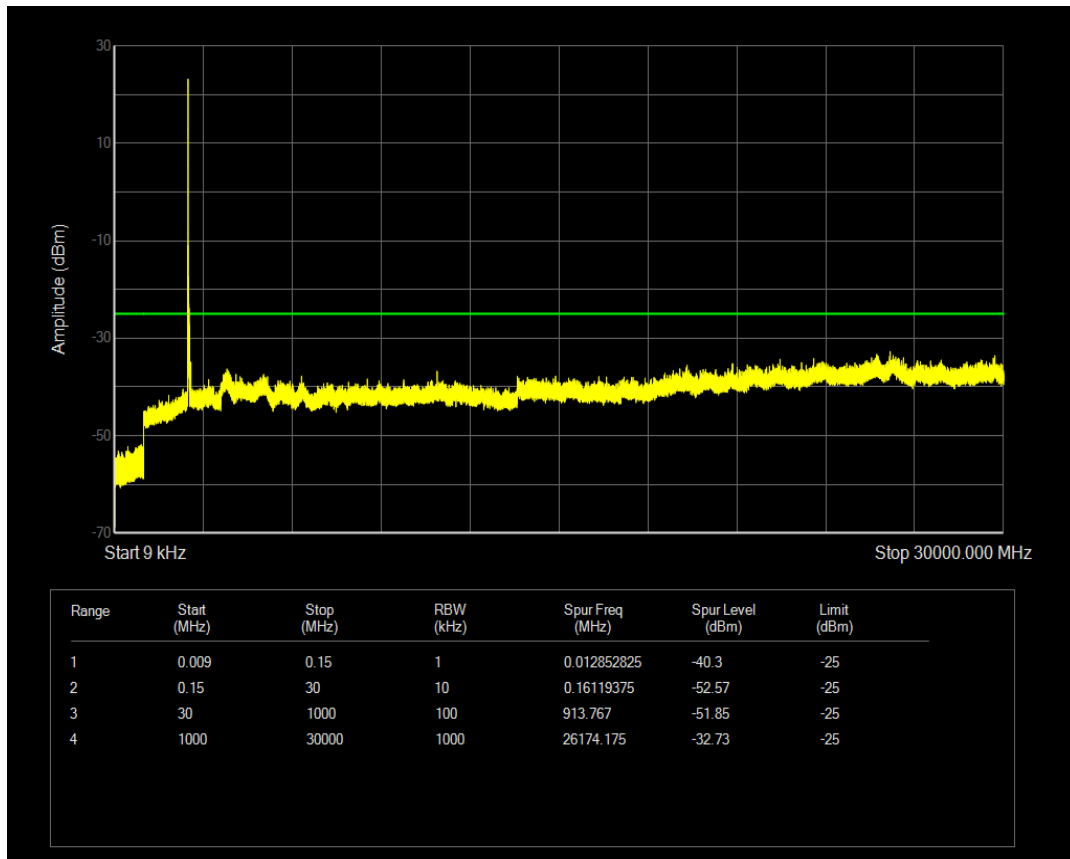
n41 SCS=15kHz DFT_QPSK BW=50MHz Channel=504201 RB=1@269
