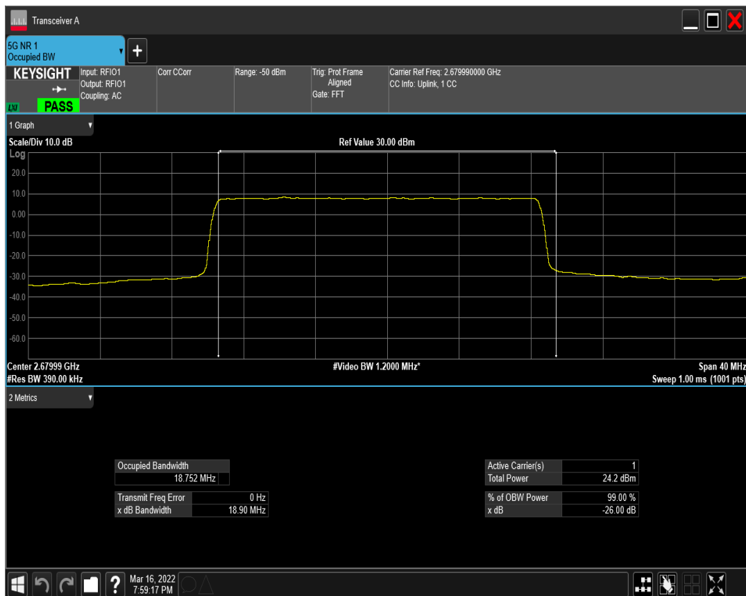
n41 SCS=15kHz DFT_QAM16 BW=20MHz Channel=535998 RB=100@0
