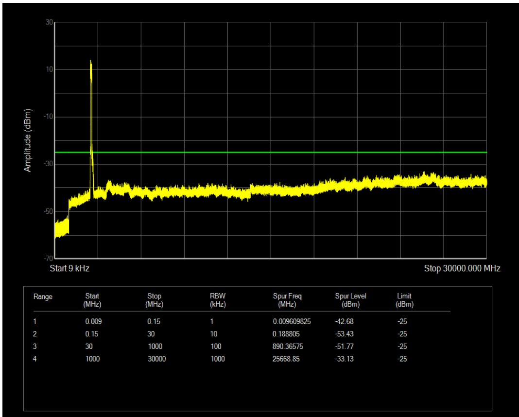
n41 SCS=30kHz DFT_QPSK BW=50MHz Channel=532998 RB=1@132
