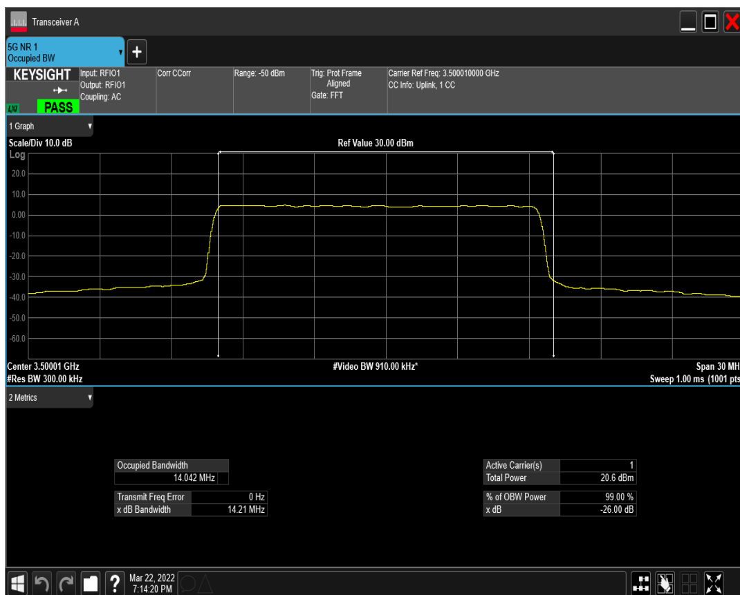
n77(3450-3550) SCS=15kHz CP_QPSK BW=15MHz Channel=633334 RB=79@0
