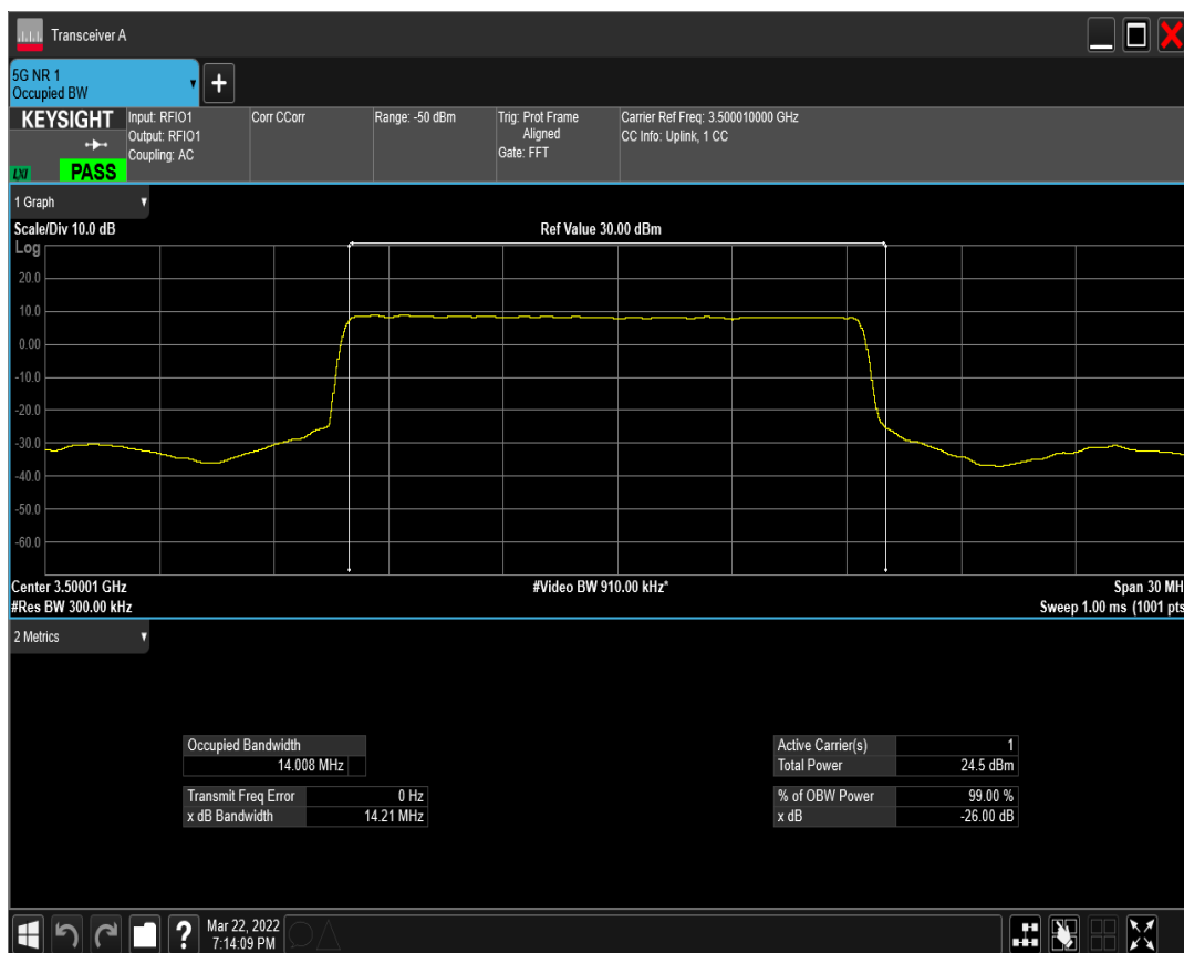
n77(3450-3550) SCS=15kHz DFT_QPSK BW=15MHz Channel=633334 RB=75@0
