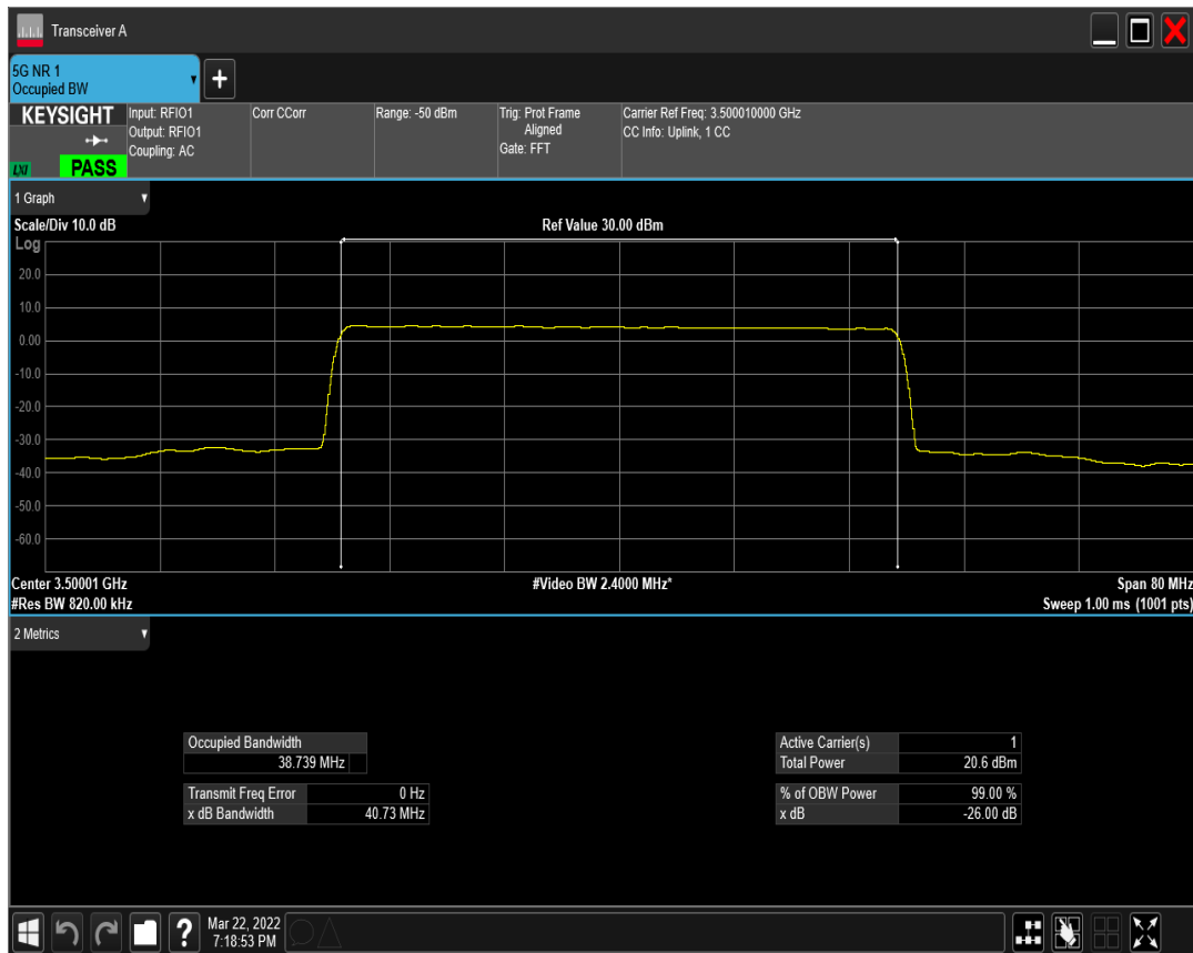
n77(3450-3550) SCS=15kHz CP_QPSK BW=40MHz Channel=633334 RB=216@0
