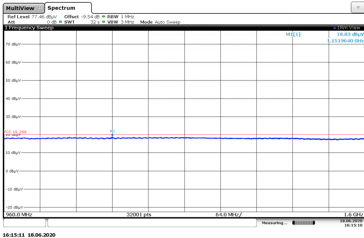
Figure 7.5.2-1: 960 MHz – 1.61 GHz – PRF16 – 1m
