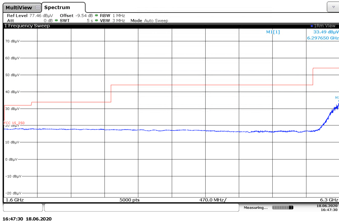
Figure 7.5.2-2: 1.61 GHz – 6.3 GHz – PRF16 – 1m
