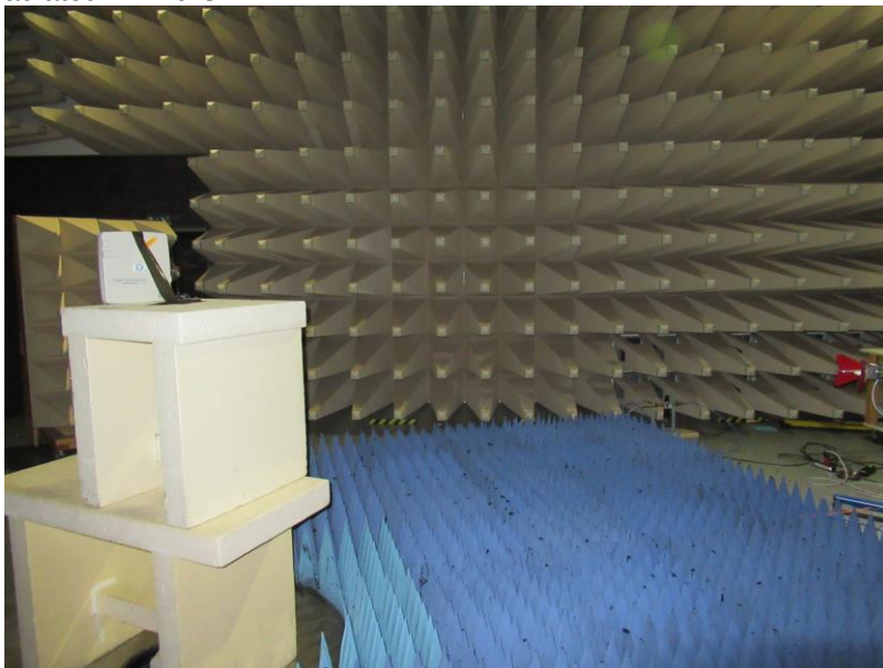
Unwanted emissions, radiated 1 – 10 GHz
