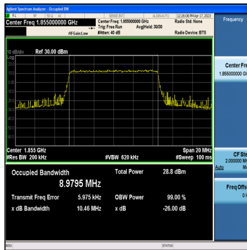
Band2-10MHz-QPSK-18650-50RB#0-8.9795
