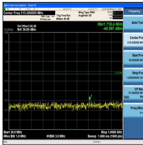
Band2-1.4MHz-16QAM-18900-6RB#0-Range1:30~1000MHz
