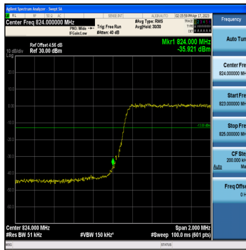
Band5-3MHz-16QAM-20415-15RB#0
