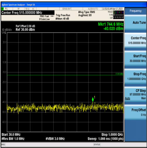
Band2-1.4MHz-QPSK-18607-6RB#0-Range1:30~1000MHz
