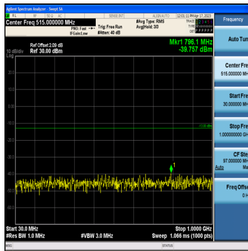
Band2-3MHz-16QAM-18900-15RB#0-Range1:30~1000MHz
