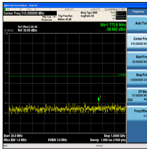
Band2-5MHz-QPSK-18625-25RB#0-Range1:30~1000MHz
