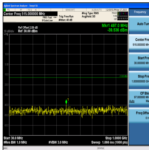
Band2-3MHz-16QAM-18615-15RB#0-Range1:30~1000MHz
