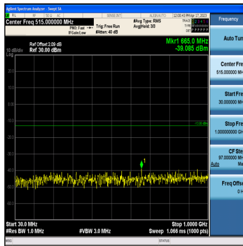
Band2-3MHz-QPSK-18615-15RB#0-Range1:30~1000MHz
