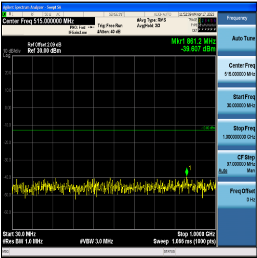
Band2-1.4MHz-16QAM-18607-6RB#0-Range1:30~1000MHz
