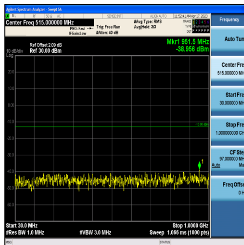
Band2-1.4MHz-QPSK-19193-6RB#0-Range1:30~1000MHz
