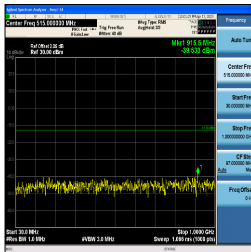
Band2-3MHz-QPSK-19185-15RB#0-Range1:30~1000MHz
