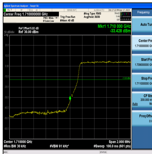
Band66-1.4MHz-QPSK-131979-6RB#0
