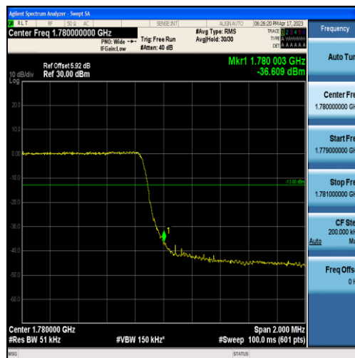
Band66-3MHz-QPSK-132657-15RB#0
