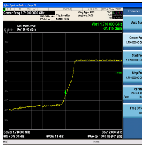
Band66-1.4MHz-16QAM-131979-6RB#0
