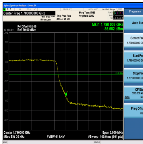
Band66-1.4MHz-16QAM-132665-6RB#0
