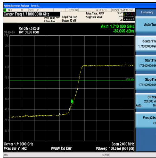
Band66-3MHz-QPSK-131987-15RB#0
