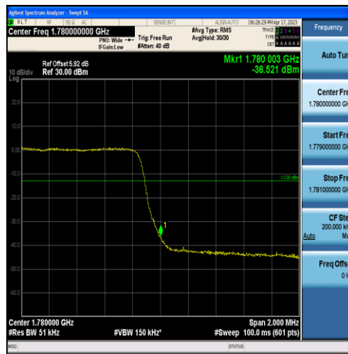
Band66-3MHz-16QAM-132657-15RB#0
