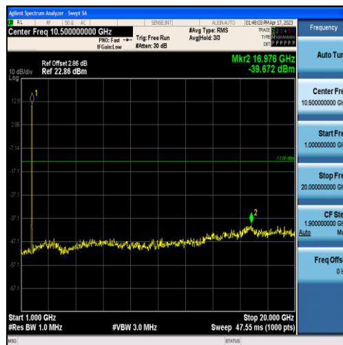
Band4-15MHz-16QAM-20325-75RB#0-Range2:1000~20000MHz
