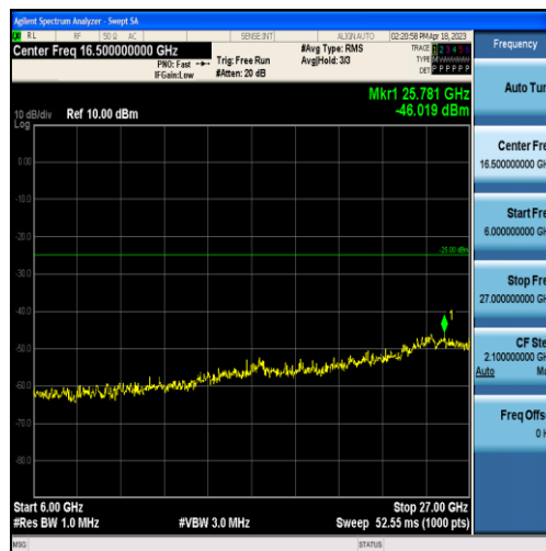
Band7-5MHz-16QAM-20775-25RB#0-Range3:6000~27000MHz
