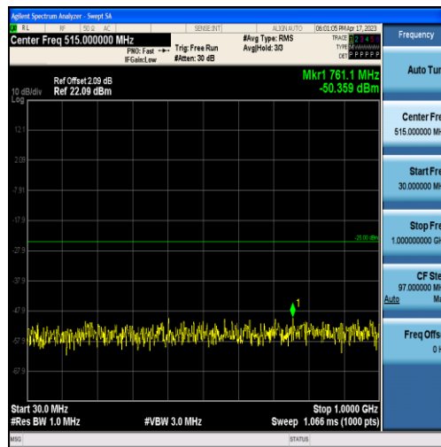
Band7-20MHz-16QAM-21100-60RB#0-Range1:30~1000MHz
