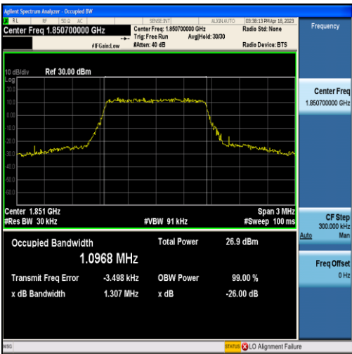
Band2-1.4MHz-16QAM-18607-6RB#0-1.0968
