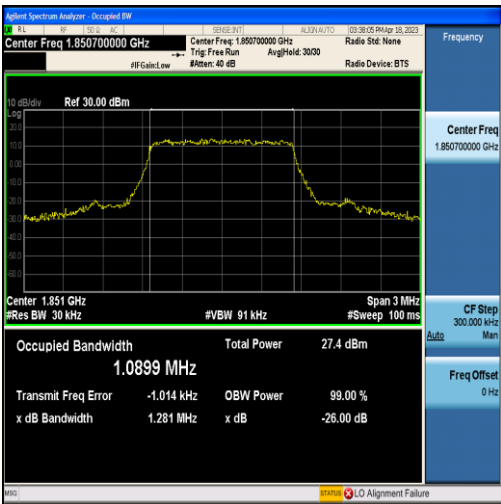
Band2-1.4MHz-QPSK-18607-6RB#0-1.0899
