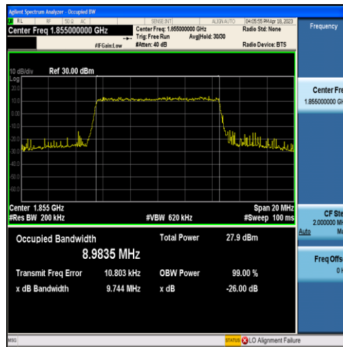
Band2-10MHz-16QAM-18650-50RB#0-8.9835
