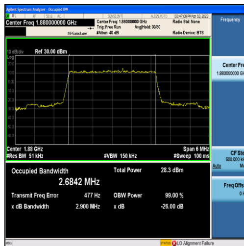
Band2-3MHz-QPSK-18900-15RB#0-2.6842
