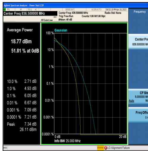
Band5-10MHz-QPSK-20525-50RB#0
