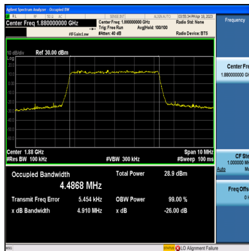
Band2-5MHz-QPSK-18900-25RB#0-4.4868
