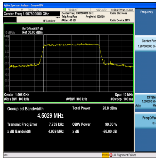
Band2-5MHz-QPSK-19175-25RB#0-4.5029
