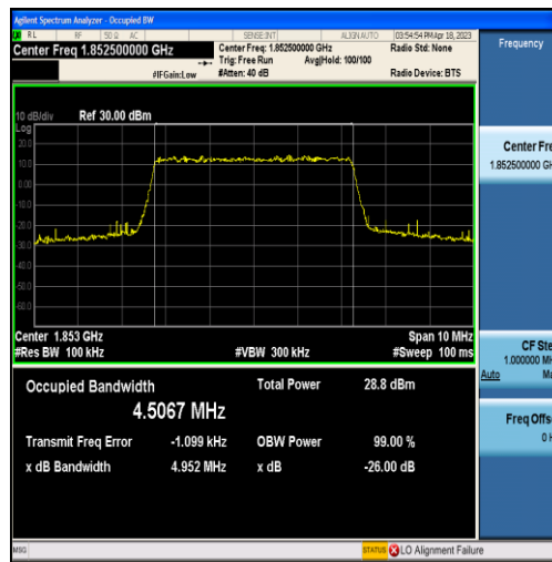
Band2-5MHz-QPSK-18625-25RB#0-4.5067
