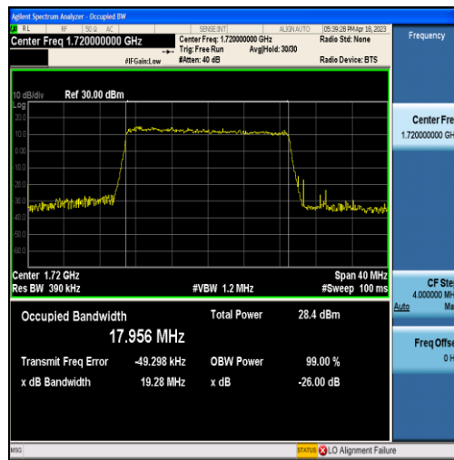
Band4-20MHz-QPSK-20050-100RB#0-17.956
