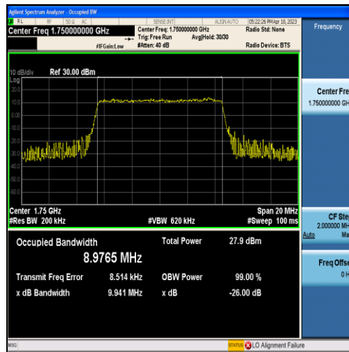
Band4-10MHz-QPSK-20350-50RB#0-8.9765
