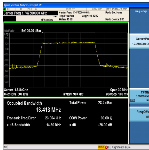
Band4-15MHz-QPSK-20325-75RB#0-13.413
