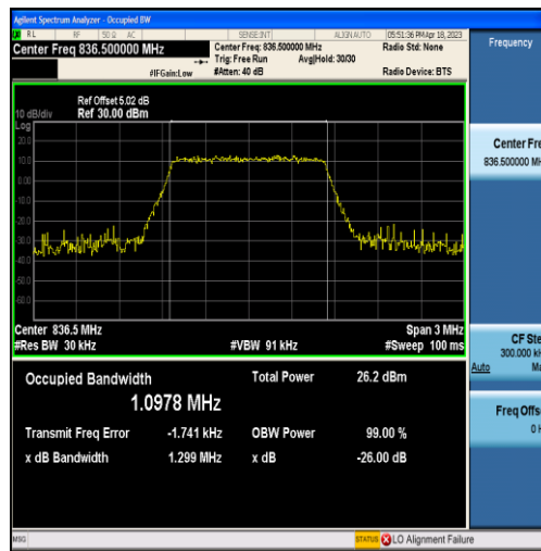
Band5-1.4MHz-16QAM-20525-6RB#0-1.0978
