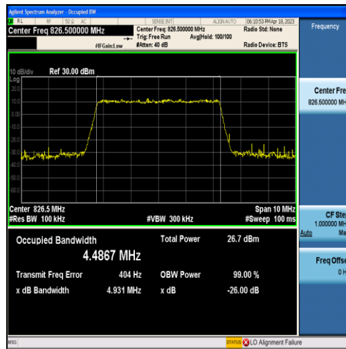
Band5-5MHz-16QAM-20425-25RB#0-4.4867
