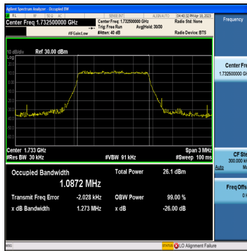
Band4-1.4MHz-16QAM-20175-6RB#0-1.0872
