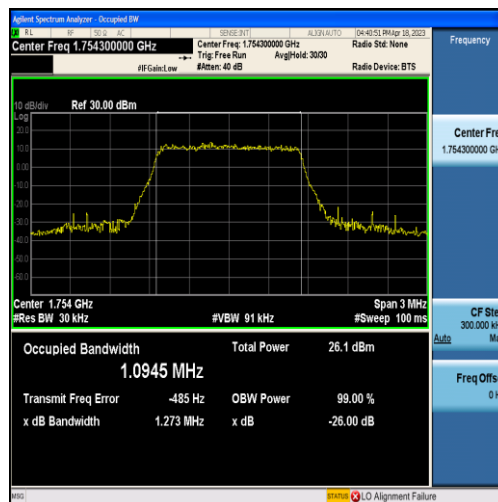
Band4-1.4MHz-16QAM-20393-6RB#0-1.0945
