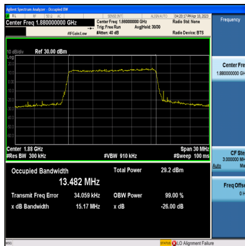
Band2-15MHz-QPSK-18900-75RB#0-13.482
