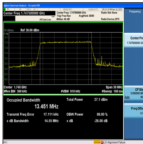
Band4-15MHz-16QAM-20325-75RB#0-13.451
