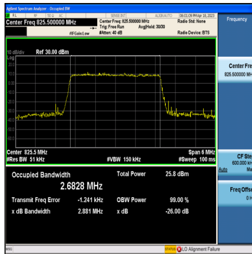
Band5-3MHz-16QAM-20415-15RB#0-2.6828
