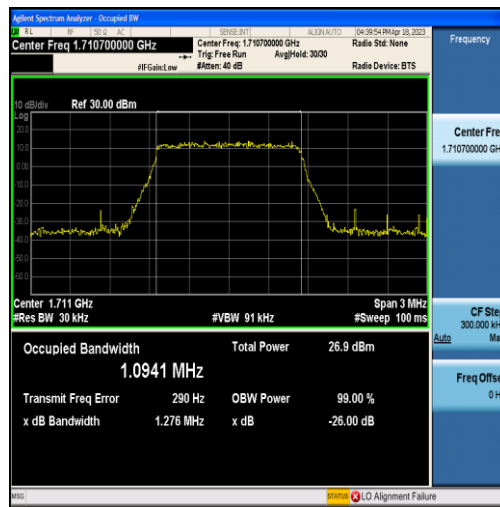
Band4-1.4MHz-QPSK-19957-6RB#0-1.0941
