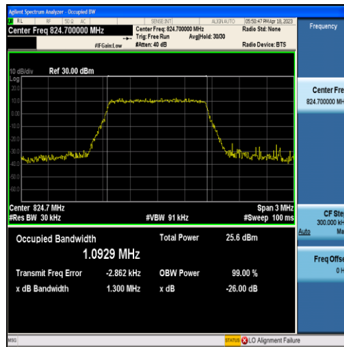
Band5-1.4MHz-16QAM-20407-6RB#0-1.0929
