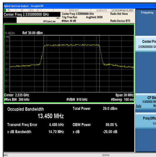
Band7-15MHz-QPSK-21100-75RB#0-13.450
