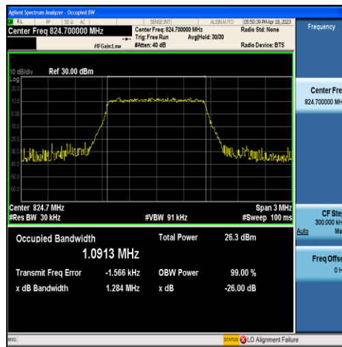
Band5-1.4MHz-QPSK-20407-6RB#0-1.0913
