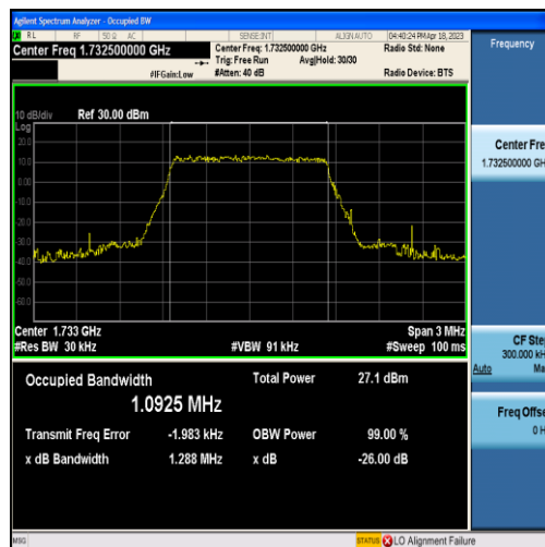
Band4-1.4MHz-QPSK-20175-6RB#0-1.0925
