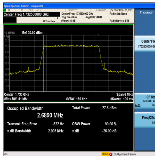
Band4-3MHz-QPSK-20175-15RB#0-2.6890
