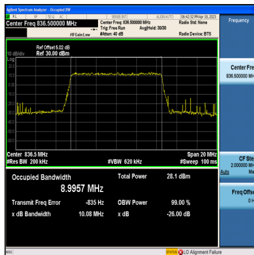
Band5-10MHz-QPSK-20525-50RB#0-8.9957
