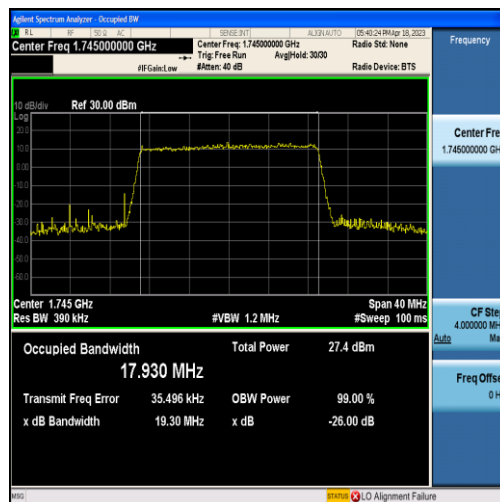
Band4-20MHz-16QAM-20300-100RB#0-17.930
