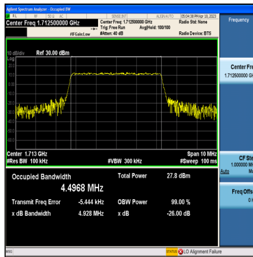
Band4-5MHz-QPSK-19975-25RB#0-4.4968
