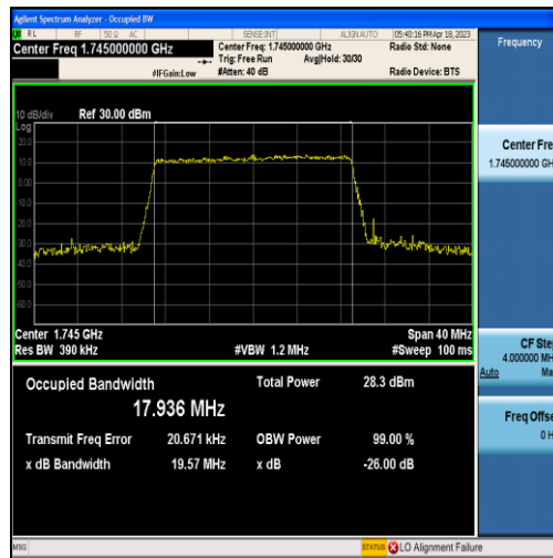
Band4-20MHz-QPSK-20300-100RB#0-17.936
