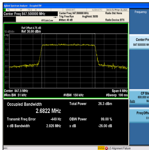
Band5-3MHz-16QAM-20635-15RB#0-2.6822
