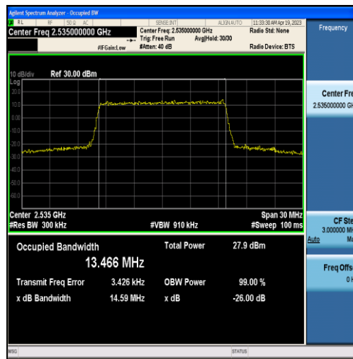
Band7-15MHz-16QAM-21100-75RB#0-13.466
