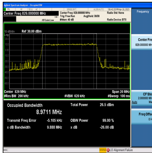
Band5-10MHz-16QAM-20450-50RB#0-8.9711
