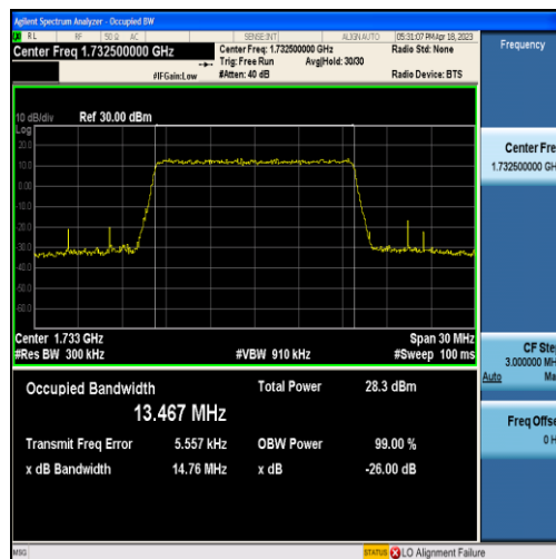
Band4-15MHz-QPSK-20175-75RB#0-13.467
