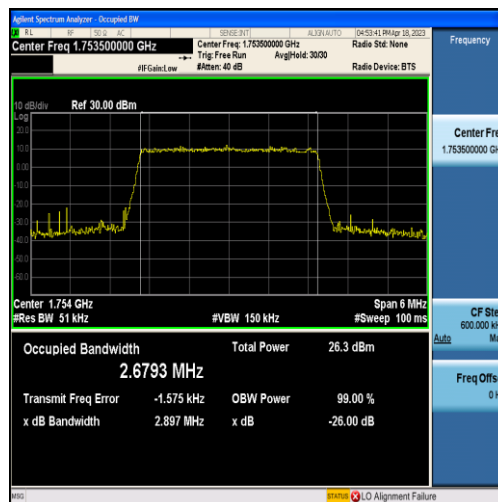
Band4-3MHz-16QAM-20385-15RB#0-2.6793
