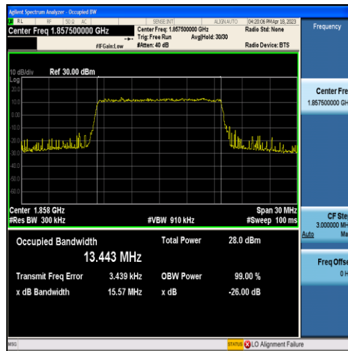
Band2-15MHz-16QAM-18675-75RB#0-13.443
