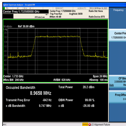
Band4-10MHz-QPSK-20175-50RB#0-8.9658
