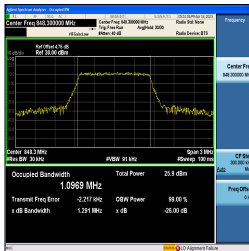
Band5-1.4MHz-16QAM-20643-6RB#0-1.0969
