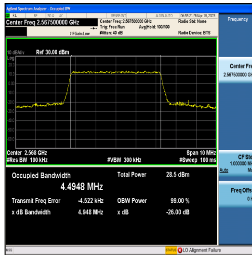
Band7-5MHz-QPSK-21425-25RB#0-4.4948
