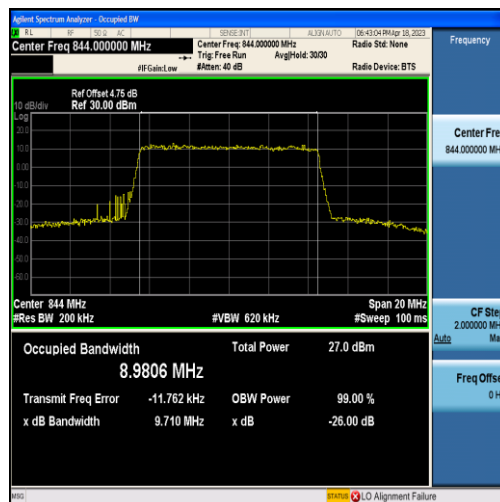
Band5-10MHz-16QAM-20600-50RB#0-8.9806
