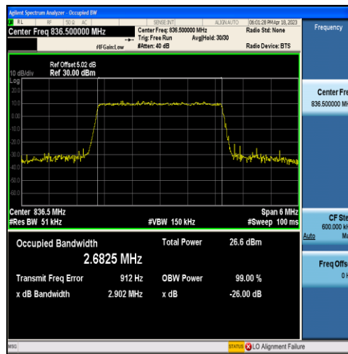
Band5-3MHz-16QAM-20525-15RB#0-2.6825
