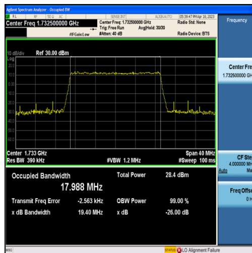
Band4-20MHz-QPSK-20175-100RB#0-17.988
