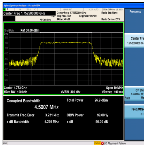
Band4-5MHz-16QAM-20375-25RB#0-4.5007
