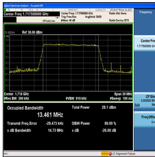
Band4-15MHz-QPSK-20025-75RB#0-13.461
