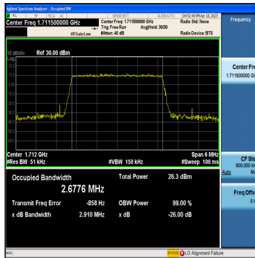
Band4-3MHz-16QAM-19965-15RB#0-2.6776
