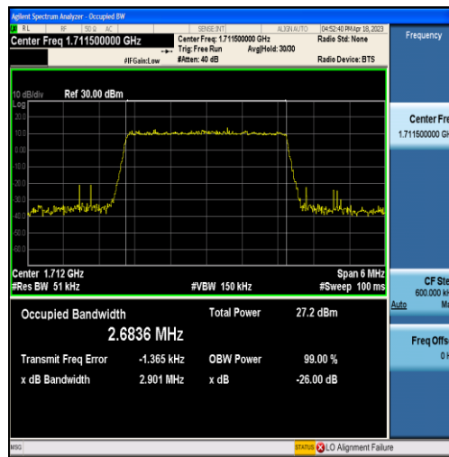
Band4-3MHz-QPSK-19965-15RB#0-2.6836
