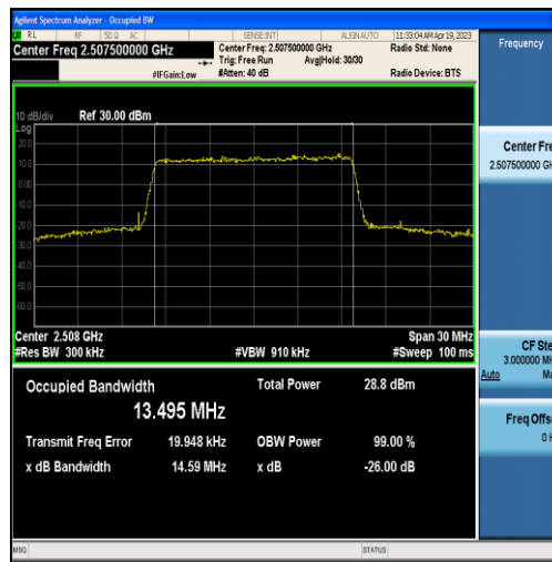
Band7-15MHz-QPSK-20825-75RB#0-13.495
