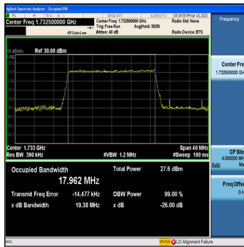
Band4-20MHz-16QAM-20175-100RB#0-17.962
