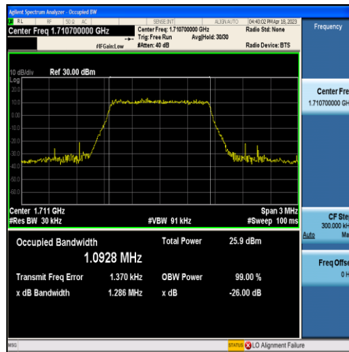
Band4-1.4MHz-16QAM-19957-6RB#0-1.0928
