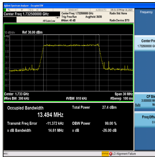
Band4-15MHz-16QAM-20175-75RB#0-13.494
