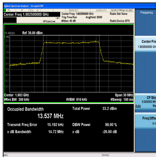
Band2-15MHz-QPSK-19125-75RB#0-13.537
