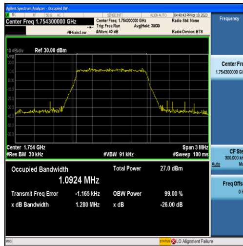
Band4-1.4MHz-QPSK-20393-6RB#0-1.0924
