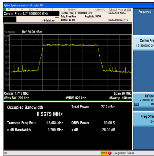
Band4-10MHz-16QAM-20000-50RB#0-8.9679
