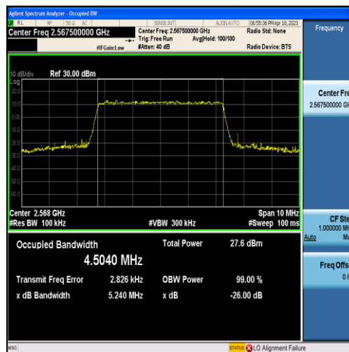
Band7-5MHz-16QAM-21425-25RB#0-4.5040
