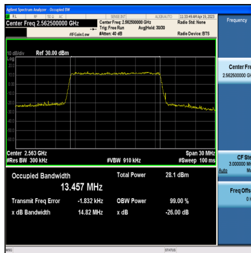
Band7-15MHz-16QAM-21375-75RB#0-13.457
