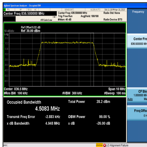
Band5-5MHz-QPSK-20525-25RB#0-4.5083
