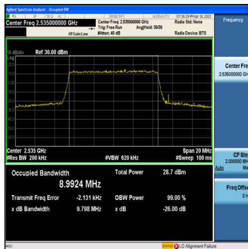
Band7-10MHz-QPSK-21100-50RB#0-8.9924
