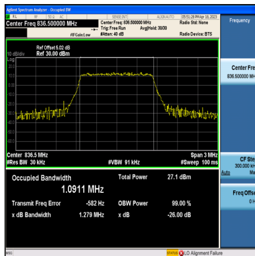
Band5-1.4MHz-QPSK-20525-6RB#0-1.0911
