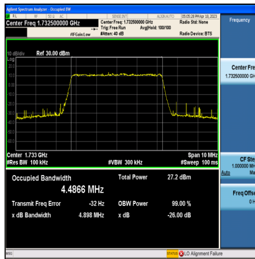
Band4-5MHz-16QAM-20175-25RB#0-4.4866
