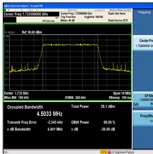
Band4-5MHz-QPSK-20175-25RB#0-4.5033
