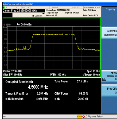
Band7-5MHz-16QAM-21100-25RB#0-4.5000
