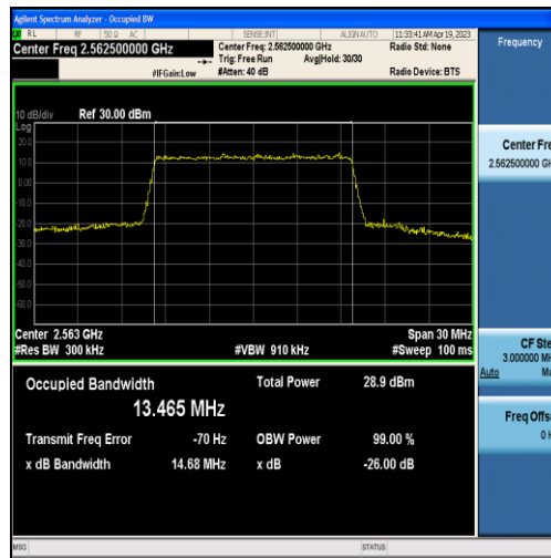
Band7-15MHz-QPSK-21375-75RB#0-13.465
