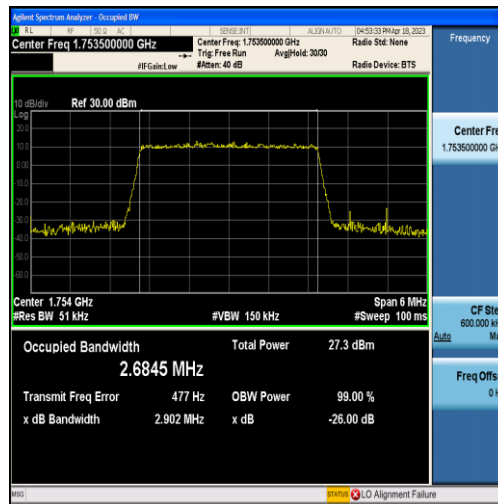
Band4-3MHz-QPSK-20385-15RB#0-2.6845
