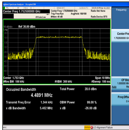
Band4-5MHz-QPSK-20375-25RB#0-4.4891
