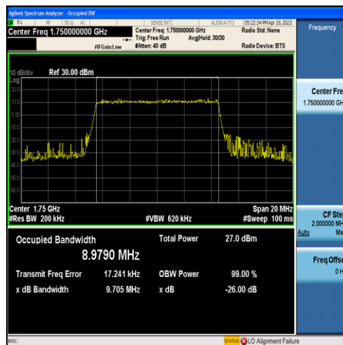
Band4-10MHz-16QAM-20350-50RB#0-8.9790
