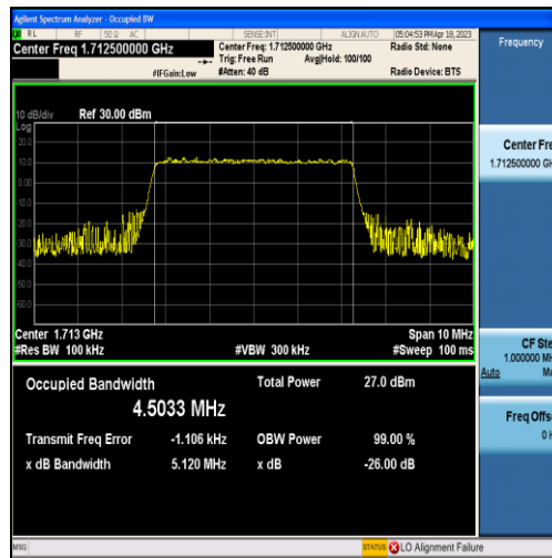
Band4-5MHz-16QAM-19975-25RB#0-4.5033
