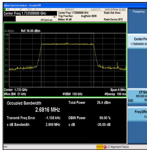
Band4-3MHz-16QAM-20175-15RB#0-2.6816
