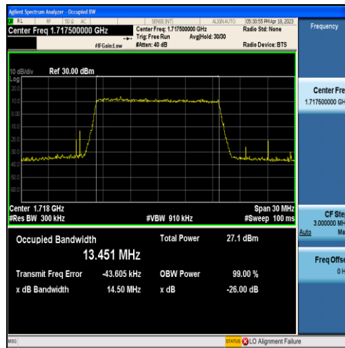
Band4-15MHz-16QAM-20025-75RB#0-13.451
