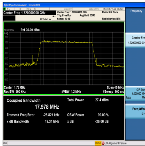
Band4-20MHz-16QAM-20050-100RB#0-17.978
