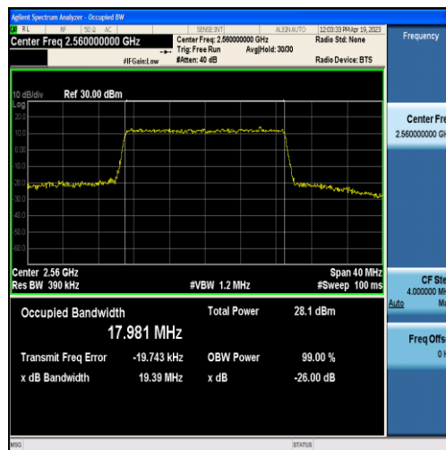
Band7-20MHz-16QAM-21350-100RB#0-17.981
