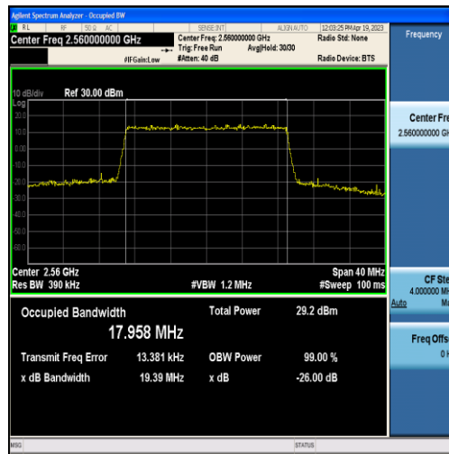
Band7-20MHz-QPSK-21350-100RB#0-17.958
