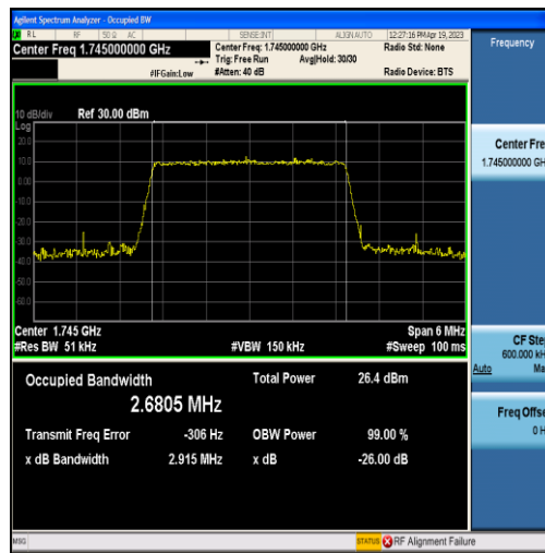
Band66-3MHz-16QAM-132322-15RB#0-2.6805
