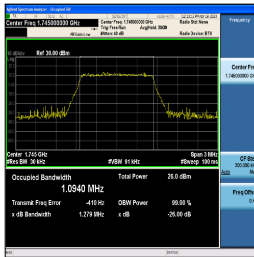
Band66-1.4MHz-16QAM-132322-6RB#0-1.0940
