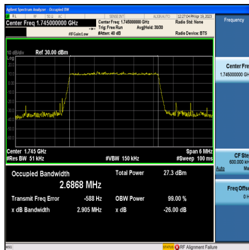
Band66-3MHz-QPSK-132322-15RB#0-2.6868
