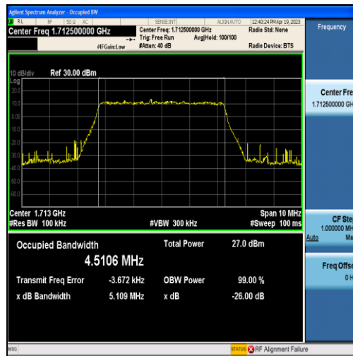
Band66-5MHz-16QAM-131997-25RB#0-4.5106
