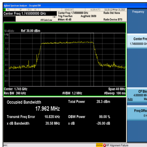
Band66-20MHz-QPSK-132322-100RB#0-17.962
