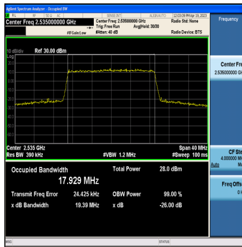
Band7-20MHz-16QAM-21100-100RB#0-17.929
