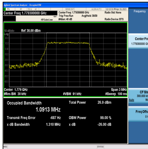
Band66-1.4MHz-QPSK-132665-6RB#0-1.0913
