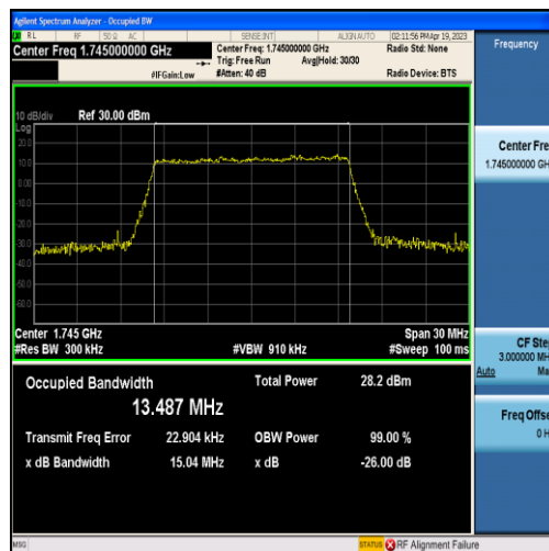
Band66-15MHz-QPSK-132322-75RB#0-13.487
