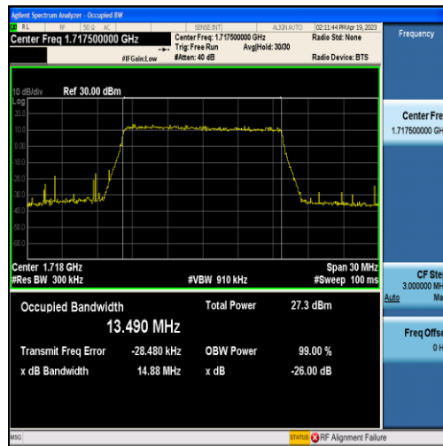
Band66-15MHz-16QAM-132047-75RB#0-13.490
