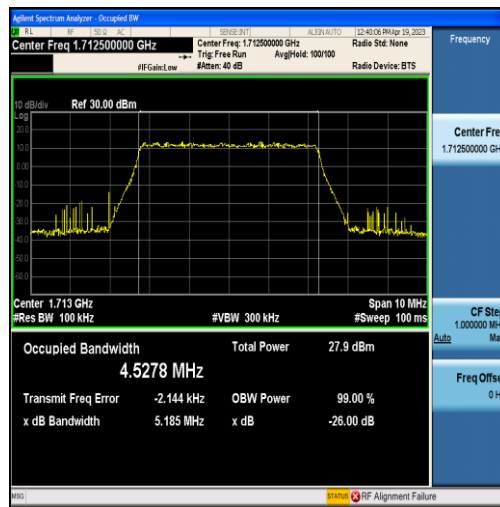
Band66-5MHz-QPSK-131997-25RB#0-4.5278
