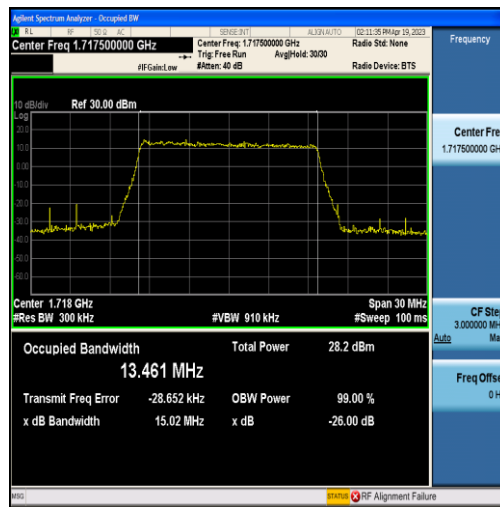
Band66-15MHz-QPSK-132047-75RB#0-13.461
