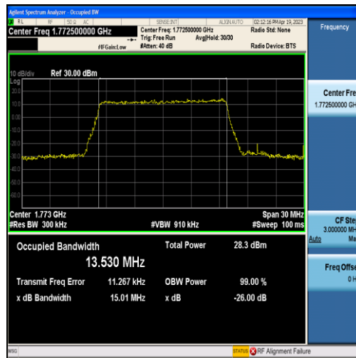
Band66-15MHz-QPSK-132597-75RB#0-13.530
