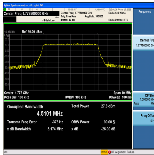
Band66-5MHz-QPSK-132647-25RB#0-4.5101
