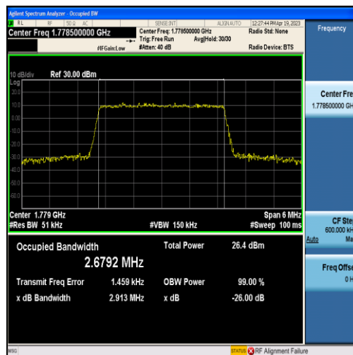
Band66-3MHz-16QAM-132657-15RB#0-2.6792
