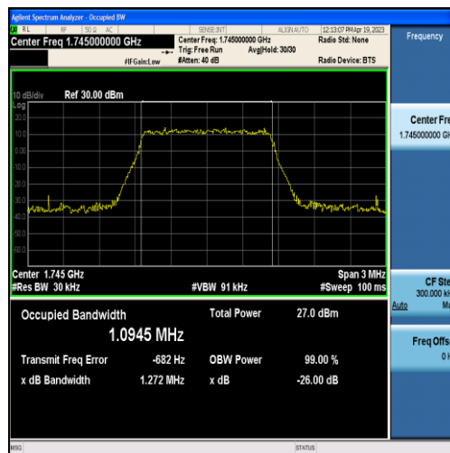
Band66-1.4MHz-QPSK-132322-6RB#0-1.0945
