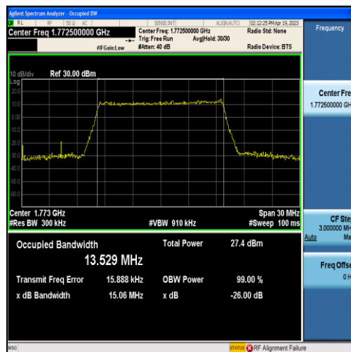
Band66-15MHz-16QAM-132597-75RB#0-13.529
