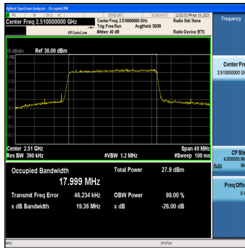
Band7-20MHz-16QAM-20850-100RB#0-17.999
