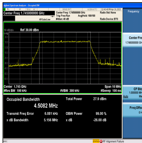
Band66-5MHz-QPSK-132322-25RB#0-4.5082
