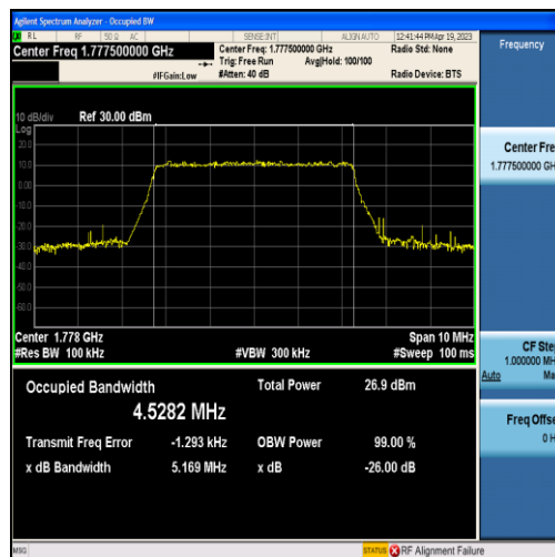
Band66-5MHz-16QAM-132647-25RB#0-4.5282
