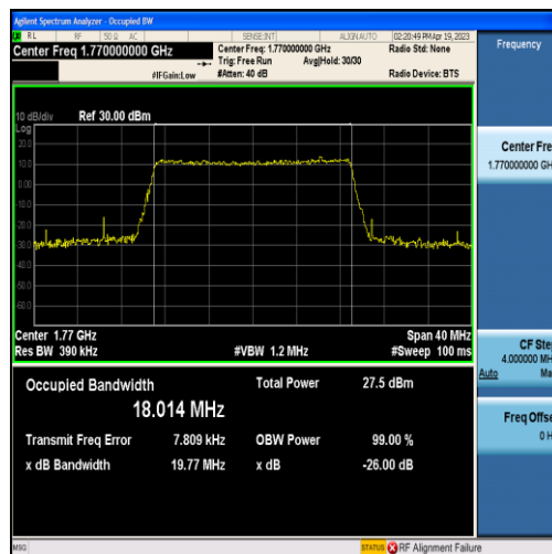
Band66-20MHz-16QAM-132572-100RB#0-18.014
