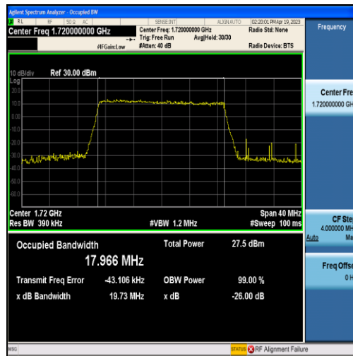
Band66-20MHz-16QAM-132072-100RB#0-17.966
