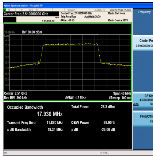
Band7-20MHz-QPSK-20850-100RB#0-17.936
