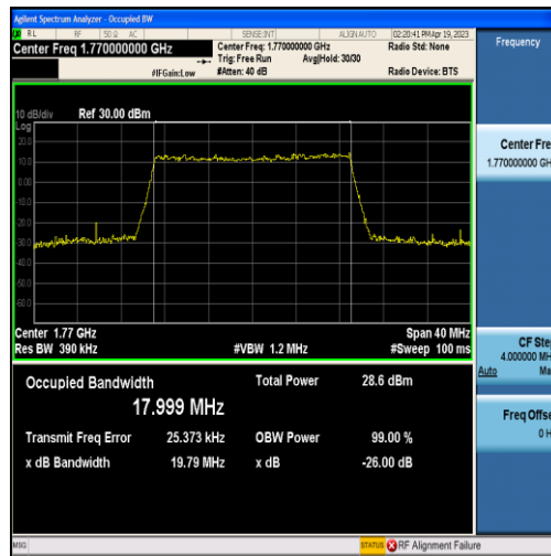
Band66-20MHz-QPSK-132572-100RB#0-17.999
