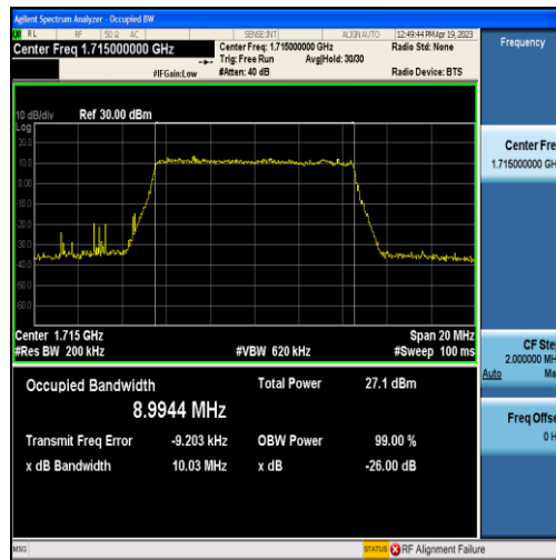
Band66-10MHz-16QAM-132022-50RB#0-8.9944
