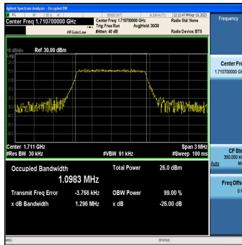
Band66-1.4MHz-16QAM-131979-6RB#0-1.0983
