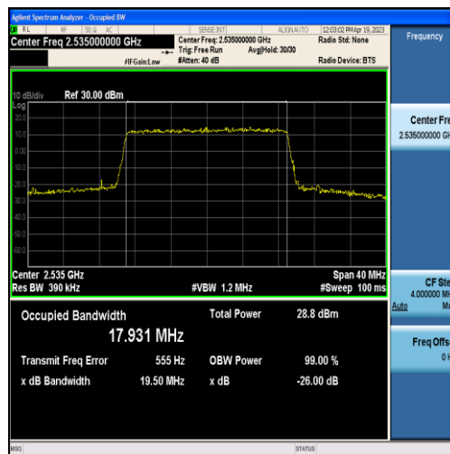
Band7-20MHz-QPSK-21100-100RB#0-17.931
