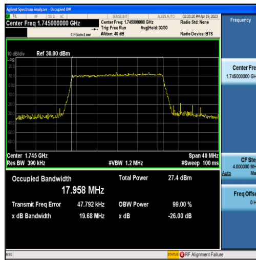
Band66-20MHz-16QAM-132322-100RB#0-17.958
