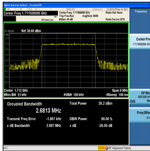
Band66-3MHz-16QAM-131987-15RB#0-2.6813
