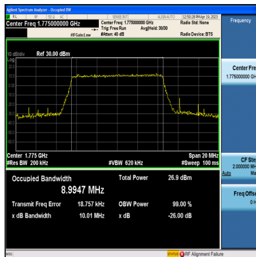
Band66-10MHz-16QAM-132622-50RB#0-8.9947
