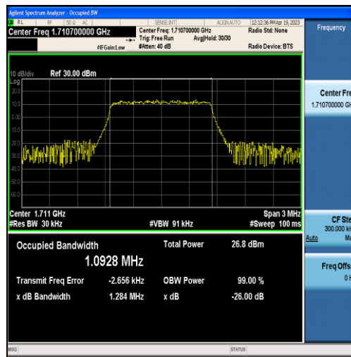
Band66-1.4MHz-QPSK-131979-6RB#0-1.0928
