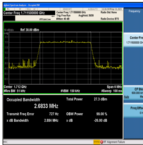
Band66-3MHz-QPSK-131987-15RB#0-2.6833
