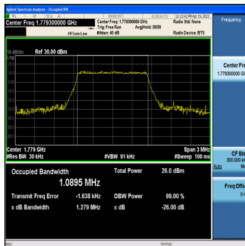
Band66-1.4MHz-16QAM-132665-6RB#0-1.0895
