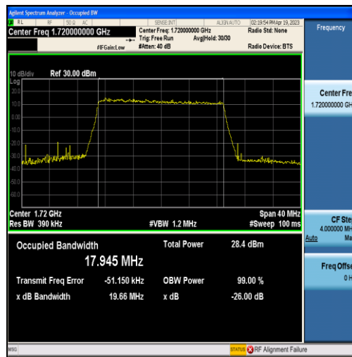
Band66-20MHz-QPSK-132072-100RB#0-17.945
