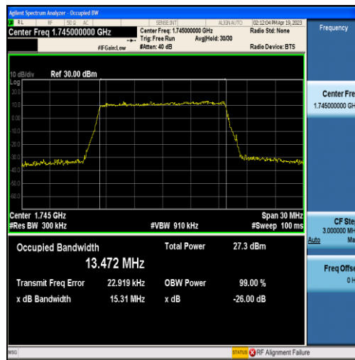
Band66-15MHz-16QAM-132322-75RB#0-13.472
