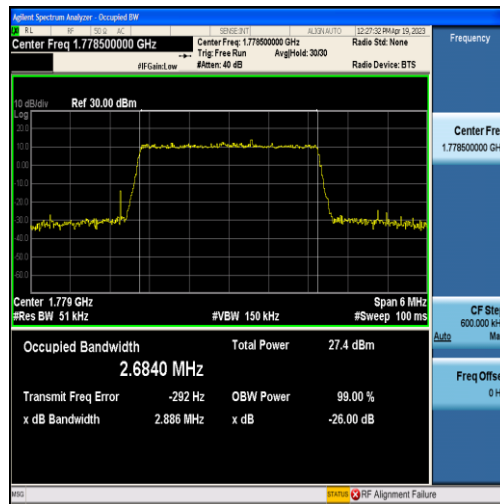
Band66-3MHz-QPSK-132657-15RB#0-2.6840
