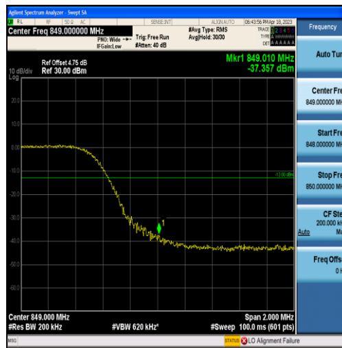
Band5-10MHz-QPSK-20600-50RB#0
