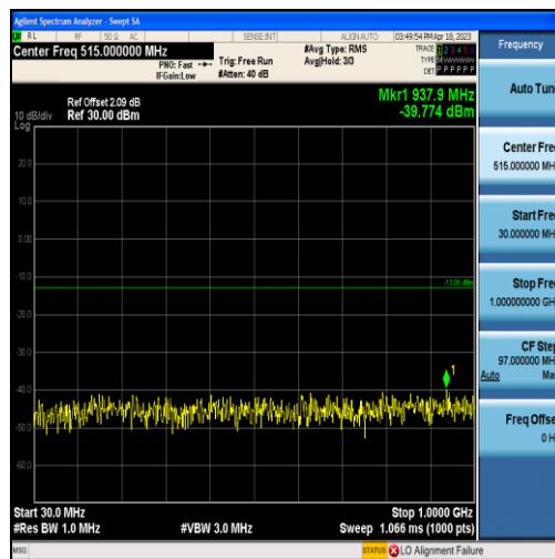
Band2-3MHz-16QAM-19185-15RB#0-Range1:30~1000MHz
