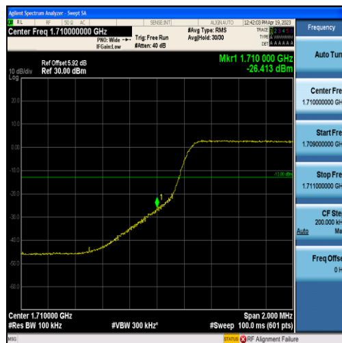
Band66-5MHz-QPSK-131997-25RB#0
