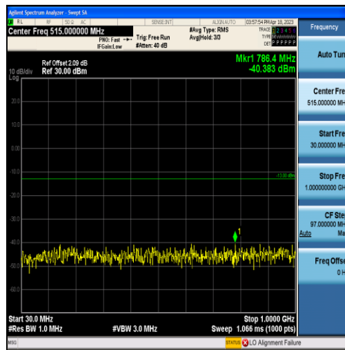
Band2-5MHz-16QAM-18625-25RB#0-Range1:30~1000MHz
