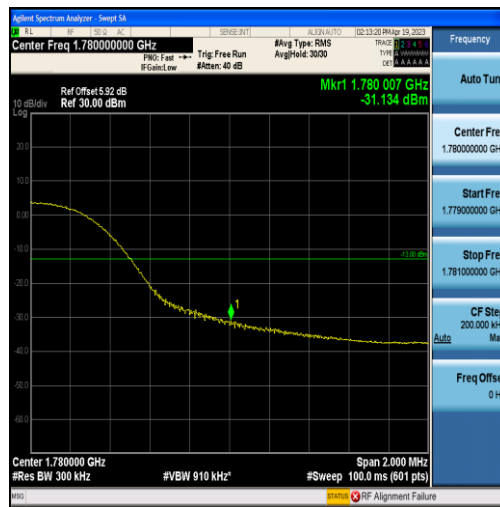
Band66-15MHz-QPSK-132597-75RB#0
