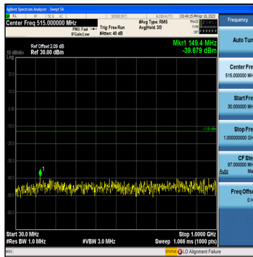
Band2-3MHz-16QAM-18615-15RB#0-Range1:30~1000MHz
