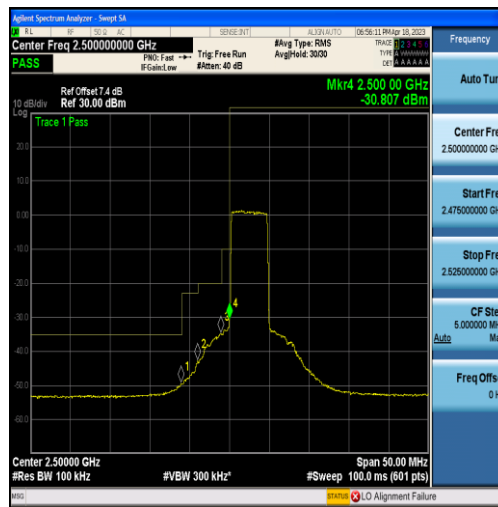
Band7-5MHz-16QAM-20775-25RB#0
