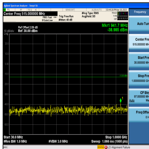
Band2-3MHz-QPSK-18900-15RB#0-Range1:30~1000MHz
