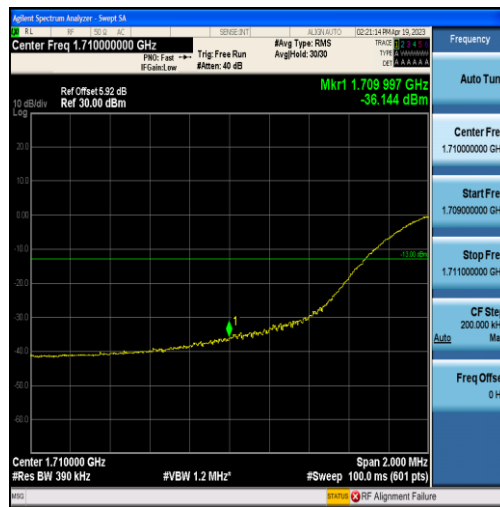
Band66-20MHz-16QAM-132072-100RB#0
