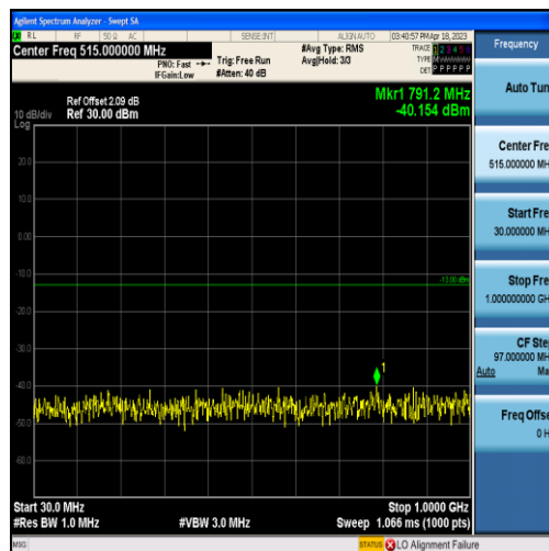
Band2-1.4MHz-16QAM-19193-6RB#0-Range1:30~1000MHz
