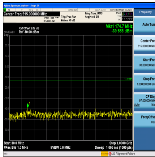
Band2-3MHz-QPSK-19185-15RB#0-Range1:30~1000MHz
