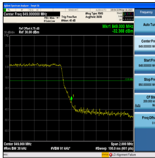
Band5-1.4MHz-QPSK-20643-6RB#0
