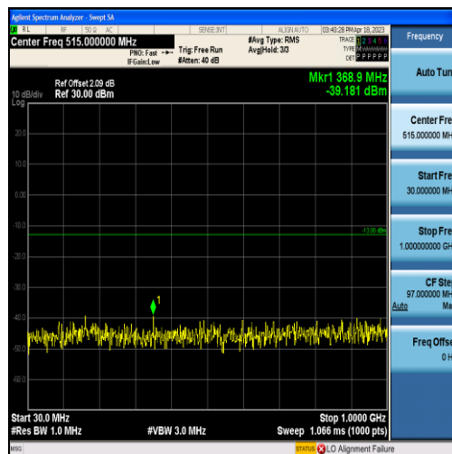
Band2-1.4MHz-QPSK-18900-6RB#0-Range1:30~1000MHz
