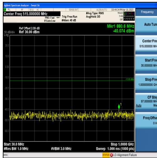
Band2-3MHz-16QAM-18900-15RB#0-Range1:30~1000MHz
