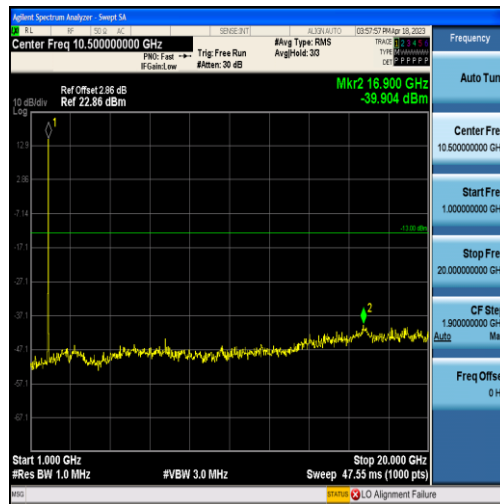
Band2-5MHz-16QAM-18625-25RB#0-Range2:1000~20000MHz
