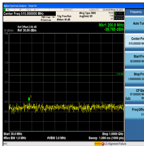
Band2-1.4MHz-QPSK-18607-6RB#0-Range1:30~1000MHz
