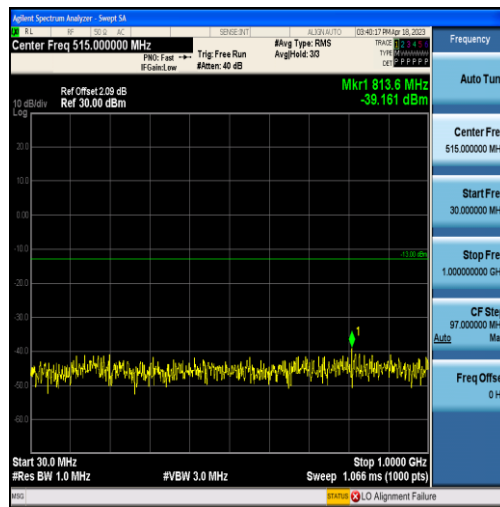
Band2-1.4MHz-16QAM-18607-6RB#0-Range1:30~1000MHz
