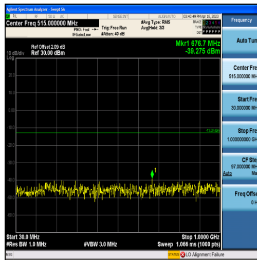
Band2-1.4MHz-QPSK-19193-6RB#0-Range1:30~1000MHz
