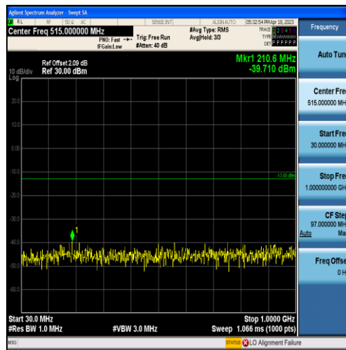
Band4-15MHz-16QAM-20025-75RB#0-Range1:30~1000MHz
