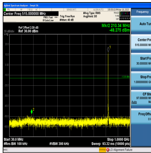
Band5-1.4MHz-16QAM-20407-6RB#0-Range1:30~1000MHz
