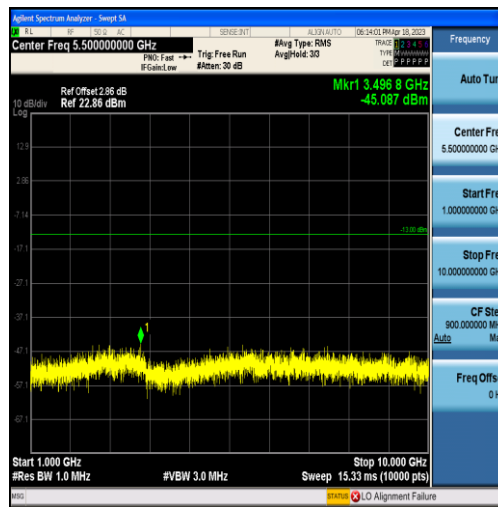
Band5-5MHz-QPSK-20525-25RB#0-Range2:1000~10000MHz
