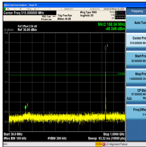
Band5-1.4MHz-16QAM-20525-6RB#0-Range1:30~1000MHz
