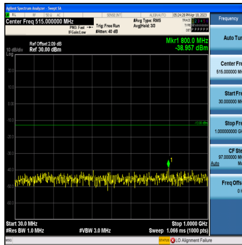
Band4-10MHz-16QAM-20175-50RB#0-Range1:30~1000MHz
