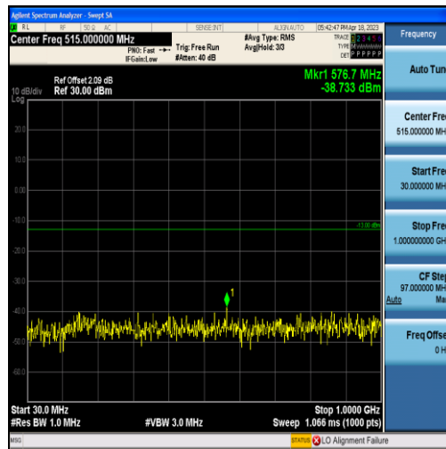
Band4-20MHz-16QAM-20175-100RB#0-Range1:30~1000MHz
