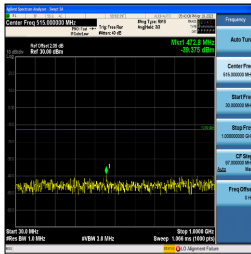
Band4-20MHz-QPSK-20300-100RB#0-Range1:30~1000MHz
