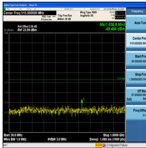
Band7-5MHz-QPSK-20775-25RB#0-Range1:30~1000MHz
