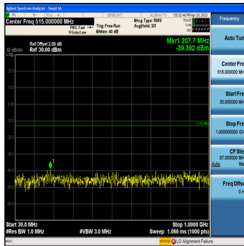
Band4-15MHz-QPSK-20025-75RB#0-Range1:30~1000MHz
