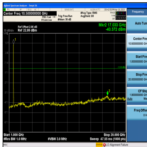
Band4-20MHz-16QAM-20175-100RB#0-Range2:1000~20000MHz
