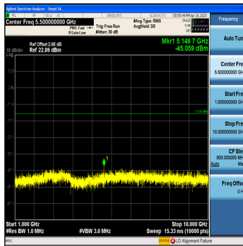
Band5-1.4MHz-16QAM-20643-6RB#0-Range2:1000~10000MHz
