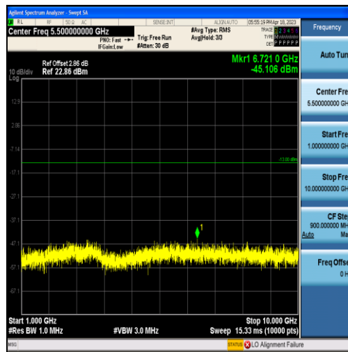
Band5-1.4MHz-QPSK-20525-6RB#0-Range2:1000~10000MHz
