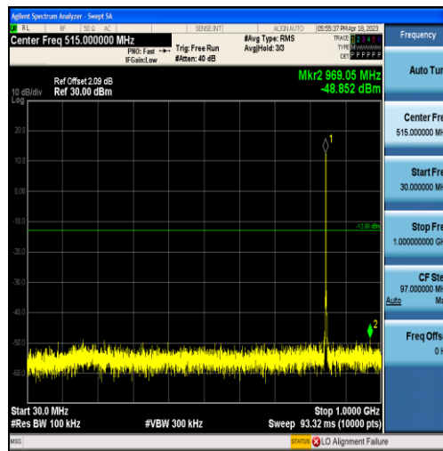
Band5-1.4MHz-QPSK-20643-6RB#0-Range1:30~1000MHz
