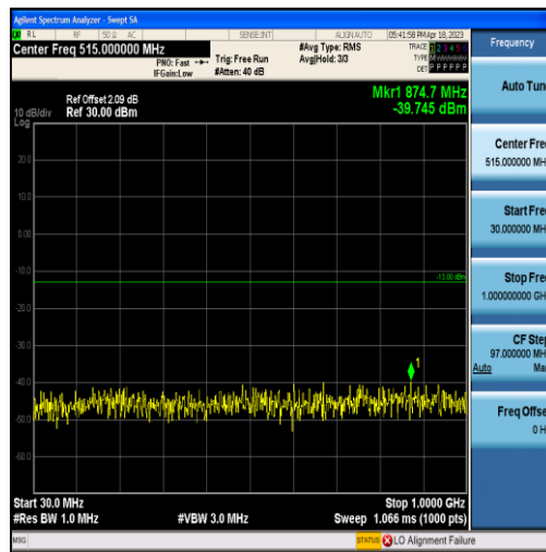
Band4-20MHz-16QAM-20050-100RB#0-Range1:30~1000MHz
