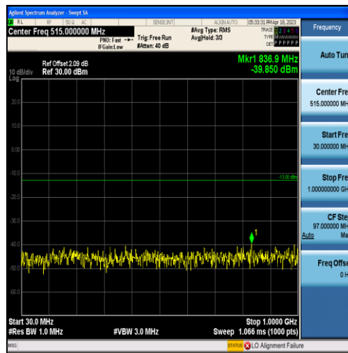
Band4-15MHz-QPSK-20325-75RB#0-Range1:30~1000MHz
