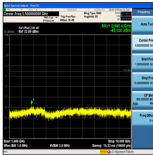
Band5-10MHz-16QAM-20600-50RB#0-Range2:1000~10000MHz
