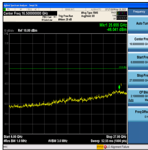
Band7-5MHz-16QAM-21425-25RB#0-Range3:6000~27000MHz
