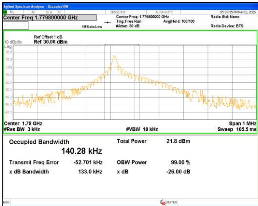
Band66 QPSK Channel=131974 nTones=12@0 Spacing=15kHz
