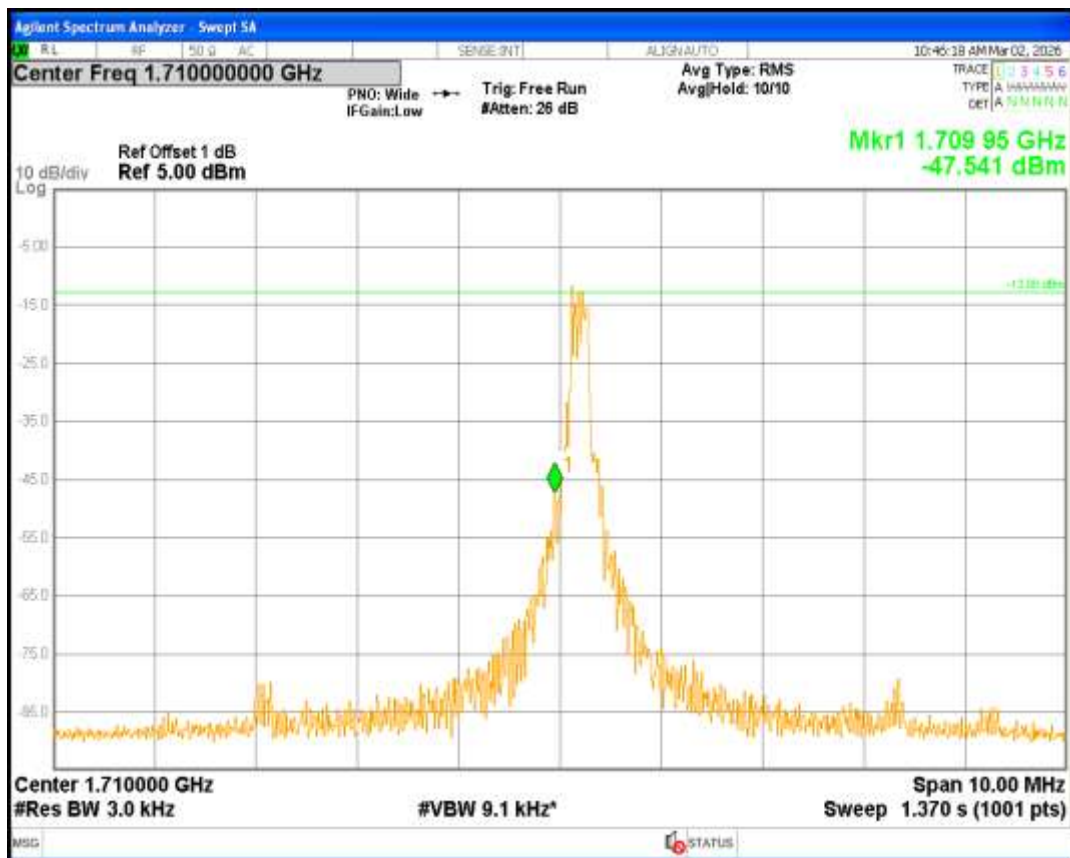
Band4 QPSK Channel=19952 nTones=1@0 Spacing=15kHz
