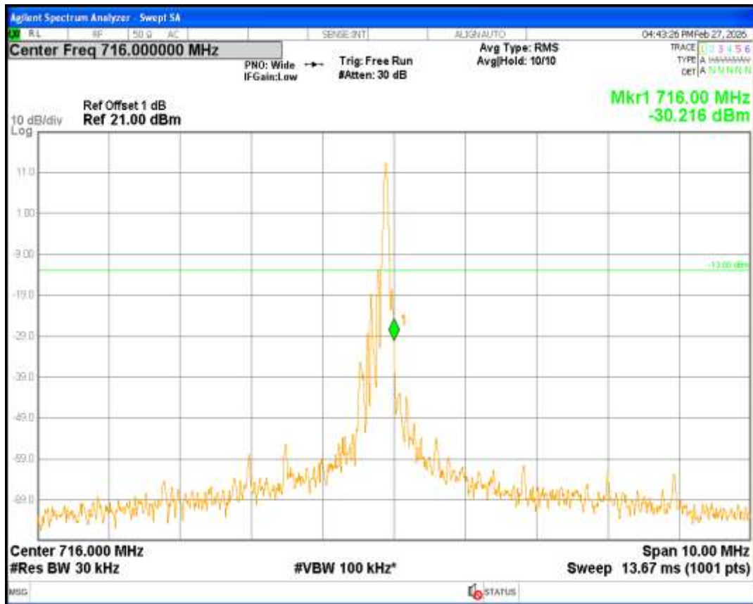
Band17 QPSK Channel=23732 nTones=1@0 Spacing=3.75kHz
