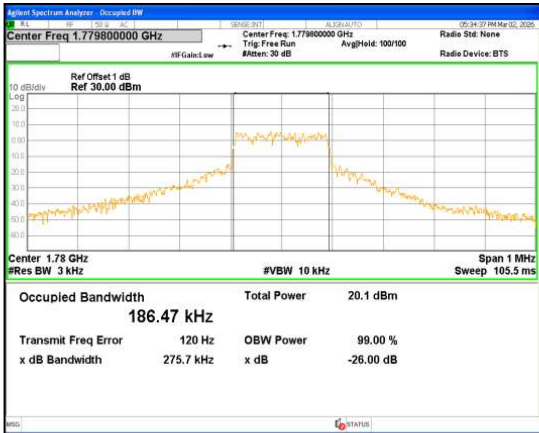
Band66 QPSK Channel=132670 nTones=1@0 Spacing=15kHz
