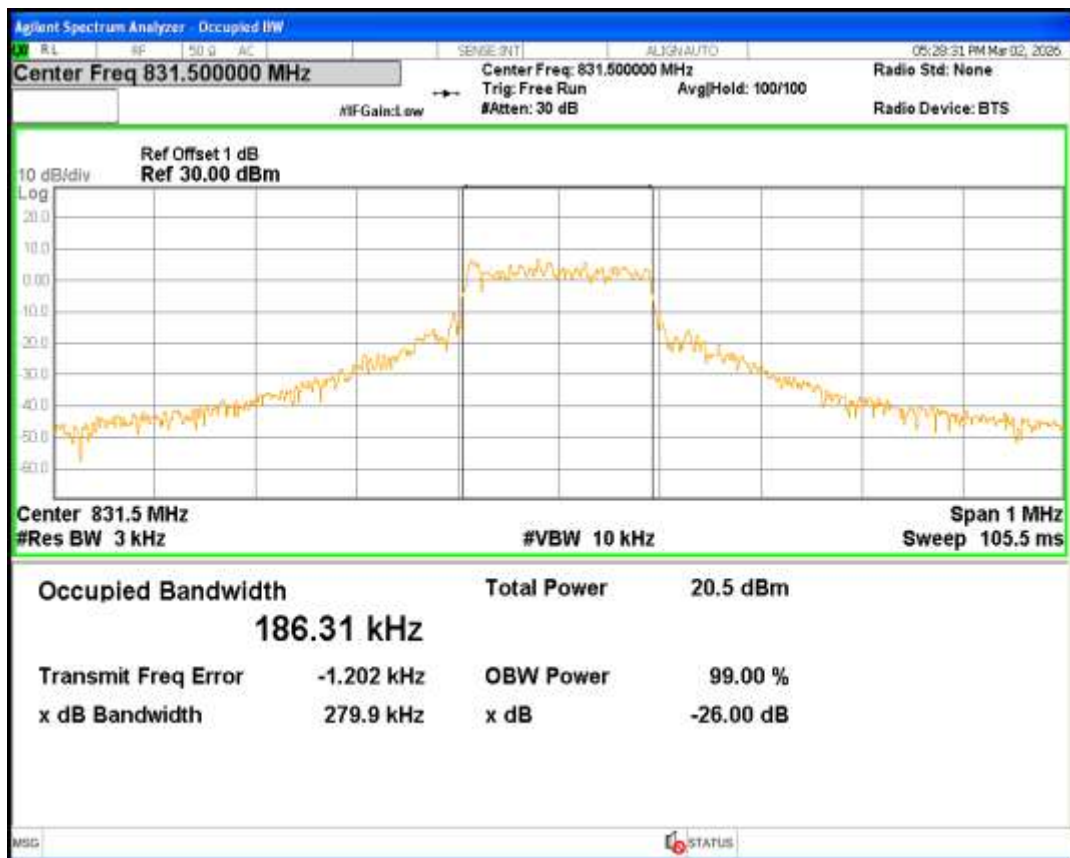
Band26 QPSK Channel=26865 nTones=1@0 Spacing=15kHz
