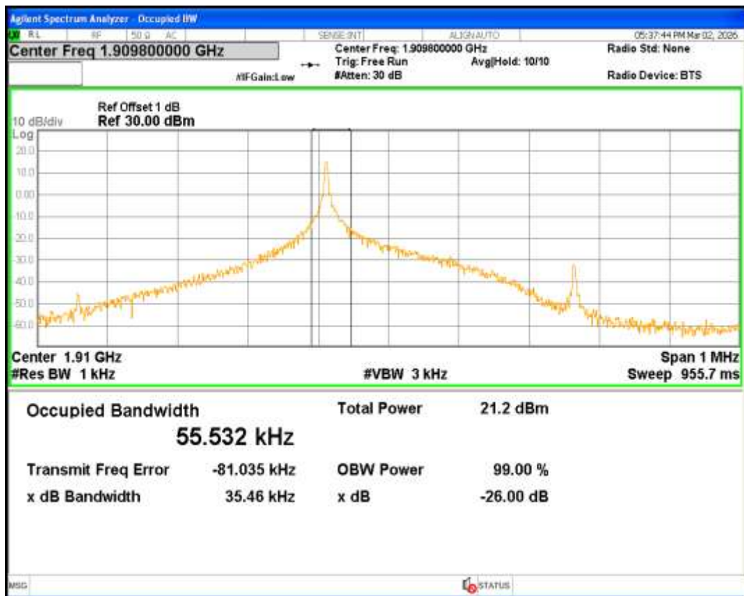
Band2 QPSK Channel=18602 nTones=1@0 Spacing=3.75kHz
