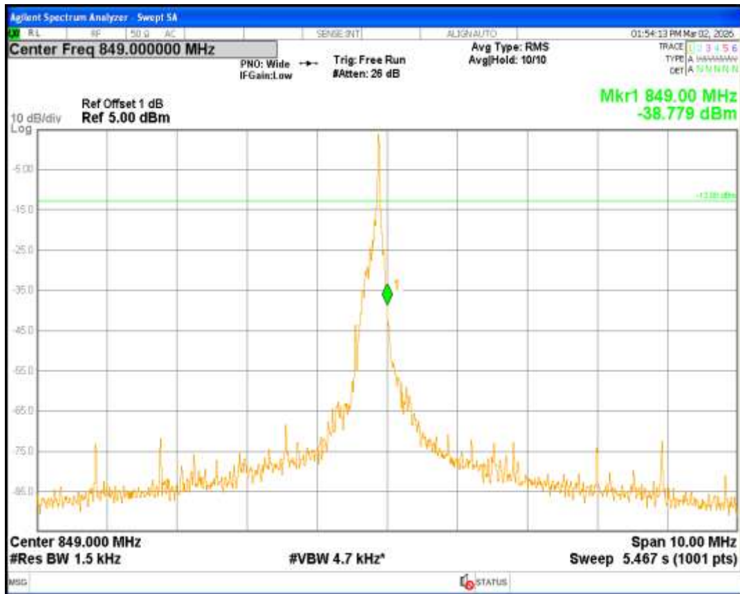
Band5 BPSK Channel=20402 nTones=1@0 Spacing=3.75kHz
