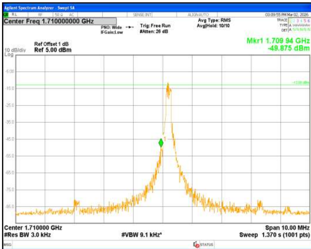
Band66 QPSK Channel=131974 nTones=1@0 Spacing=15kHz
