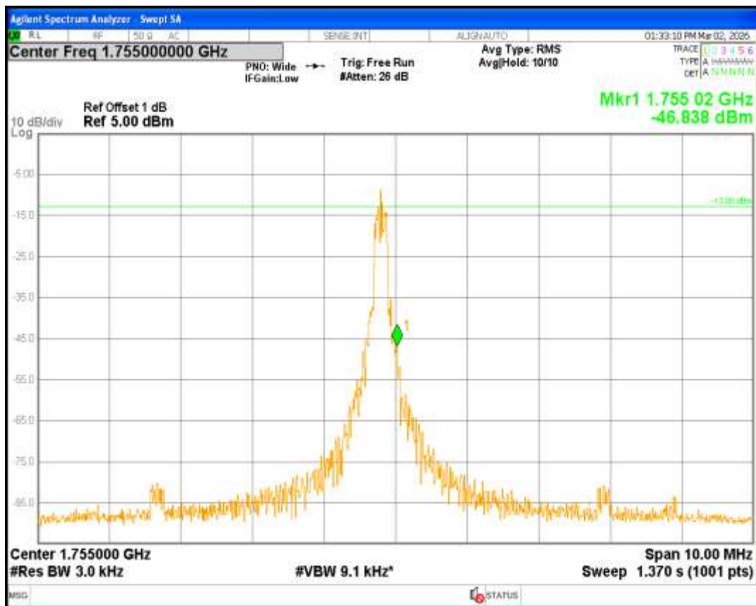
Band4 QPSK Channel=20398 nTones=1@11 Spacing=15kHz
