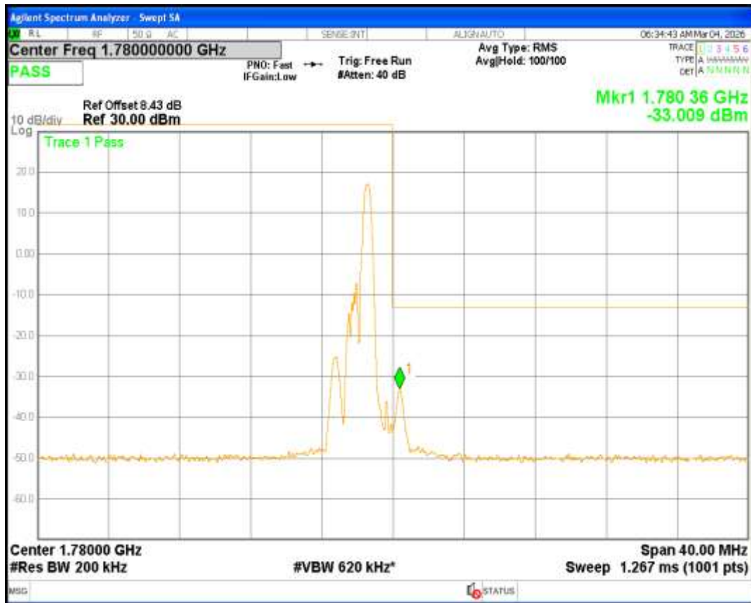
Band66 QPSK BW=20MHz Channel=132572 RB Size=6 Position=#Max NB Index=15
