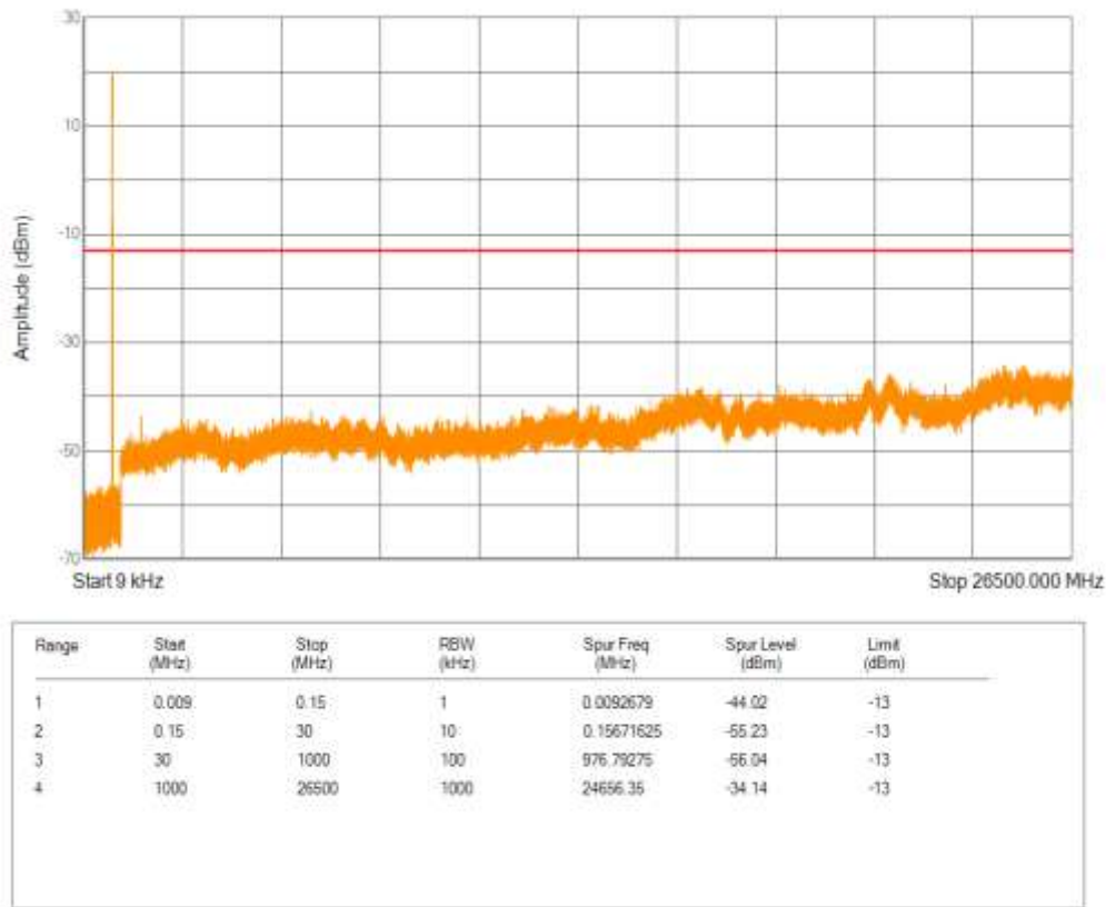
Band13 16QAM BW=5MHz Channel=23230 RB Size=1 Position=#0 NB Index=0
