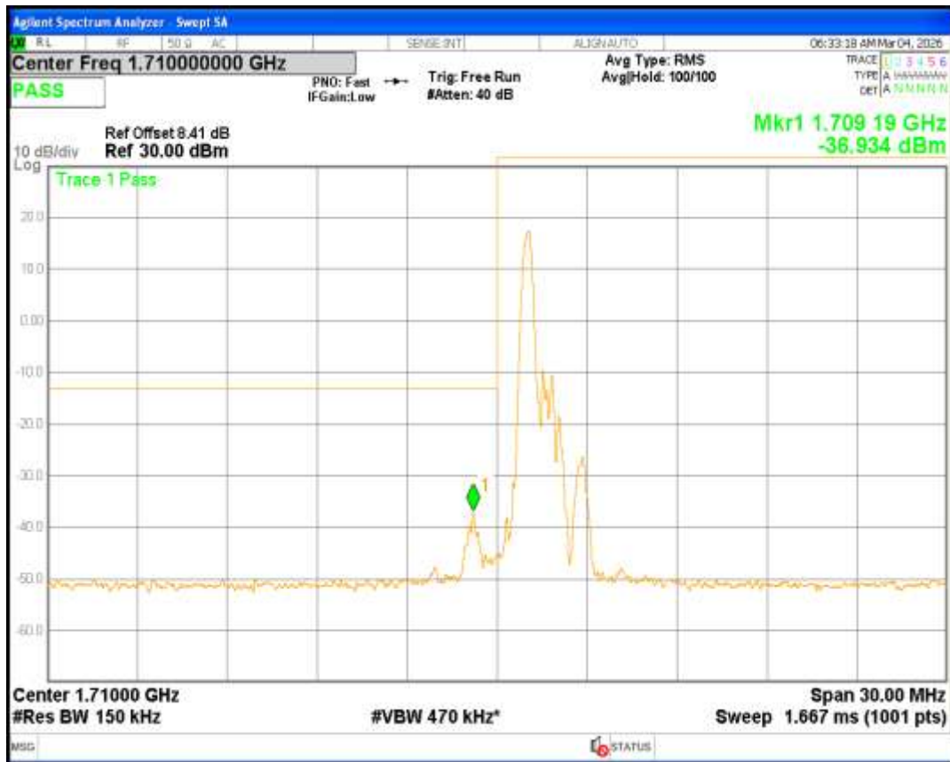
Band66 16QAM BW=15MHz Channel=132597 RB Size=1 Position=#Max NB Index=11
