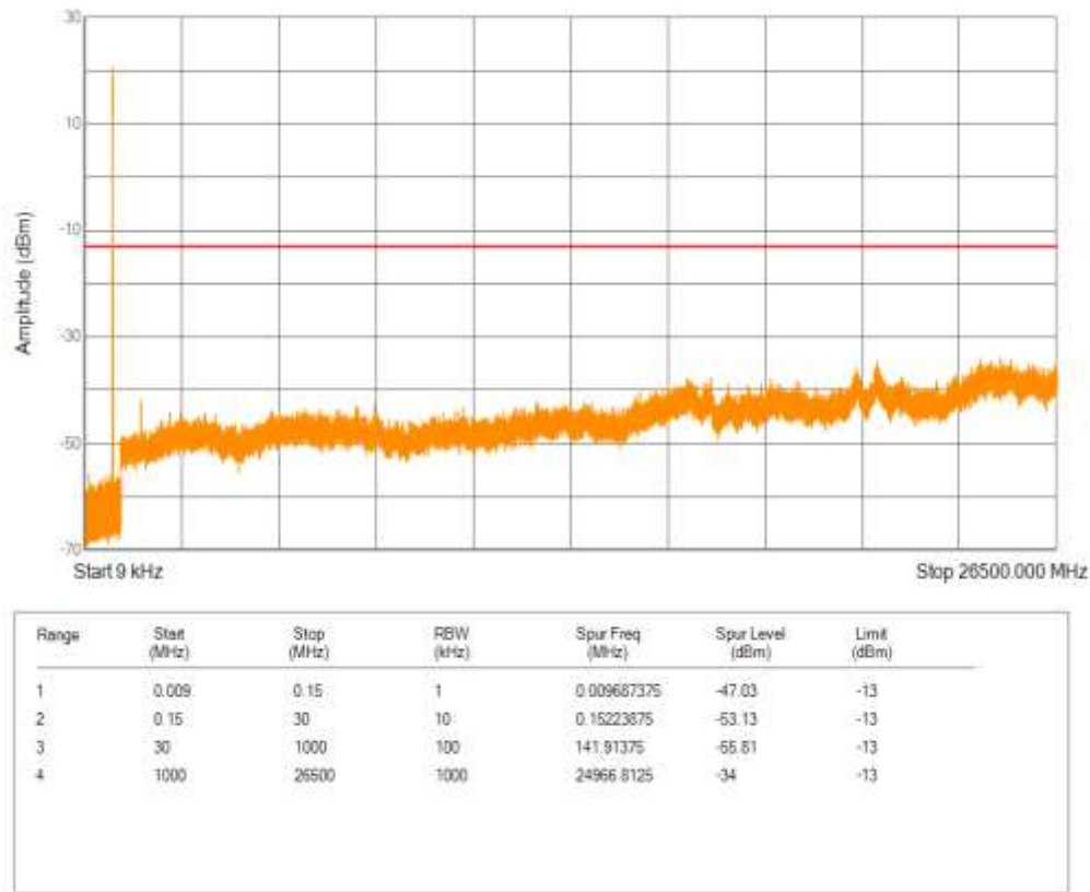
Band13 QPSK BW=5MHz Channel=23230 RB Size=1 Position=#0 NB Index=0
