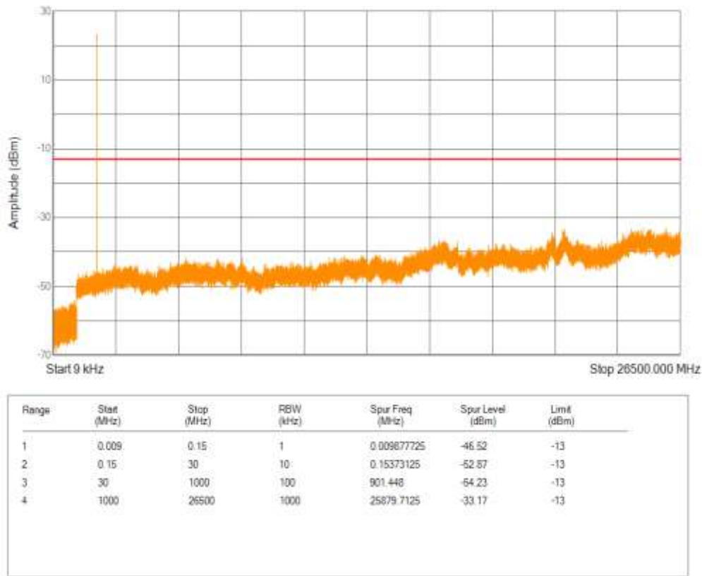
Band2 16QAM BW=1.4MHz Channel=18900 RB Size=1 Position=#0 NB Index=0
