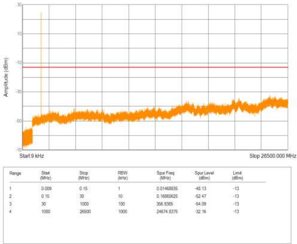
Band2 16QAM BW=1.4MHz Channel=18900 RB Size=5 Position=#0 NB Index=0
