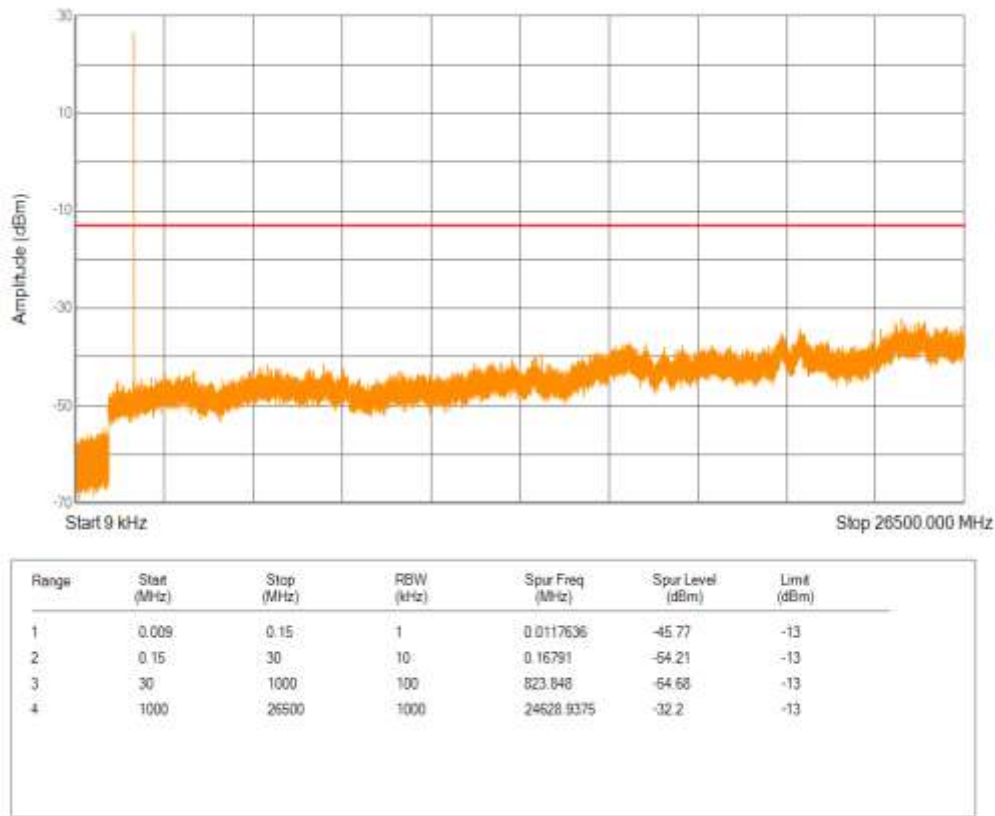
Band66 QPSK BW=3MHz Channel=131987 RB Size=1 Position=#0 NB Index=0
