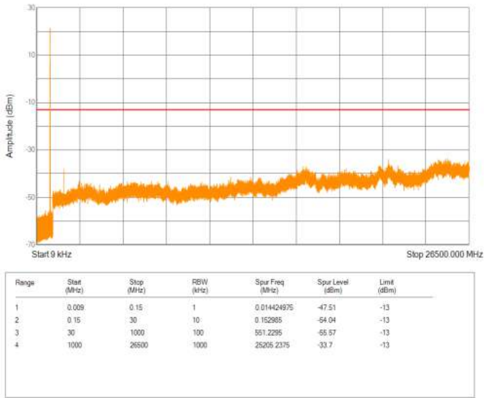
Band5 16QAM BW=10MHz Channel=20600 RB Size=1 Position=#0 NB Index=0
