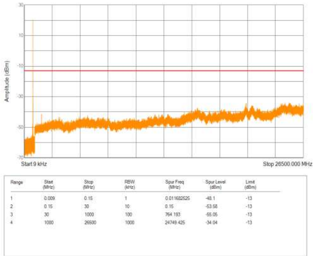
Band5 16QAM BW=5MHz Channel=20525 RB Size=1 Position=#0 NB Index=0
