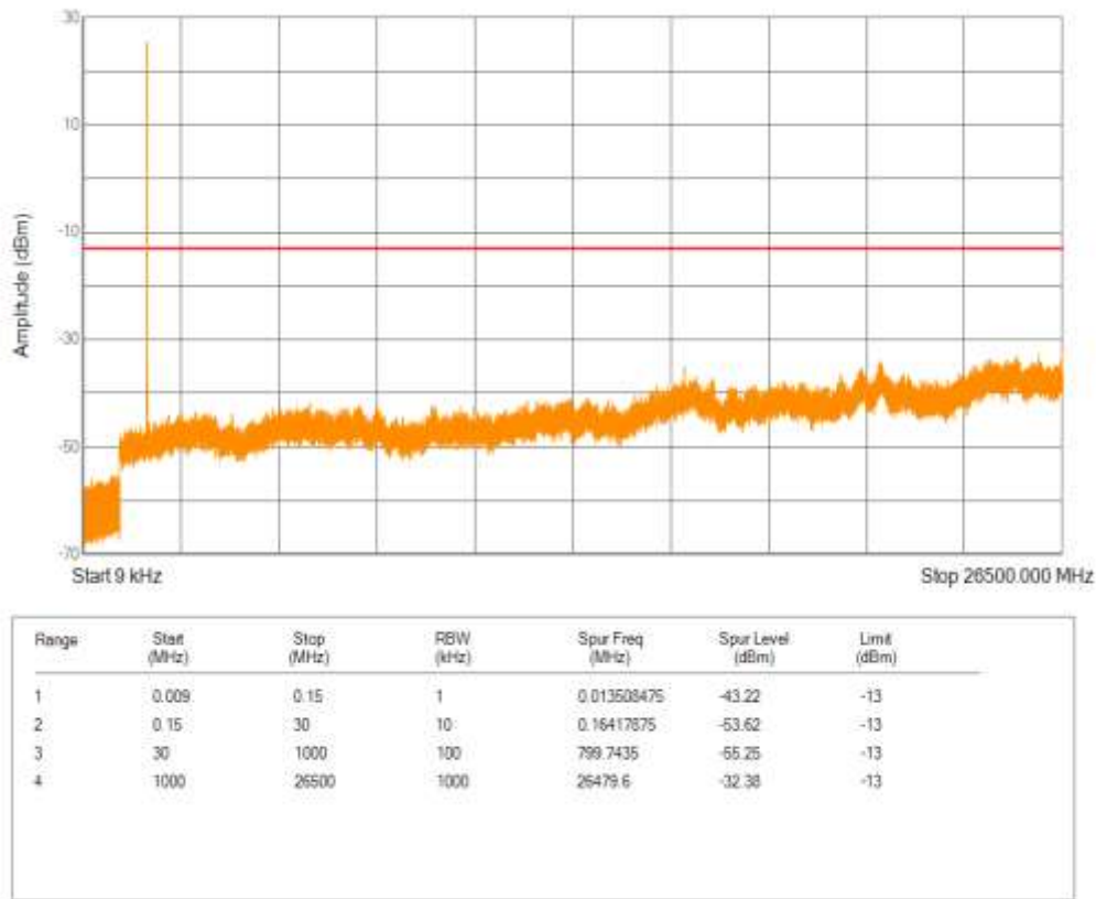
Band66 16QAM BW=1.4MHz Channel=132665 RB Size=1 Position=#0 NB Index=0
