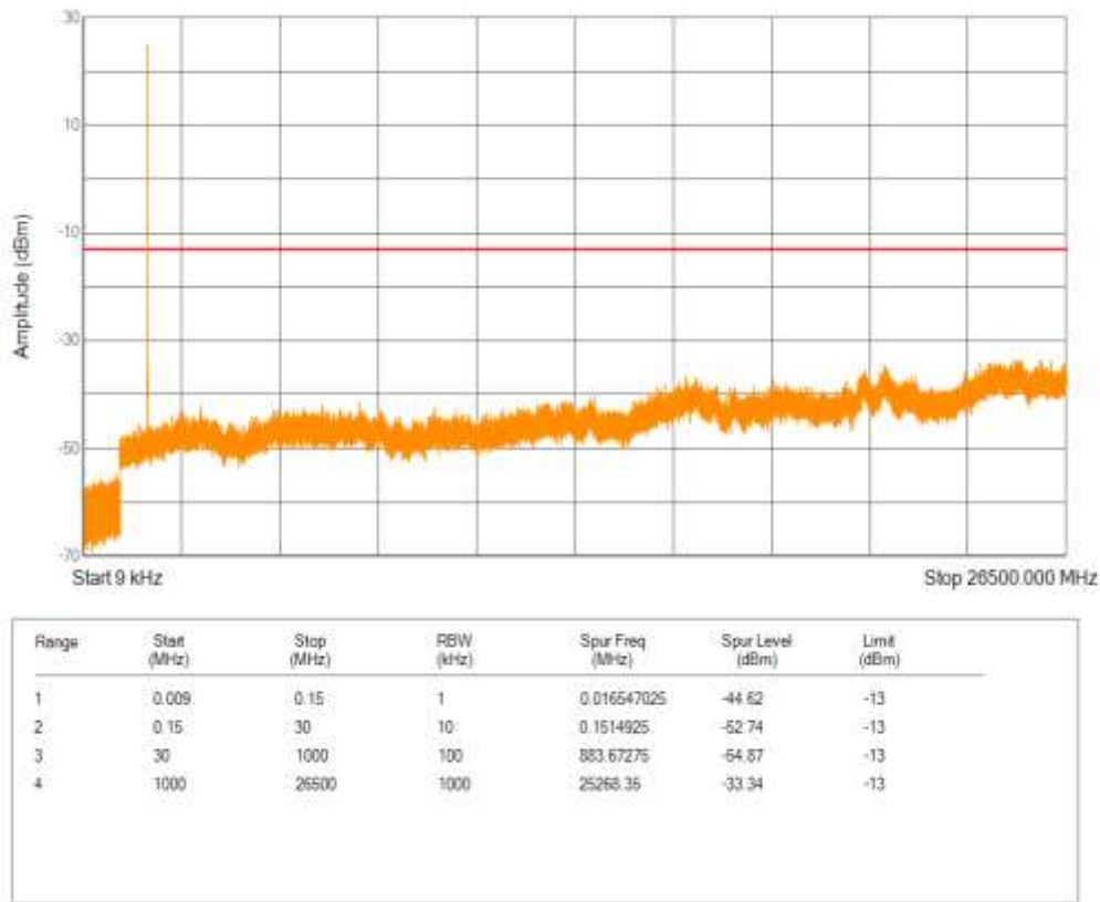
Band5 16QAM BW=1.4MHz Channel=20407 RB Size=1 Position=#0 NB Index=0
