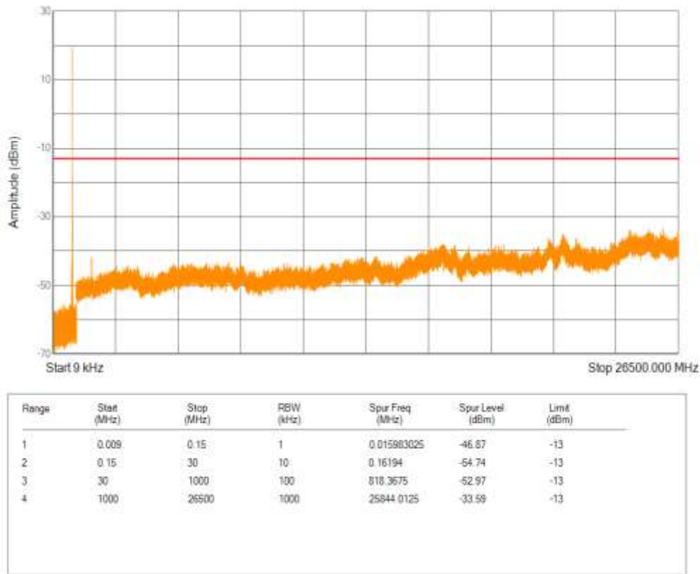
Band5 QPSK BW=1.4MHz Channel=20525 RB Size=1 Position=#0 NB Index=0
