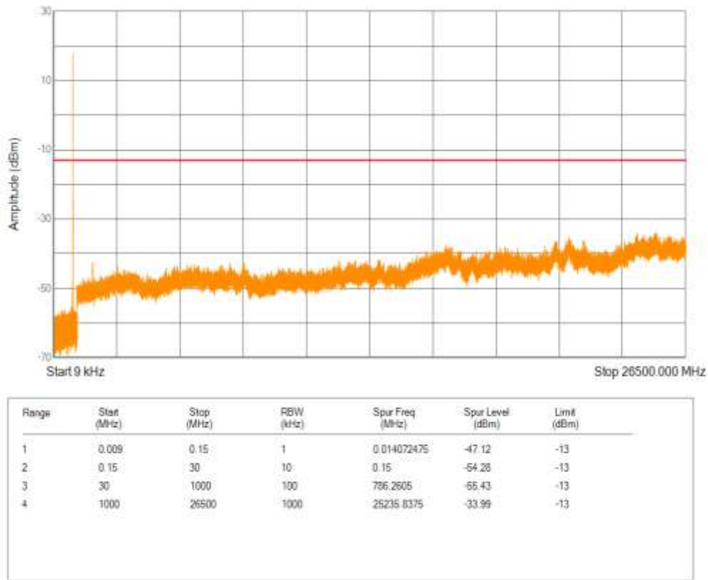
Band5 16QAM BW=1.4MHz Channel=20525 RB Size=1 Position=#0 NB Index=0
