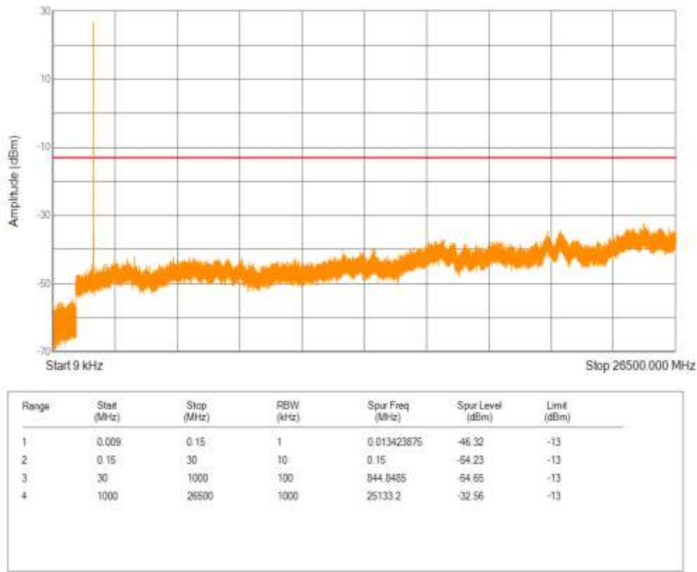
Band66 16QAM BW=1.4MHz Channel=132322 RB Size=5 Position=#0 NB Index=0
