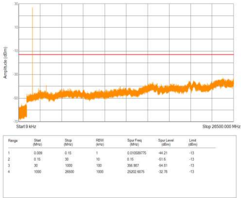
Band66 16QAM BW=20MHz Channel=132572 RB Size=1 Position=#0 NB Index=0
