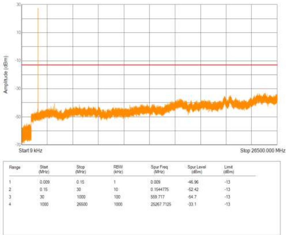
Band66 16QAM BW=10MHz Channel=132322 RB Size=1 Position=#0 NB Index=0
