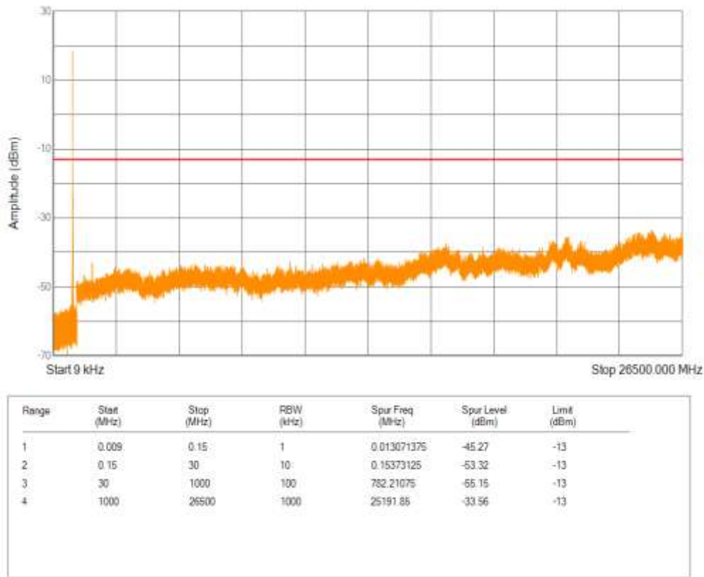
Band5 QPSK BW=3MHz Channel=20525 RB Size=1 Position=#0 NB Index=0
