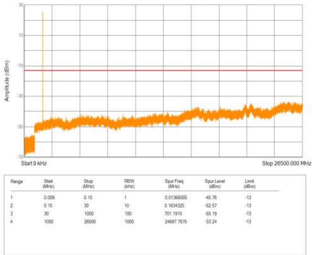
Band66 16QAM BW=5MHz Channel=131997 RB Size=1 Position=#0 NB Index=0
