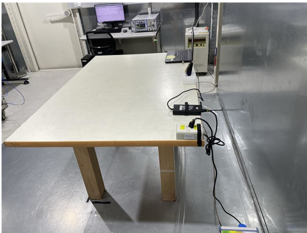
Conducted Test
