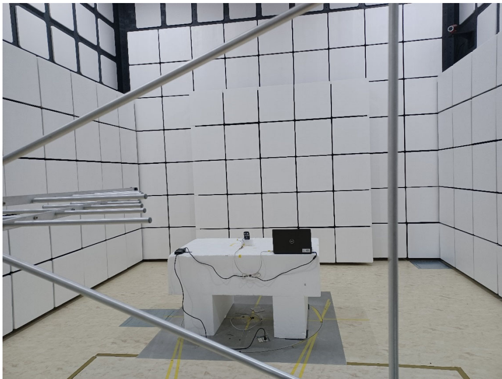
Radiated Test
