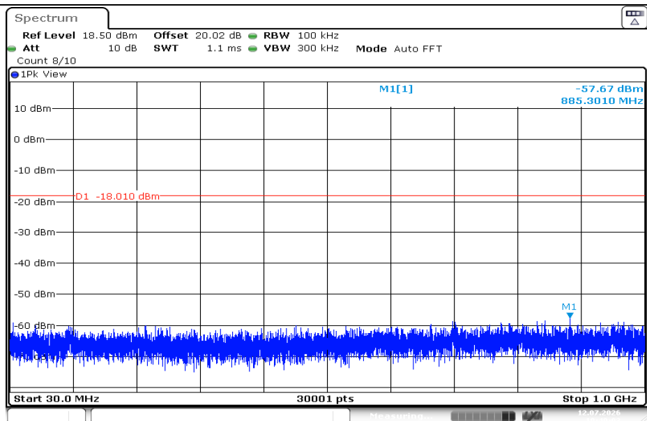
SRD_1Mbps-Ant1-2440-30~1000-PASS
