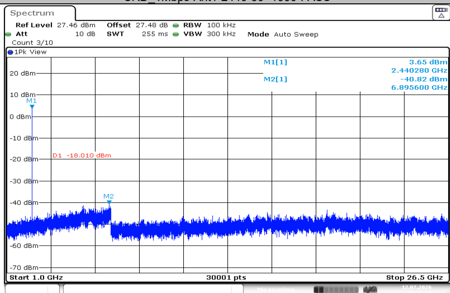
SRD_1Mbps-Ant1-2440-1000~26500-PASS
