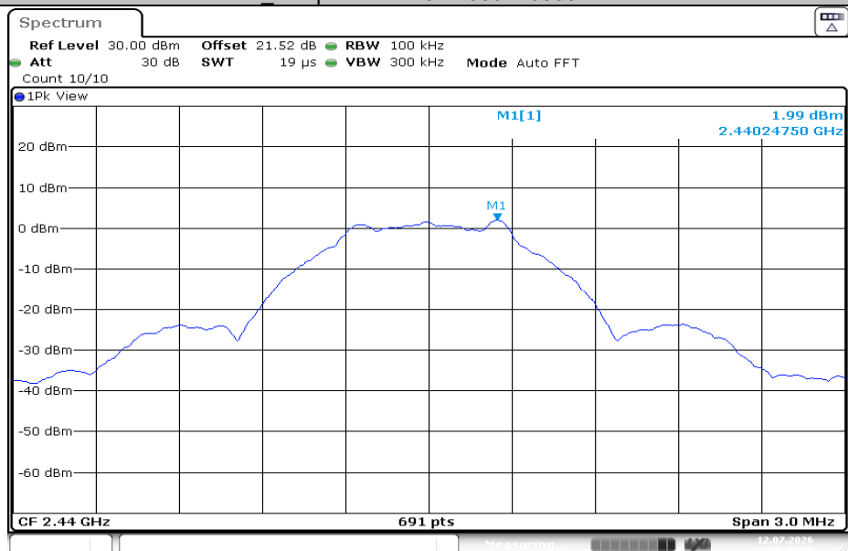
SRD_1Mbps-Ant1-2440-0~Reference-PASS
