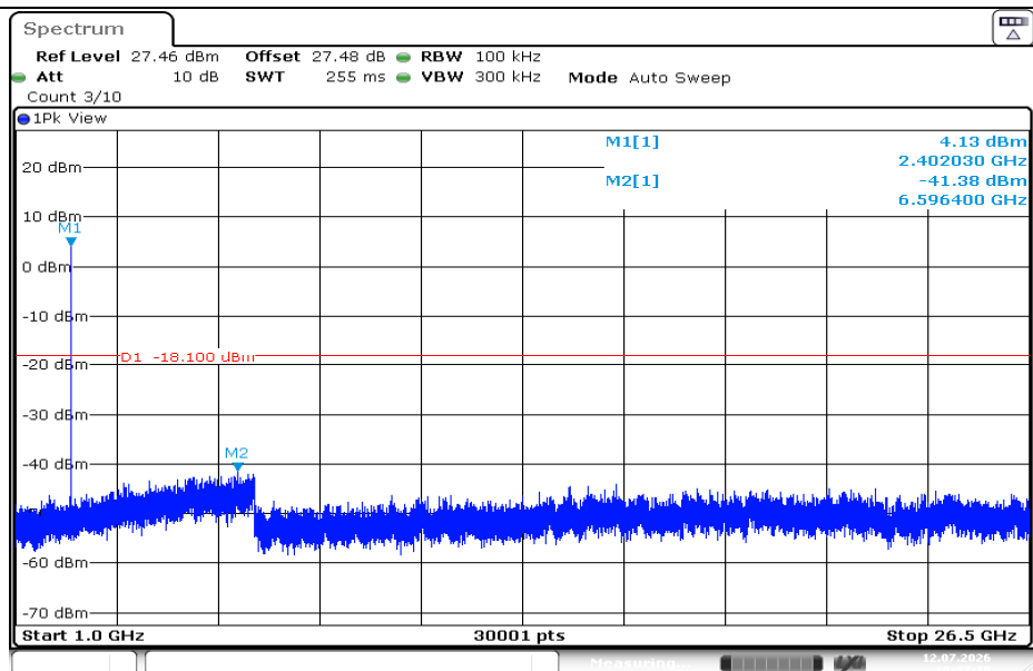
SRD_1Mbps-Ant1-2402-1000~26500-PASS
