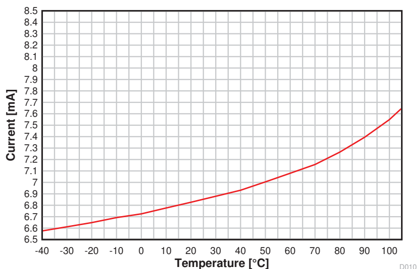
Figure 5-6. RX Current vs. Temperature (BLE 1 Mbps, 2.44 GHz)
