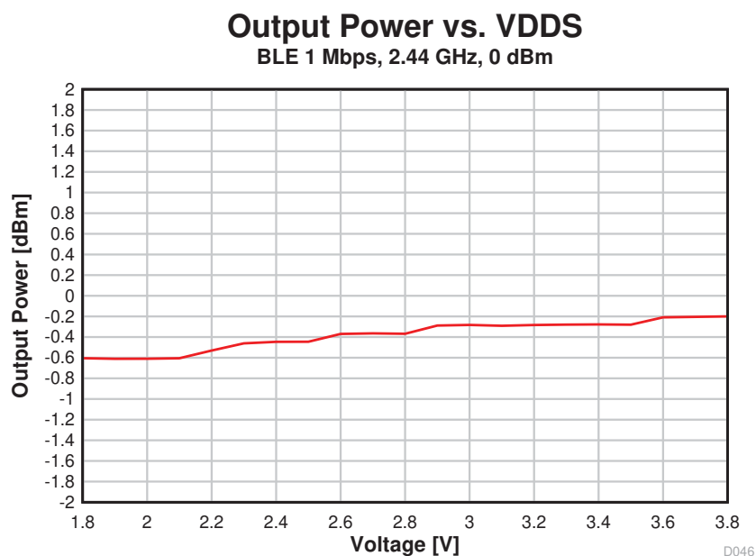
Figure 5-16. Output Power vs. Supply Voltage (VDD5) (BLE 1 Mbps, 2.44 GHz)
