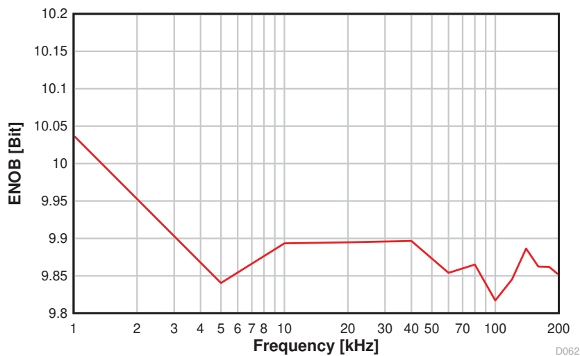
Figure 5-21. ENOB vs. Sampling Frequency
