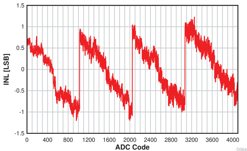
Figure 5-22. INL vs. ADC Code
