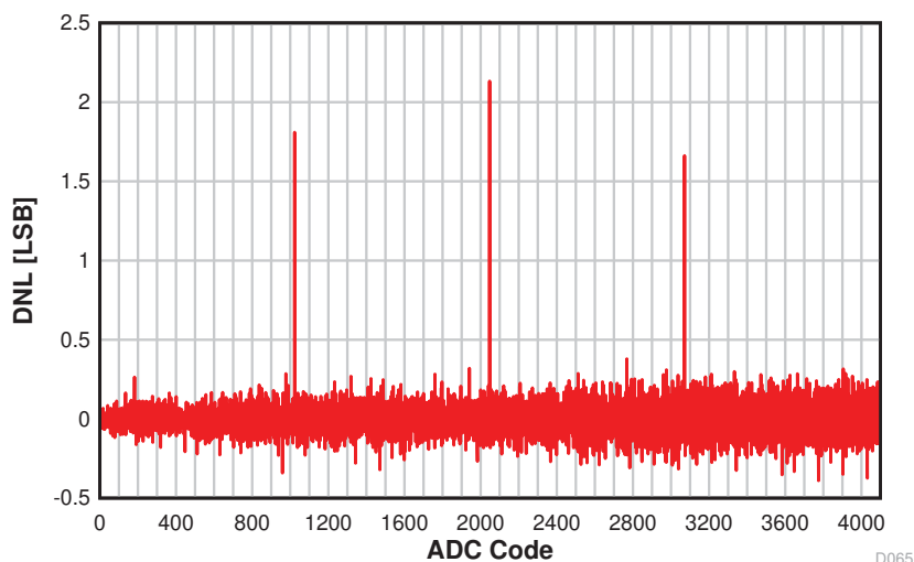
Figure 5-23. DNL vs. ADC Code
