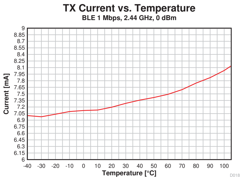
Figure 5-8. TX Current vs. Temperature (BLE 1 Mbps, 2.44 GHz)
