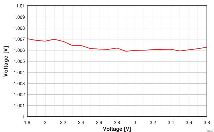
Figure 5-25. ADC Accuracy vs. Supply Voltage (VDD5)
