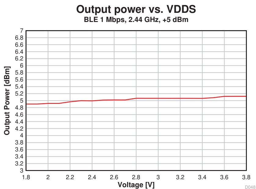
Figure 5-17. Output Power vs. Supply Voltage (VDD5) (BLE 1 Mbps, 2.44 GHz, +5 dBm)
