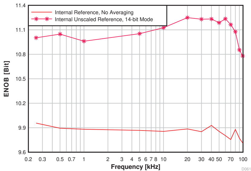
Figure 5-20. ENOB vs. Input Frequency
