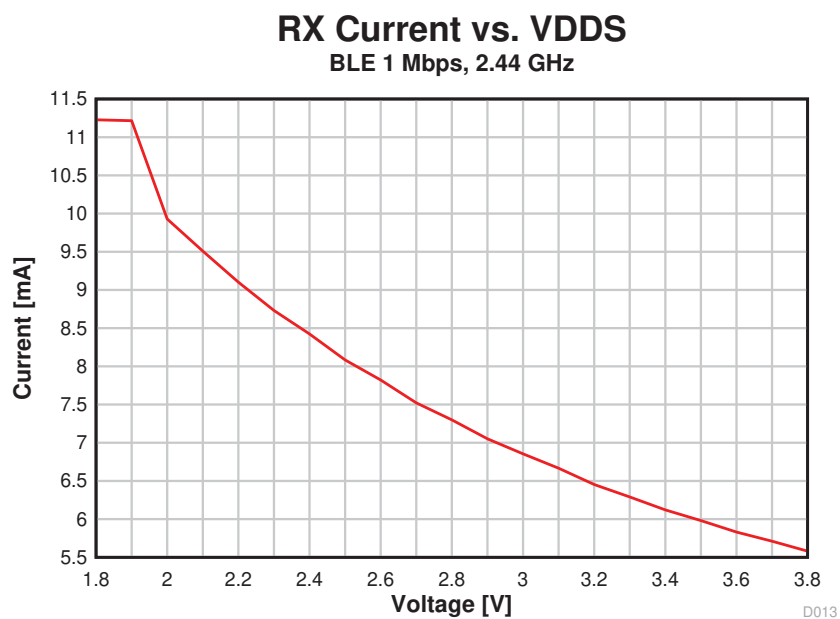
Figure 5-7. RX Current vs. Supply Voltage (VDD5) (BLE 1 Mbps, 2.44 GHz)
