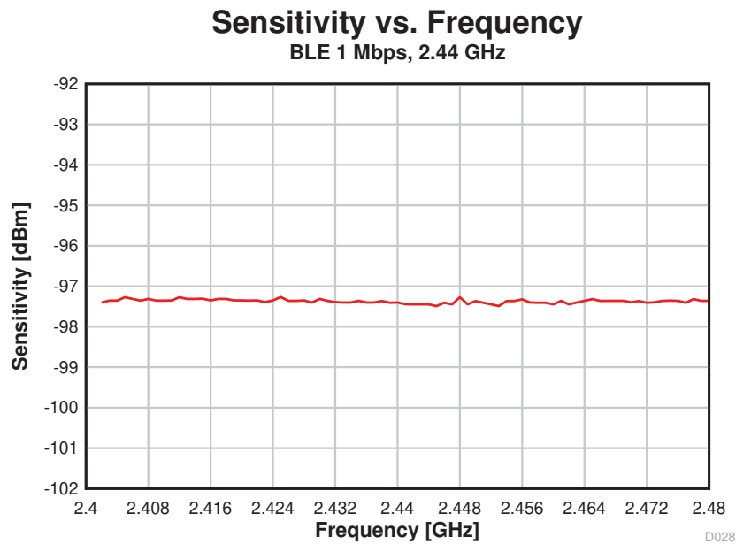
Figure 5-10. Sensitivity vs. Frequency (BLE 1 Mbps, 2.44 GHz)
