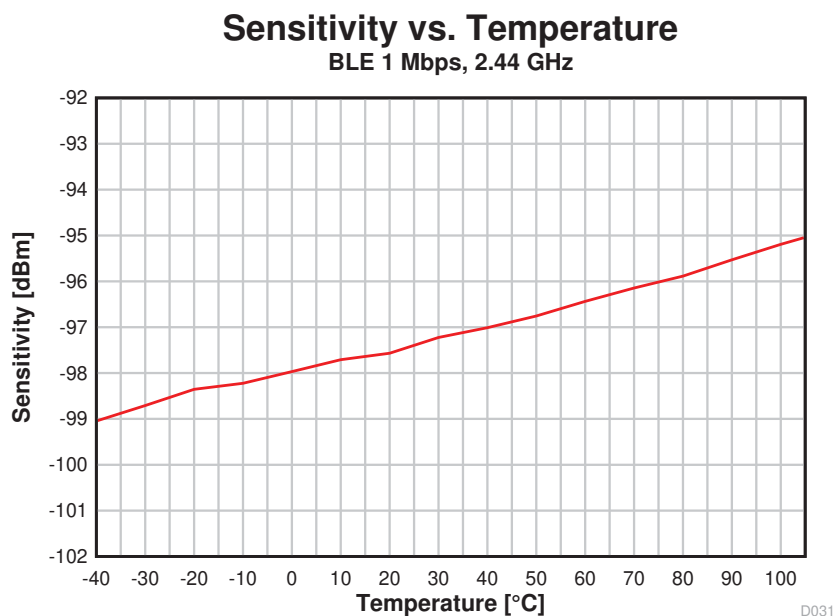
Figure 5-11. Sensitivity vs. Temperature (BLE 1 Mbps, 2.44 GHz)
