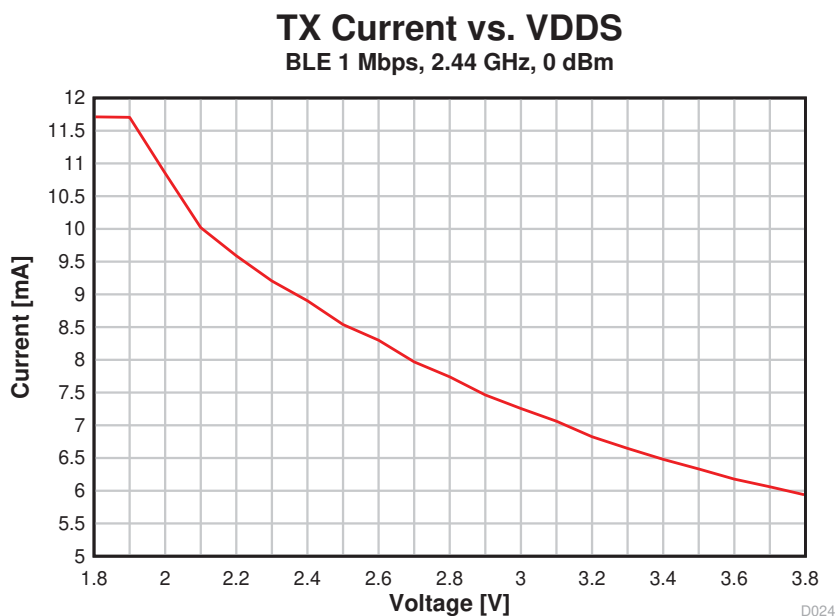
Figure 5-9. TX Current vs. Supply Voltage (VDD5) (BLE 1 Mbps, 2.44 GHz)
