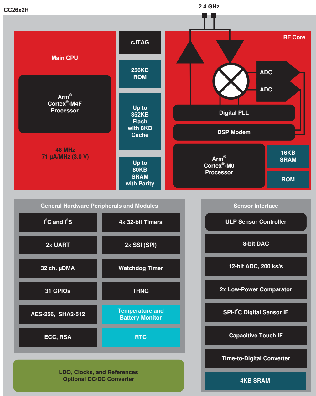
Figure 1-1. CC2642R Block Diagram
