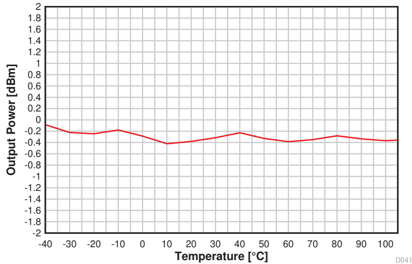
Figure 5-14. Output Power vs. Temperature (BLE 1 Mbps, 2.44 GHz)
