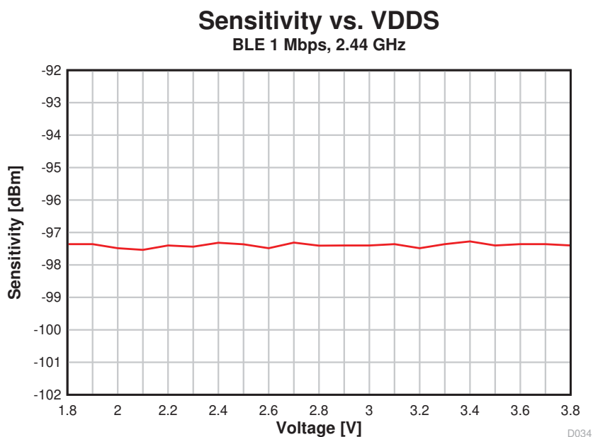
Figure 5-12. Sensitivity vs. Supply Voltage (VDDS) (BLE 1 Mbps, 2.44 GHz)
