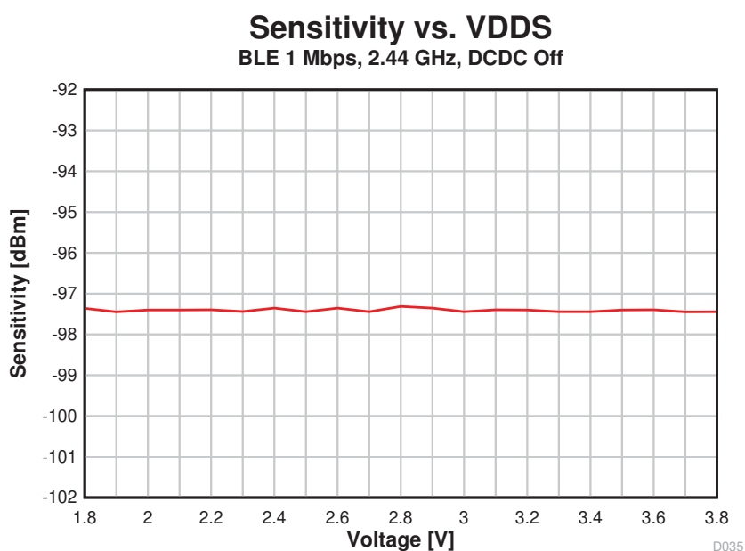
Figure 5-13. Sensitivity vs. Supply Voltage (VDDS) (BLE 1 Mbps, 2.44 GHz, DCDC Off)
