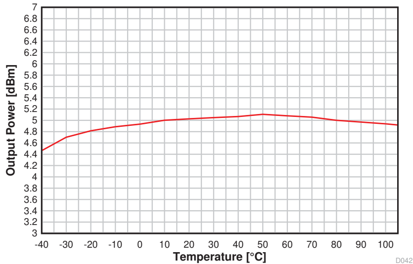
Figure 5-15. Output Power vs. Temperature (BLE 1 Mbps, 2.44 GHz, +5 dBm)
