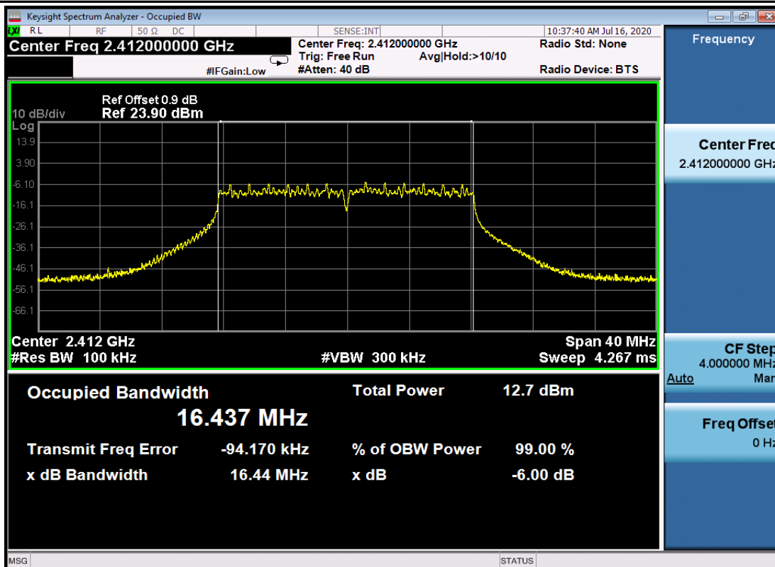
6dB Bandwidth 11G 2412 Ant1
