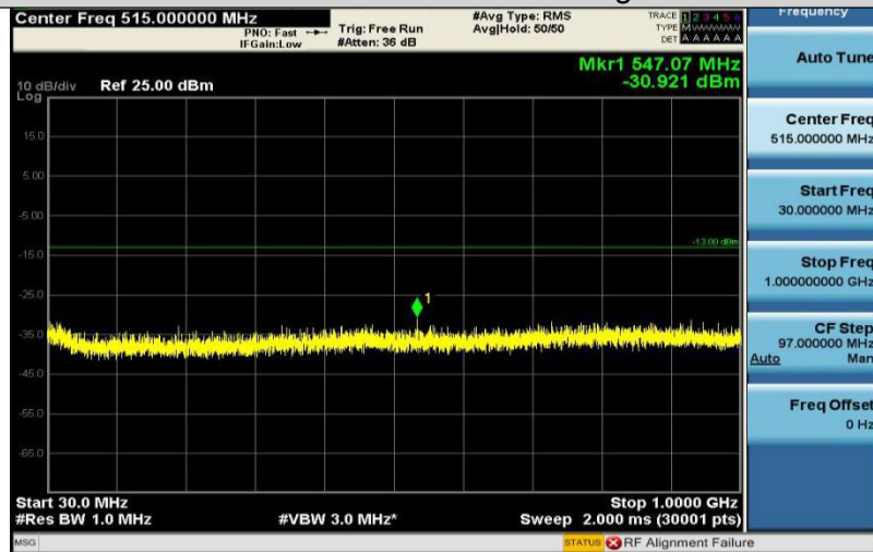
Band4-5MHz-16QAM-20175-1RB#0-Range1:30~1000MHz
