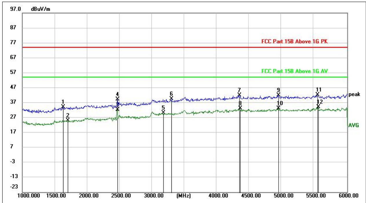
(Plot D: ANT- Vertical, 1GHz - 6GHz)
