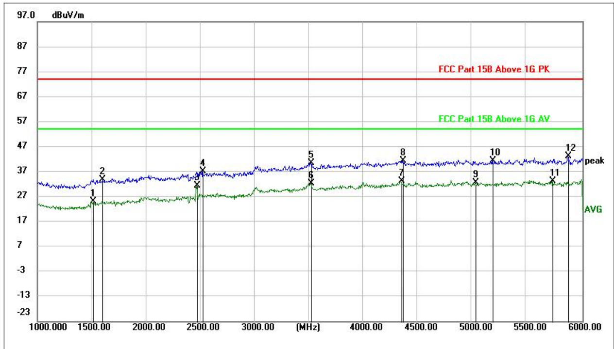
(Plot B: ANT- Horizontal, 1GHz - 6GHz)
