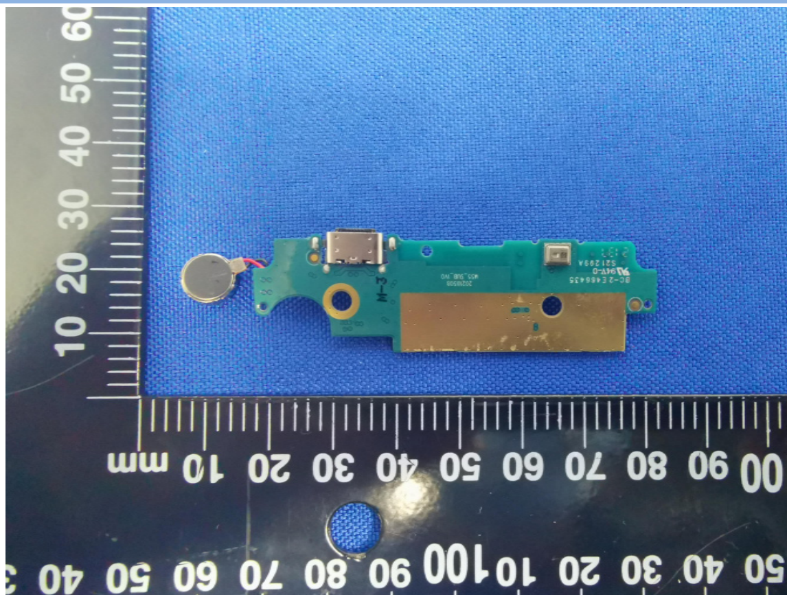
SUB BOARD BACK SIDE VIEW (WITHOUT SHIELDING)
