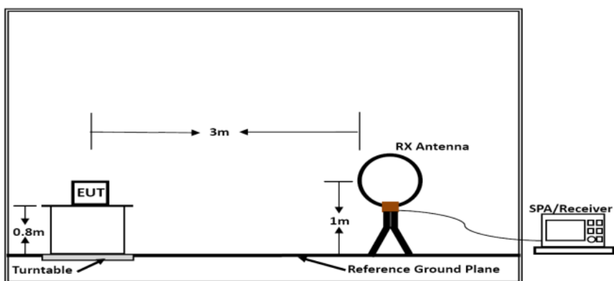
Below 30MHz
