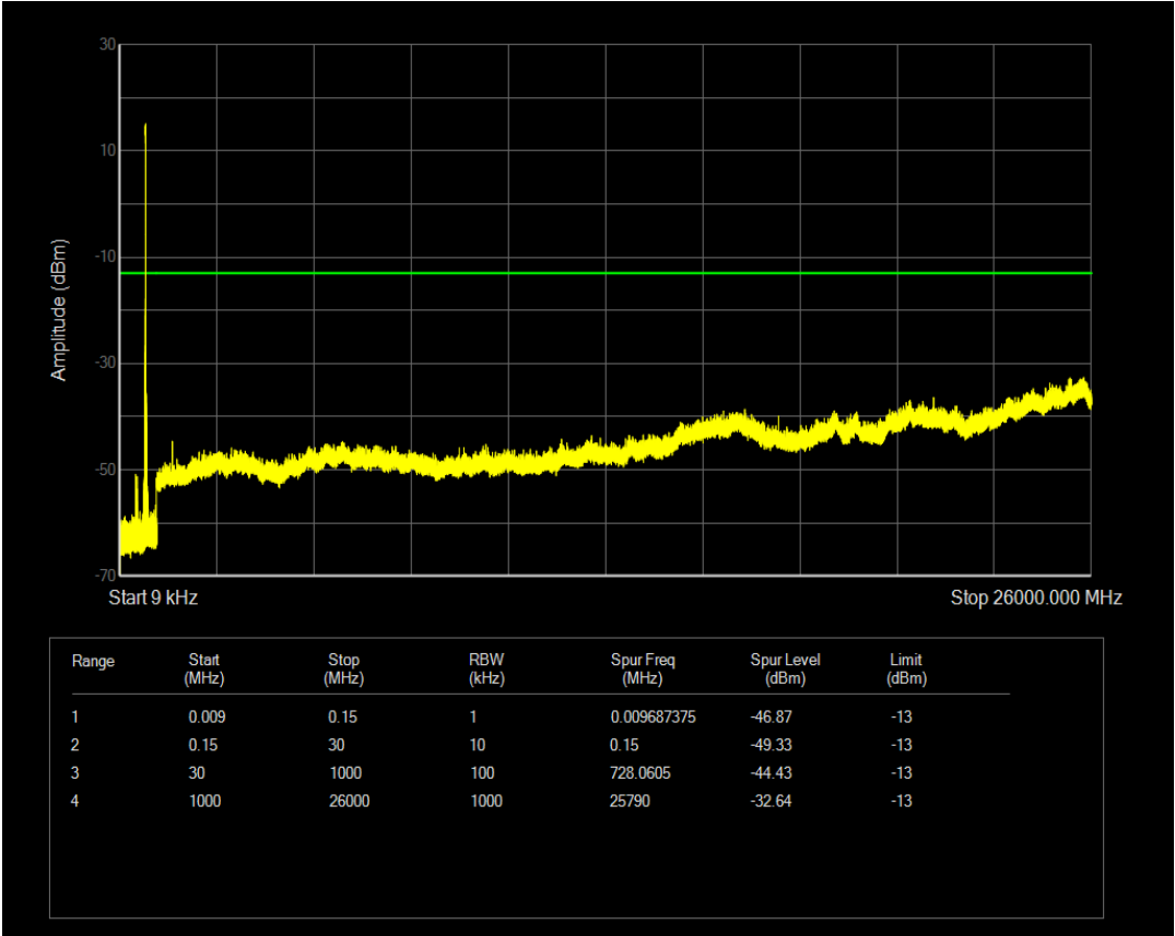
Band12 QAM16 BW=3MHz Channel=23165 RB Size=1 Position=#0 NB Index=0
