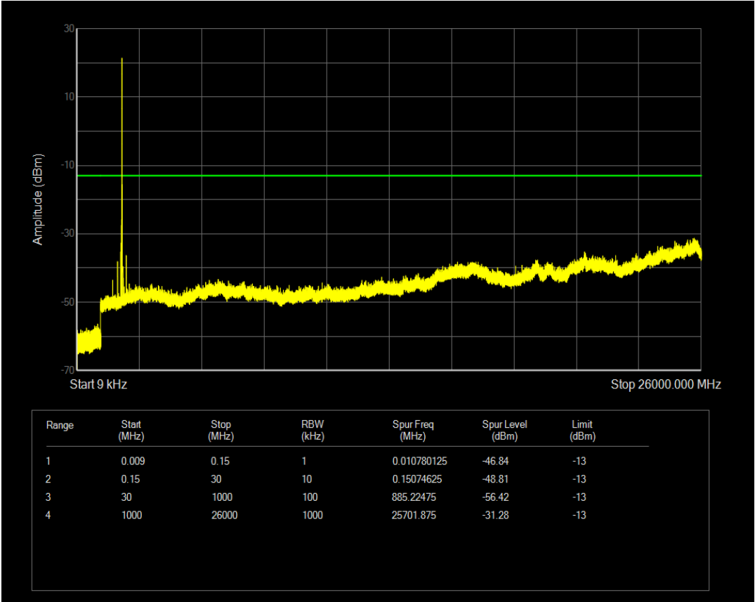
Band2 QAM16 BW=20MHz Channel=19100 RB Size=1 Position=#0 NB Index=0
