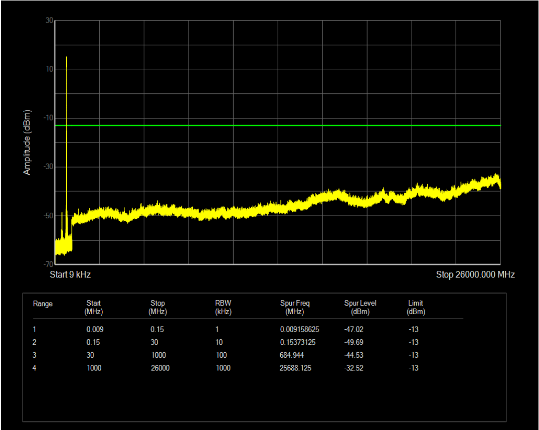
Band12 QPSK BW=3MHz Channel=23165 RB Size=1 Position=#0 NB Index=0
