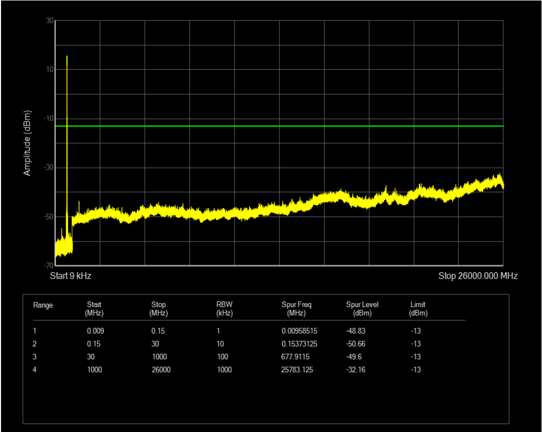
Band12 QPSK BW=5MHz Channel=23155 RB Size=1 Position=#0 NB Index=0
