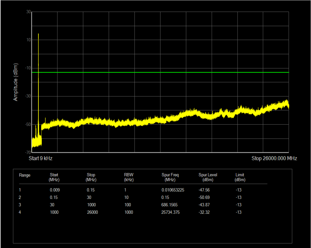
Band12 QAM16 BW=3MHz Channel=23025 RB Size=1 Position=#0 NB Index=0
