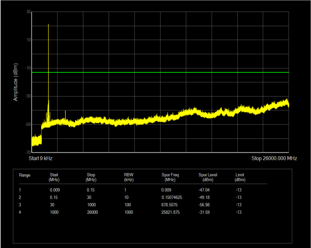
Band4 QAM16 BW=10MHz Channel=20000 RB Size=1 Position=#0 NB Index=0
